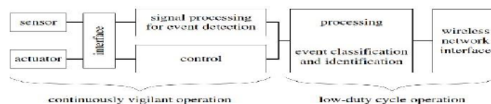
Figure 1 Node Architecture
