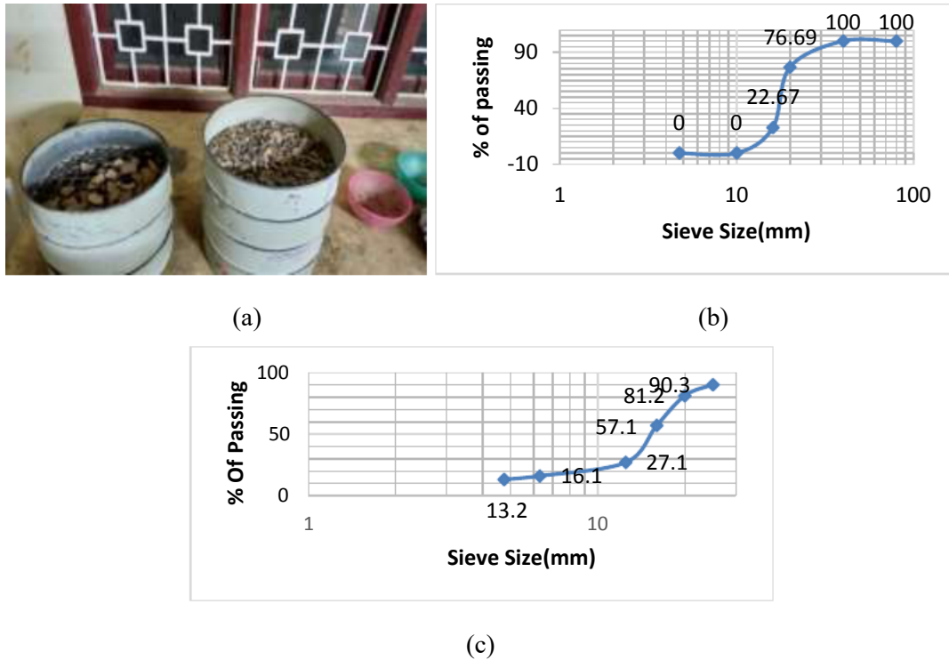
Figure 1 (a) Sieve Analysis of Coarse Aggregate; (b) Fineness modulus for conventional coarse aggregate; (c) Fineness modulus for coconut shell aggregate;
