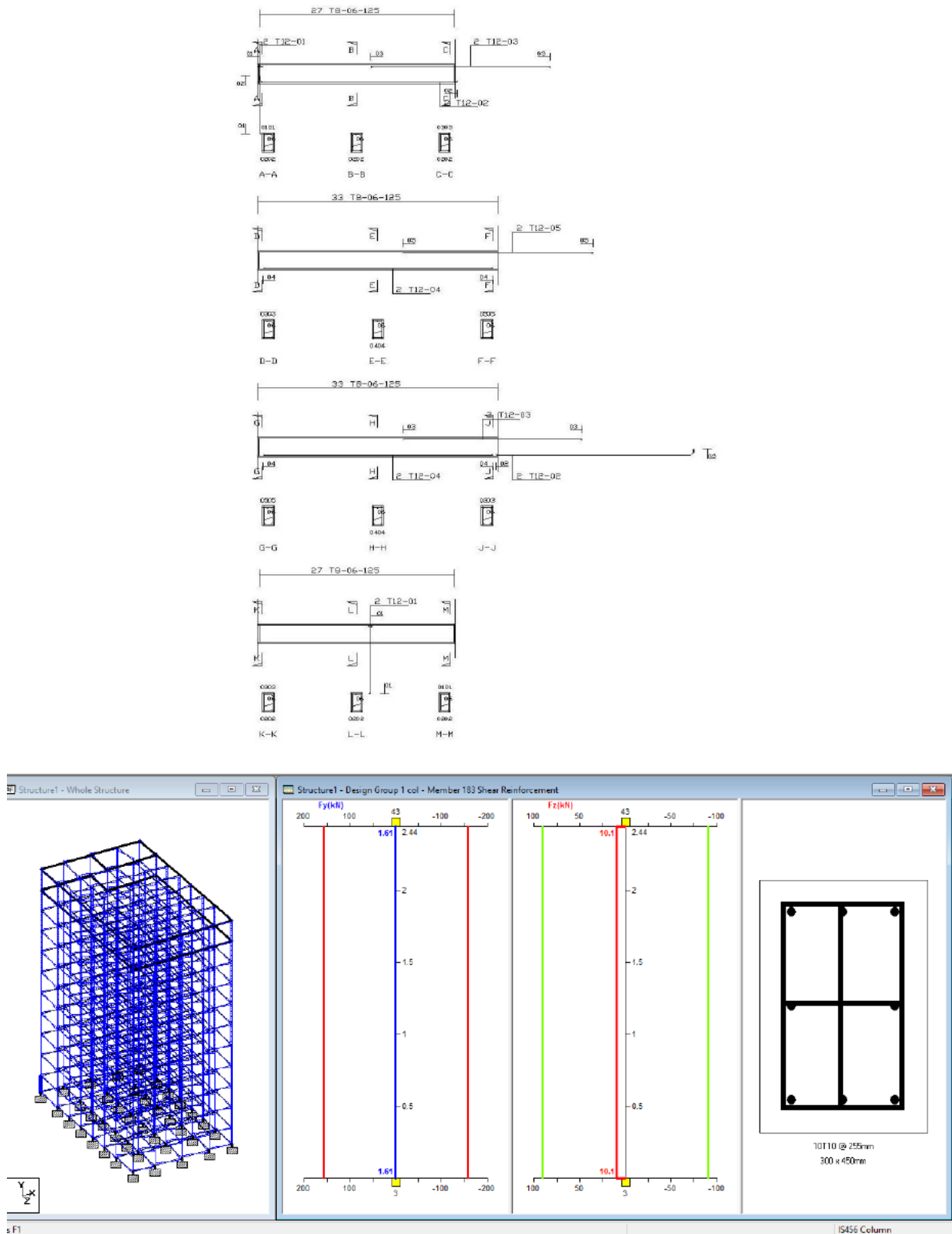
Figure 7 Shear force diagram and column detail for structure
