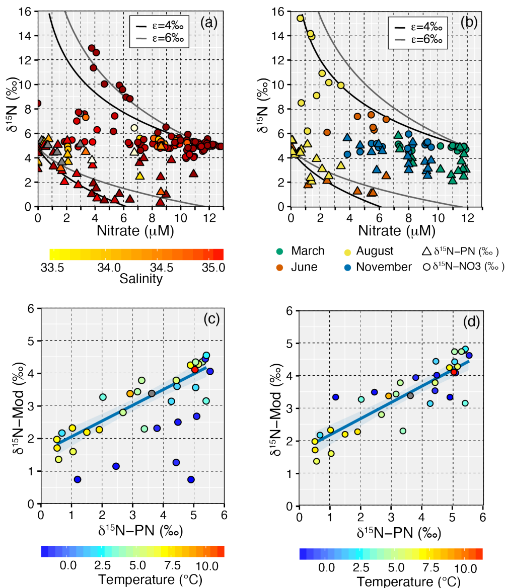
Figure 6. (a) \delta^{15}\text{N-NO}_3 (circles) and \delta^{15}\text{N-PN} (triangles) plotted against nitrate (JR16006), with the colour axis denoting changes in salinity. The lines show the fractionation models for a closed system at \epsilon=4 and 6\text{‰} with an initial nitrate concentration of 11.8\mu\text{M} and \delta^{15}\text{N-NO}_3 of 5.1\text{‰} . (b) \delta^{15}\text{N-NO}_3 (circles) and \delta^{15}\text{N-PN} (triangles) plotted against nitrate from the March, June, August and November Norbjørn transects, with the colour denoting the month of sampling. The lines show the fractionation models for a closed system at \epsilon=4 and 6\text{‰} . (c) Regression between measured and predicted \delta^{15}\text{N-PN} in the upper 40m using a 5\text{‰} fractionation for all samples. (d) Regression between measured and predicted \delta^{15}\text{N-PN} in the upper 40m using a 5\text{‰} fractionation for AW and a 1.8\text{‰} fractionation for ArW.
