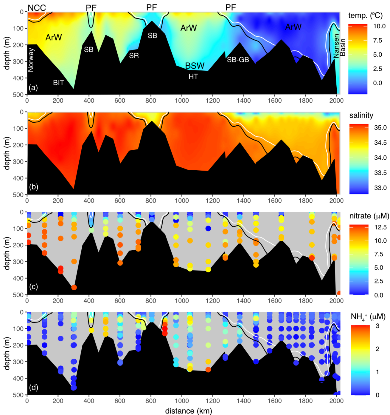
Figure 2. Full 2017 transect of (a) temperature, (b) salinity, (c) nitrate, and (d) \text{NH}_4^+ . Transect is displayed in Figure 1. Solid black and white lines are the 34.8 and 34.7 isohalines. Atlantic Water (AW), Arctic Water (ArW), Barents Sea Water (BSW) and the Norwegian Coastal Current (NCC) are indicated in (a). For reference, key bathymetry features are marked in (a): Spitzbergen Bank
