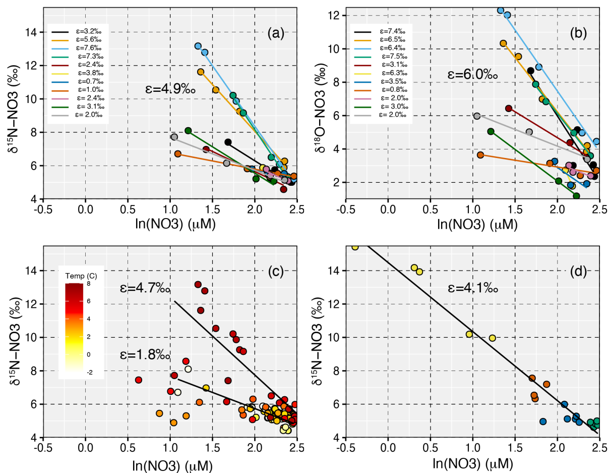
695 Figure 5. (a) \delta^{15}\text{N}-\text{NO}_3 vs \ln\text{NO}_3 , from JR16006 showing the isotope effect ( \epsilon ) for individual stations and an average of 4.9‰. (b) \delta^{18}\text{O}-\text{NO}_3 vs \ln\text{NO}_3 , from JR16006 showing \epsilon for individual stations and an average of 6.0‰. In (a) and (b) only stations with 3+measurements in the upper 120m are used and \epsilon is calculated from stations with less than a 0.2 unit change in salinity. (c) \delta^{15}\text{N}-\text{NO}_3 vs \ln\text{NO}_3 for all samples from JR16006. Atlantic Water \epsilon = 4.7\text{‰} and Arctic Water \epsilon = 1.8\text{‰} . (d) \delta^{15}\text{N}-\text{NO}_3 vs \ln\text{NO}_3 for seasonal Norbjorn samples between 72 and 76°N from the Barents Sea Opening, \epsilon = 4.1\text{‰} .
