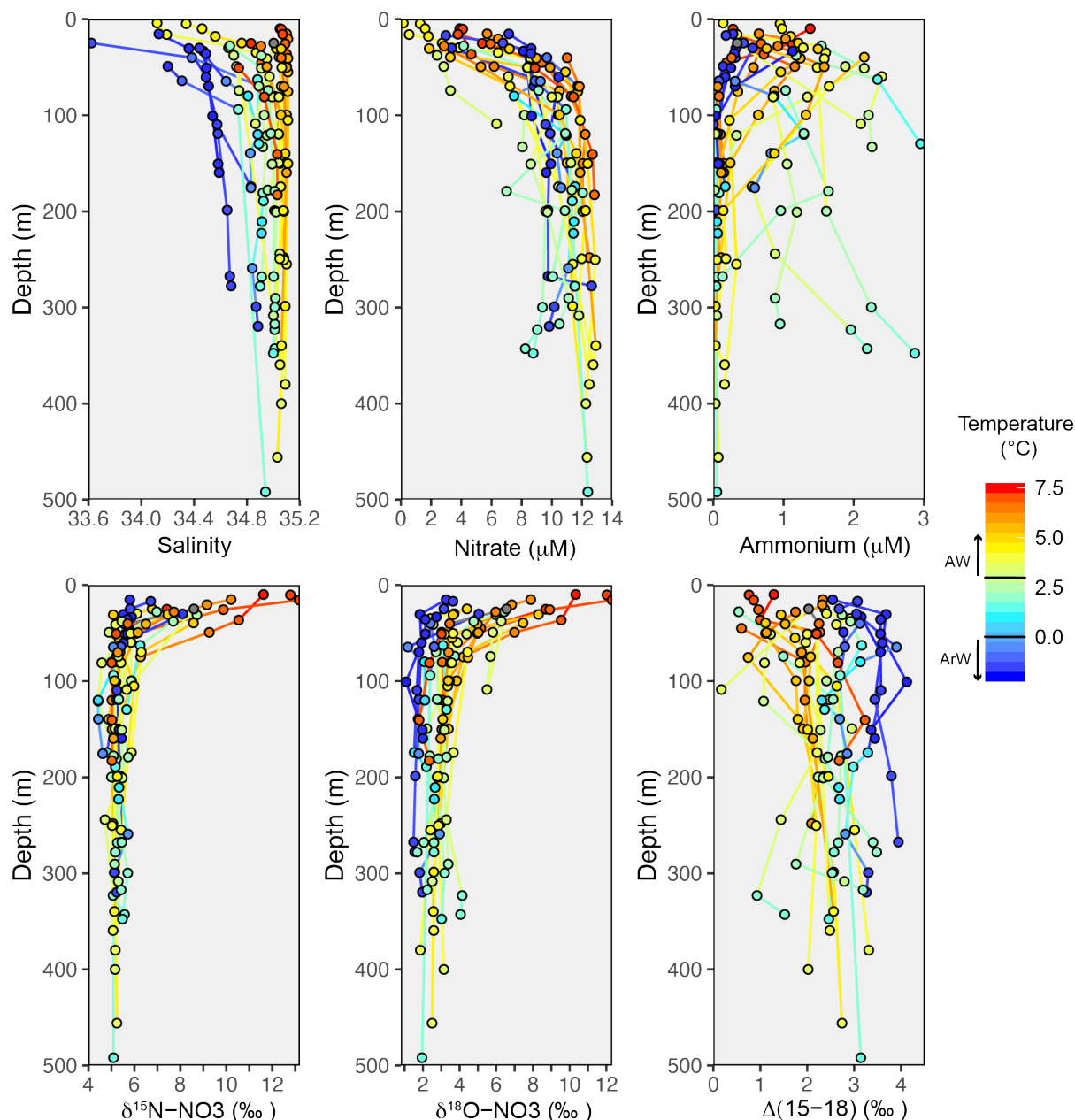
Figure 4. Depth profiles in upper 500 m of the Barents Sea shelf. Colour denotes temperature changes. (a) Salinity, (b) Nitrate ( \mu\text{M} ), (d) \text{NH}_4^+ ( \mu\text{M} ), (d) \delta^{15}\text{N-NO}_3 (‰ vs. AIR), (e) \delta^{18}\text{O-NO}_3 (‰ vs. VSMOW) and (f) \Delta(15-18) (‰). Need to add (a), (b) to subplots.
