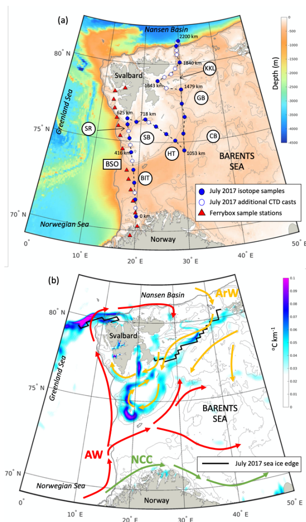
Figure 1. (a) Station locations within the Barents Sea from JR16006 during July 2017 and on repeat FerryBox transects in March, June, August and November 2018. Shading is the depth (in metres). The grey contours mark the 200 m, 300 m and 500 m isobaths. Key bathymetric features are marked: Bear Island Trough (BIT), Hopen Trench (HT), Spitzbergen Bank (SB), Central Bank (CB), Great Bank (GB), Storfjordrenna (SR), Kong Karls Land (KKL) and the Barents Sea Opening (BSO). Distances along the transects presented in Figure 2 and 3 are marked. (b) Schematic of the circulation of Atlantic Water (AW), Arctic Water (ArW) and the Norwegian Coastal Current (NCC). Shading is the July 2017 sea surface temperature gradient ( ^{\circ}\text{C km}^{-1} ) calculated from the OSTIA SST product (Donlon et al., 2012) and shows the sea surface temperature expression of the Polar Front along the edges of Spitzbergen Bank and Grand Bank. The solid black contour marks the July 2017 sea ice edge (data from the National Snow and Ice Data Center). Grey bathymetric contours as in (a).
