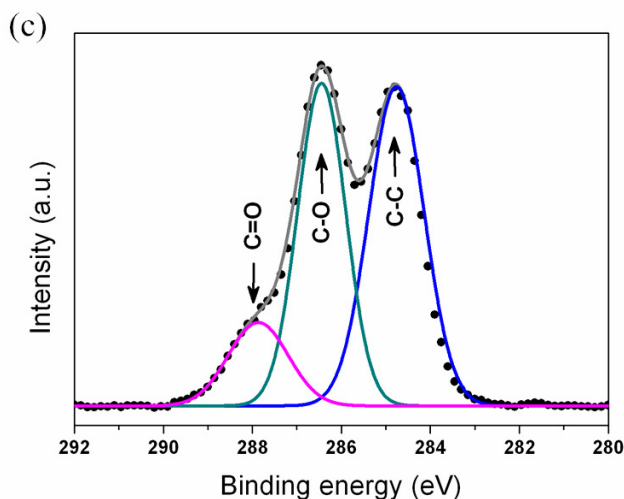
Figure 2: High resolution C 1s spectra, with component fitted carbon region, for (a) untreated hemp, (b) waterbath treated fiber and (c) microwave treated fiber
