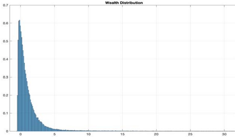
Figure 3: Wealth Distribution Histogram
