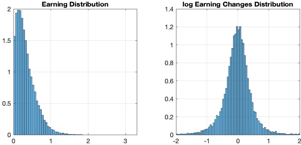
Figure 2: Square-root Earning Distribution
