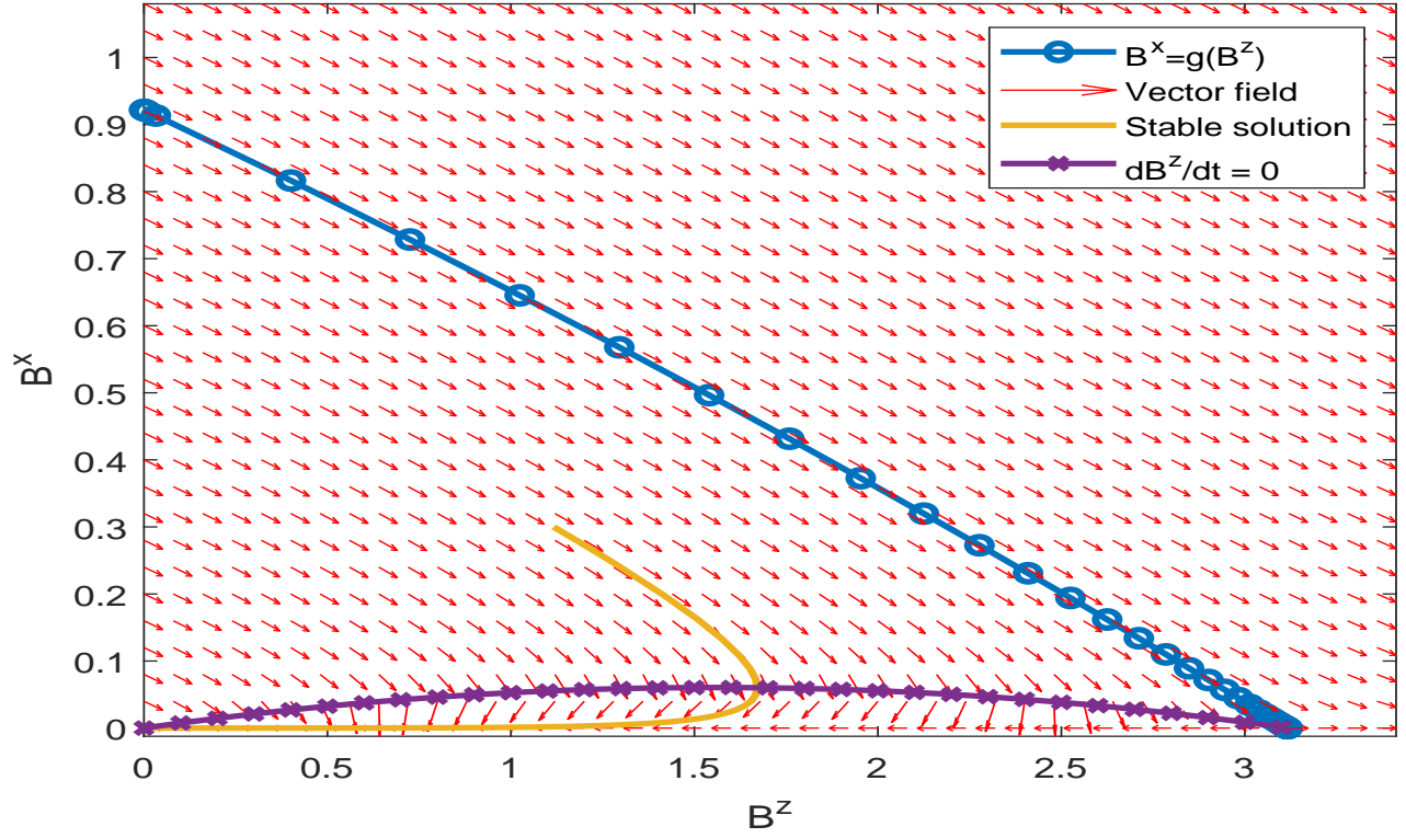
Figure 5: Vector fields
