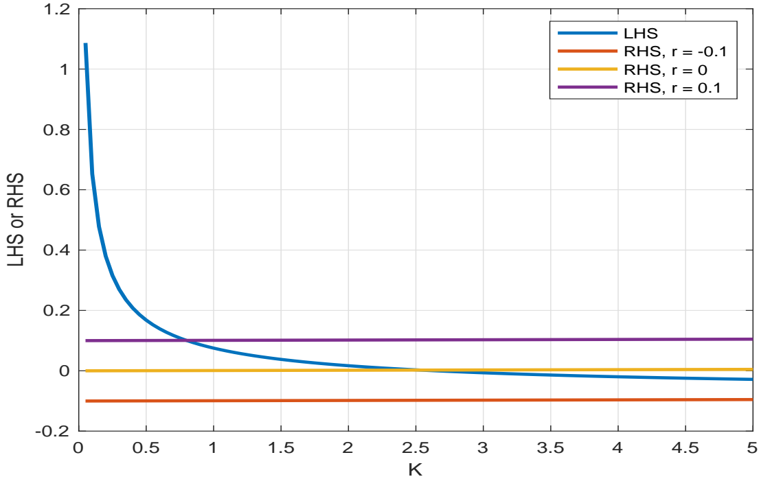
Figure 4: LHS and RHS of (37)
