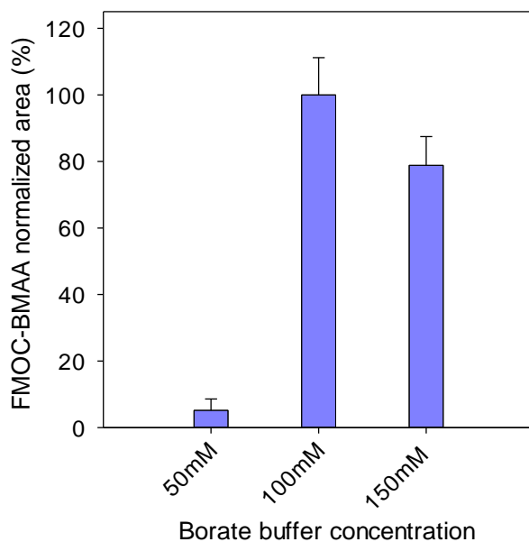
S6 Fig. Optimization of derivatization reaction: influence of borate buffer concentration on the FMOC-BMAA signal. A surface water matrix was spiked at 1000 ng L -1 with BMAA and submitted to the different conditions. Absolute areas were normalized (%) to the maximum observed among the tested conditions. Error bars represent standard deviations (n = 3).
