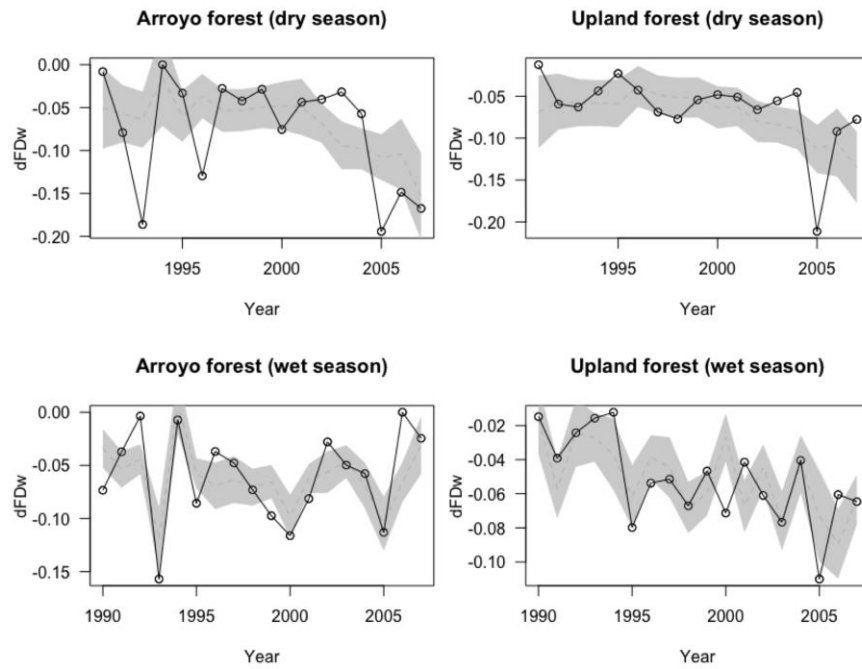
S8 Fig: Temporal dynamics for the observed dFDw (dots and lines) and 95% confidence interval predicted by the selected models (gray area).
