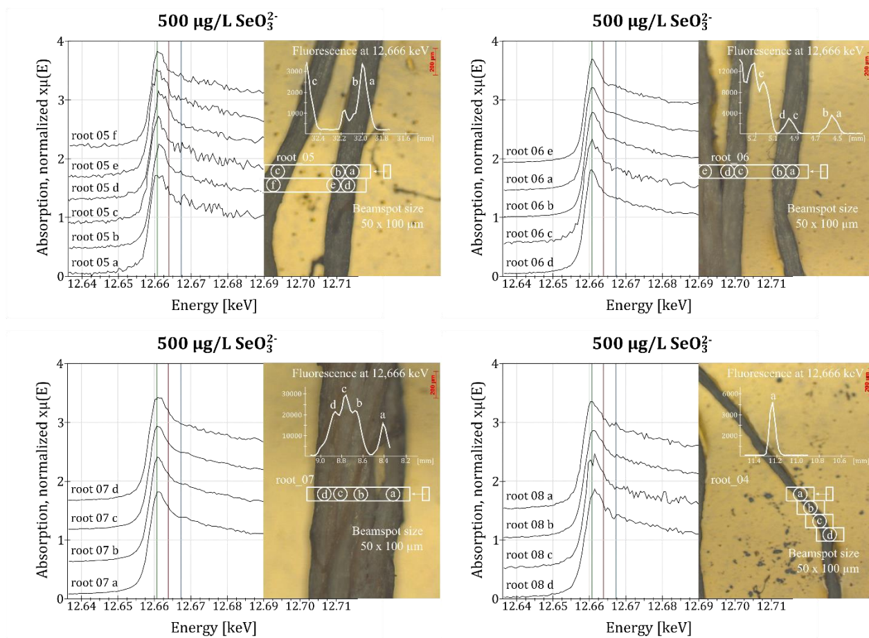
S1 Fig: all XANES spectra of each region of interest (ROI) on a rice plant treated with 500 \mu\text{g/L Se} as \text{Na}_2\text{SeO}_3 in nutrient solution
