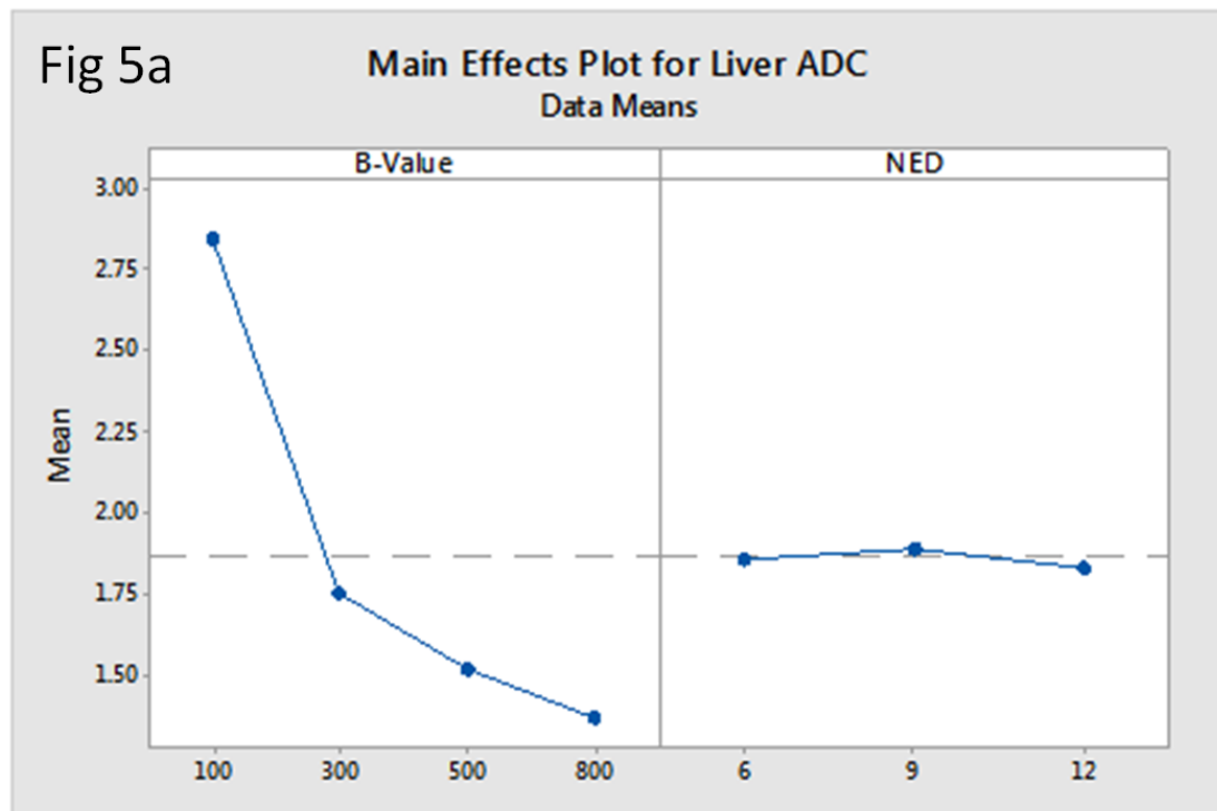
Fig 5. Results of the direct comparisons with different b-values and NED in liver ADC.
