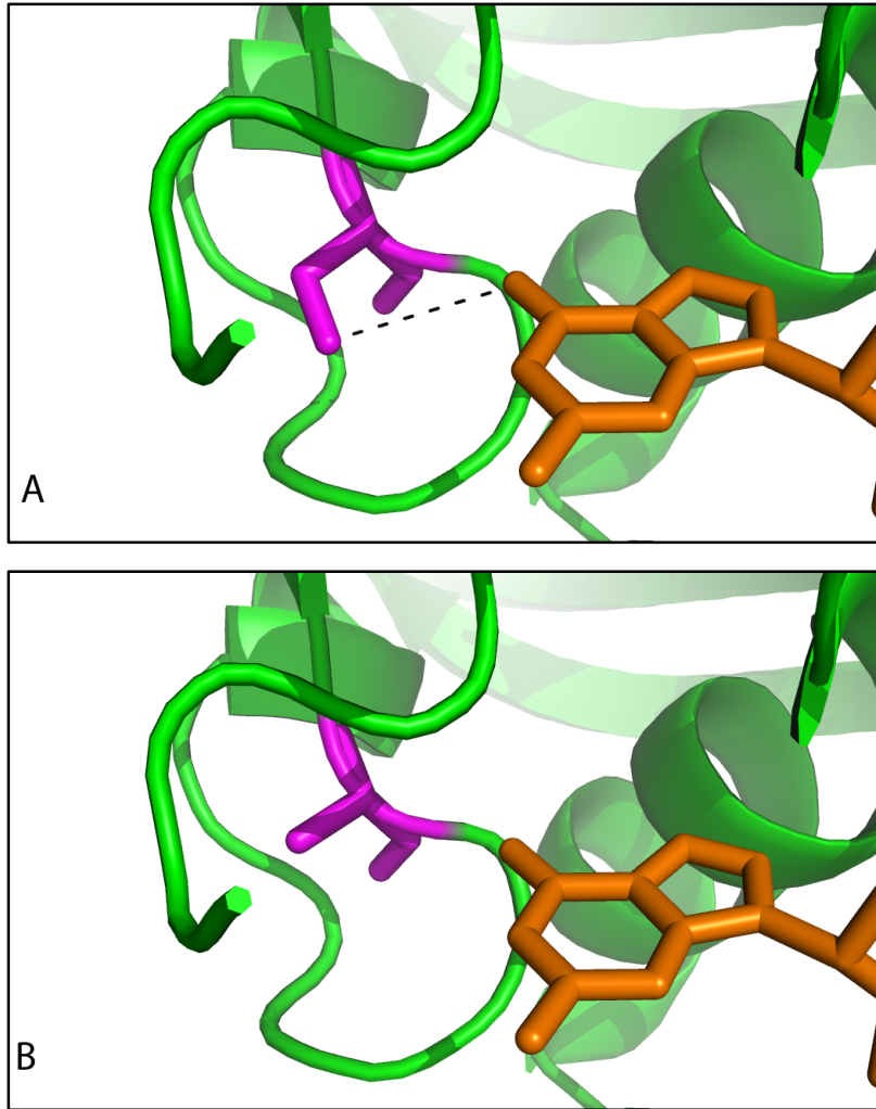
S4 Figure. Detailed view of the wild type S157 residue and its substitution S157A. Panel A shows the serine residue (in magenta) with its hydrogen bond with GDP (black dashed line, GDP in orange). Panel B shows the substitution for alanine (magenta) unable to form the hydrogen bond.
