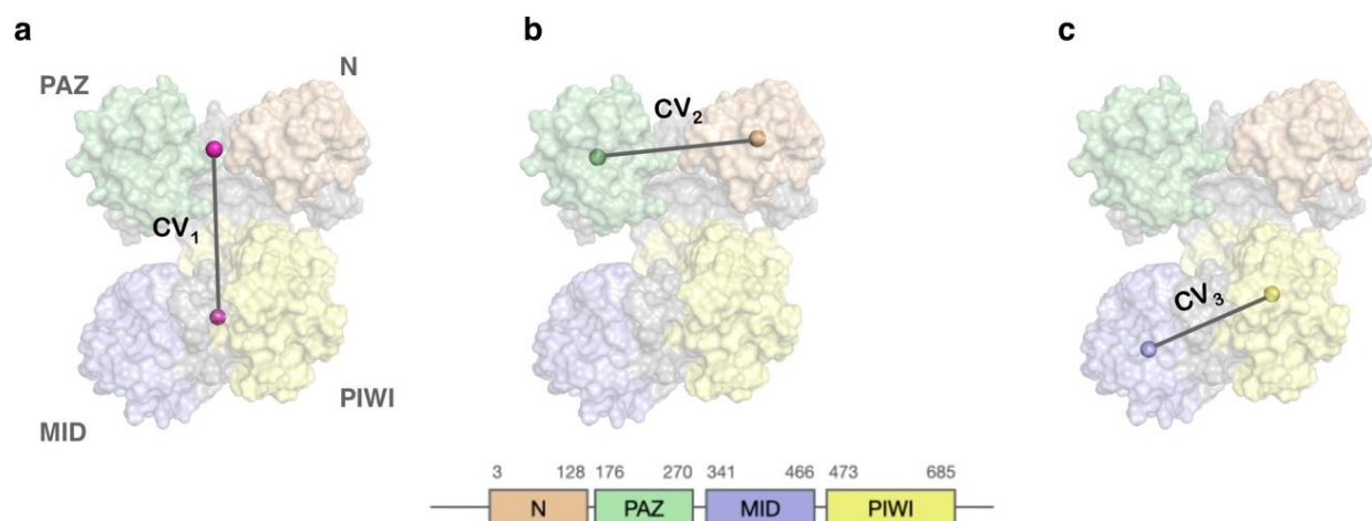
S2_Fig. Three center-of-mass (COM) distances served as collective variables. Each CV was independently biased by a potential to promote domain motions. The CVs were defined as the distance between centers-of mass of the two lobes ( a ), PAZ & N ( b ), and MID & PIWI ( c ).
