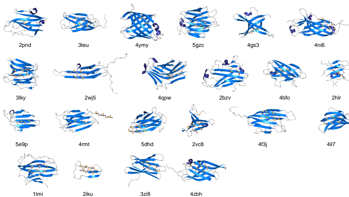
Figure S2 Test cases in the all- \beta test set solved by Fragon . The fragment placed by Phaser is shown as yellow sticks.
