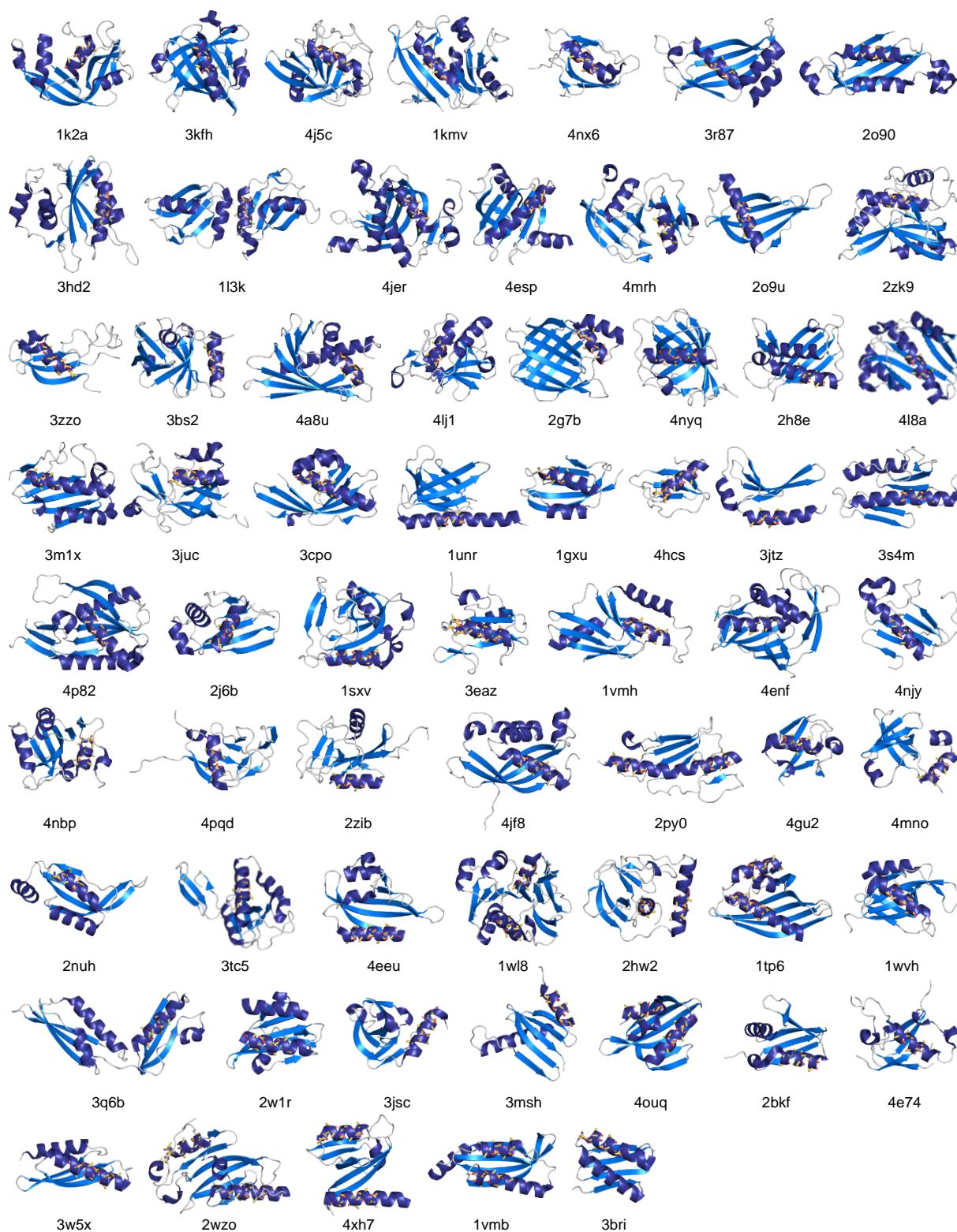
Figure S1 Test cases in the mixed \alpha/\beta test set solved by Fragon . The fragment placed by Phaser is shown as yellow sticks.
