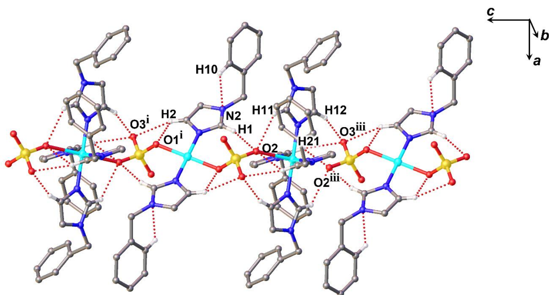
Figure S2. Intramolecular hydrogen bonding interactions in the 1D chain of the title compound. Some hydrogen atoms located at carbon atoms and lattice water and DMF solvate molecules are omitted for clarity. (symmetry codes (i) = -x+1, -y+1, -z+2 and (iii) = -x+1, -y+1, -z+1 )
