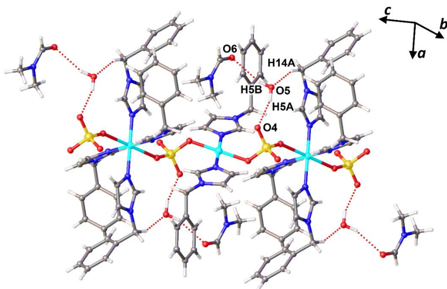
Figure S3. Intermolecular hydrogen bonding interactions between 1D chains and lattice solvent molecules of the title compound.
