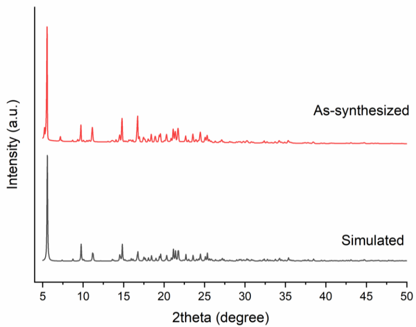
Figure S7. PXRD patterns of the title compound
