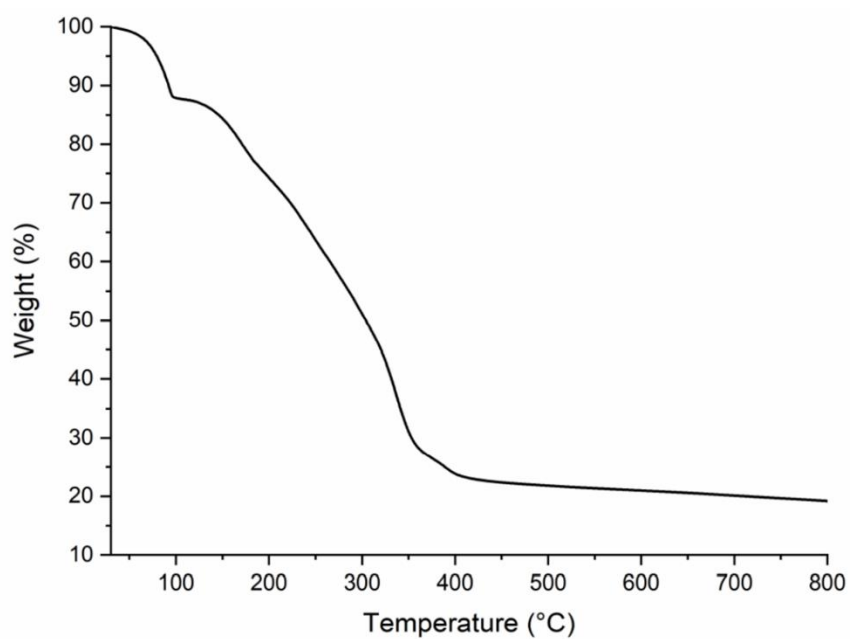
Figure S8. TGA curve of the title compound
