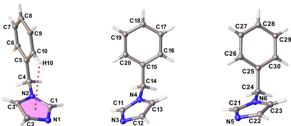
Figure S1. Conformations of bzi molecules in the title compound.
