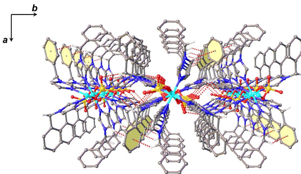
Figure S4. Side view of 2D supramolecular network in crystallographic ab plane through hydrogen bonding interactions between methylene group and sulfate ligand, and the C-H \cdots \pi interactions.
