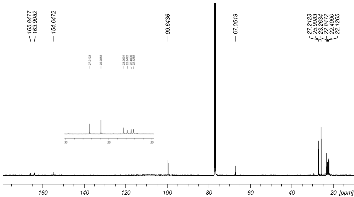
Figure S2. ^{13}\text{C} NMR spectrum of 2 in \text{CDCl}_3 .
