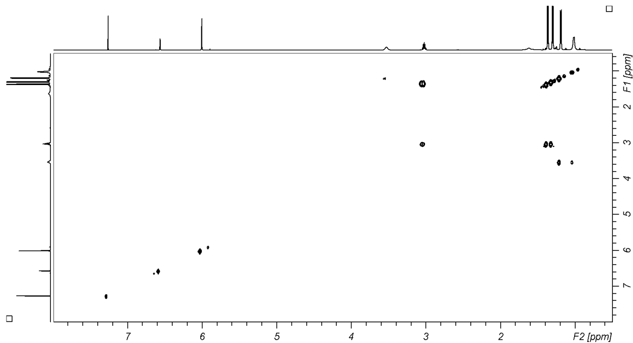
Figure S5. COSY NMR spectrum of 2 in \text{CDCl}_3 .
