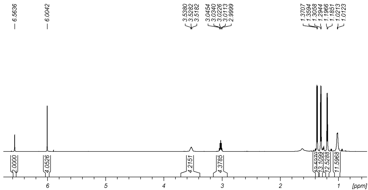
Figure S1. ^1\text{H} NMR spectrum of 2 in \text{CDCl}_3 .
