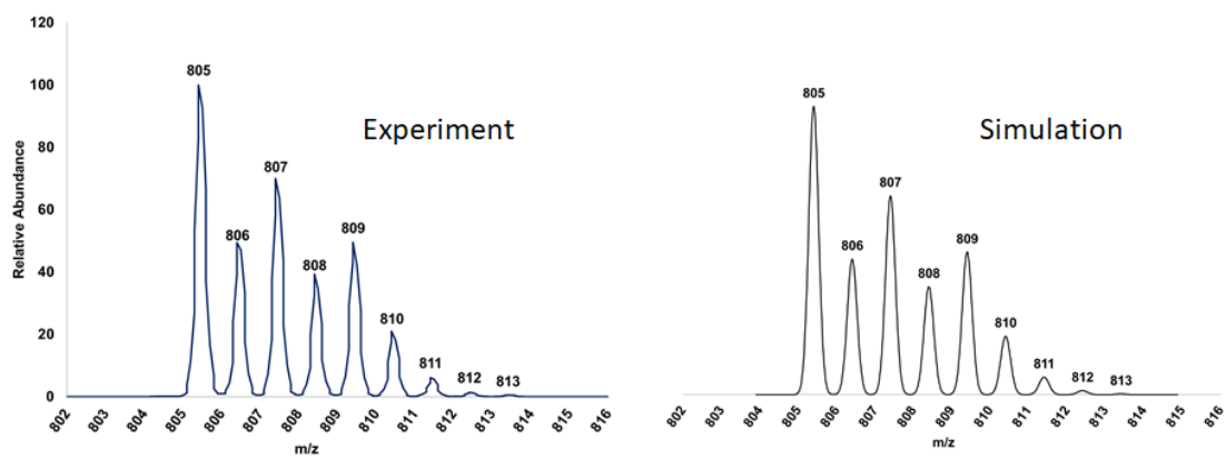
Figure S6. Experimental (left) and theoretical (right) ESI-MS spectra of 2 .
