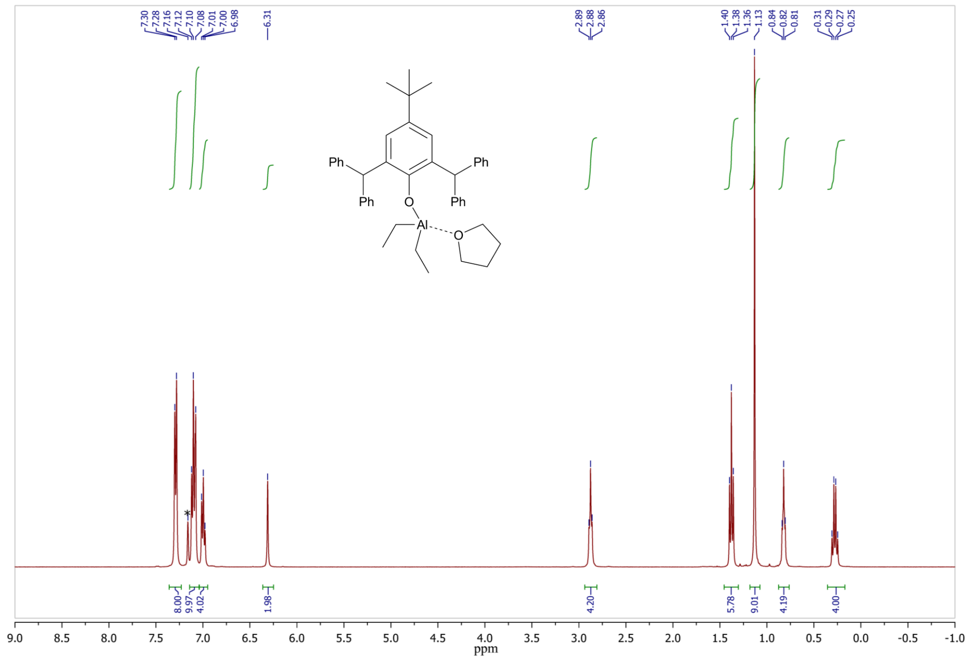
1 H NMR spectrum of {Al[O-2,6-(Ph 2 CH) 2 -4- t BuC 6 H 2 ]Et 2 (THF)} in C 6 D 6 at 400MHz.
