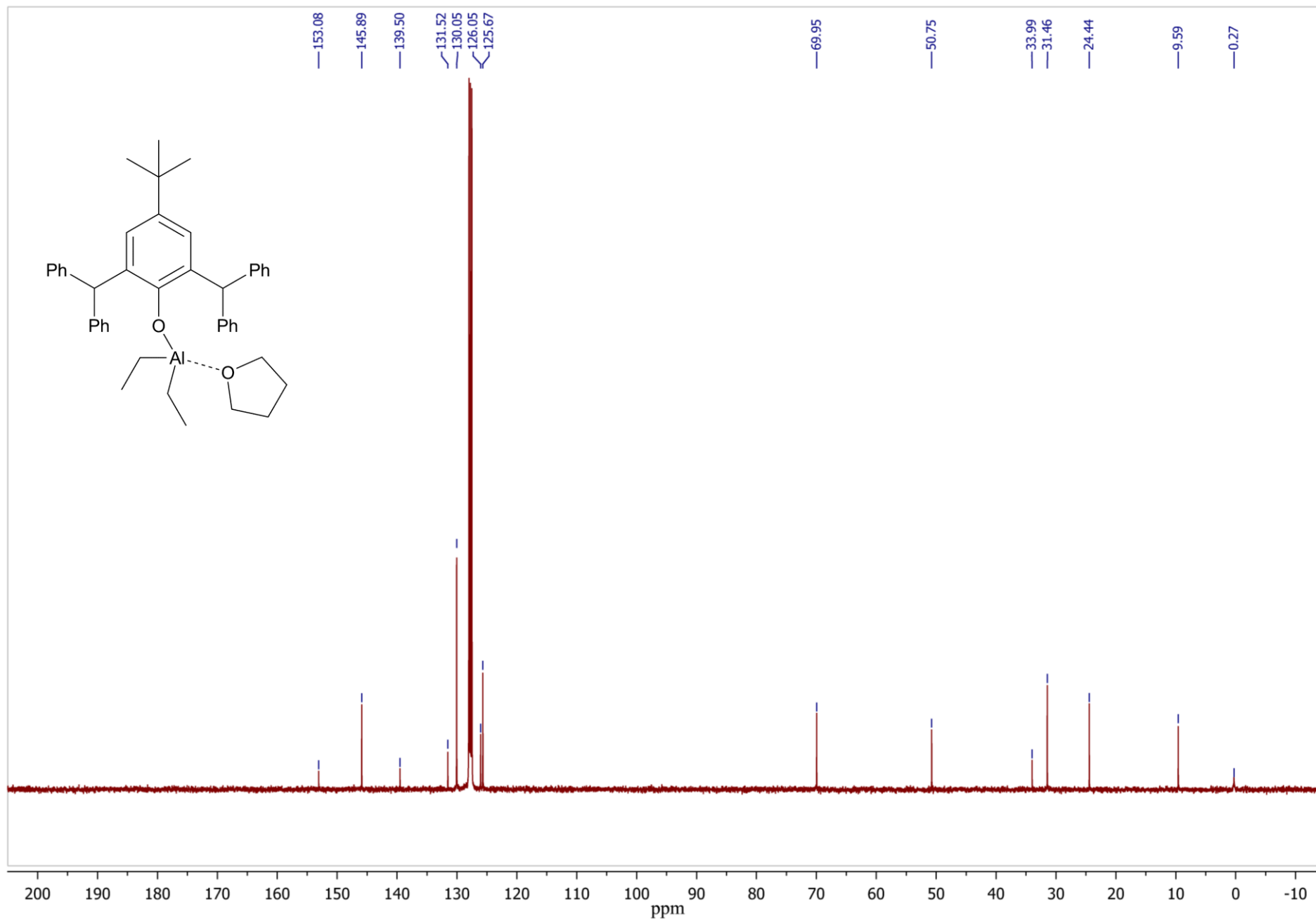
^{13}\text{C}\{^1\text{H}\} NMR spectrum of \{\text{Al}[\text{O}-2,6-(\text{Ph}_2\text{CH})_2-4\text{-}^t\text{BuC}_6\text{H}_2]\text{Et}_2(\text{THF})\} in \text{C}_6\text{D}_6 at 100MHz.
