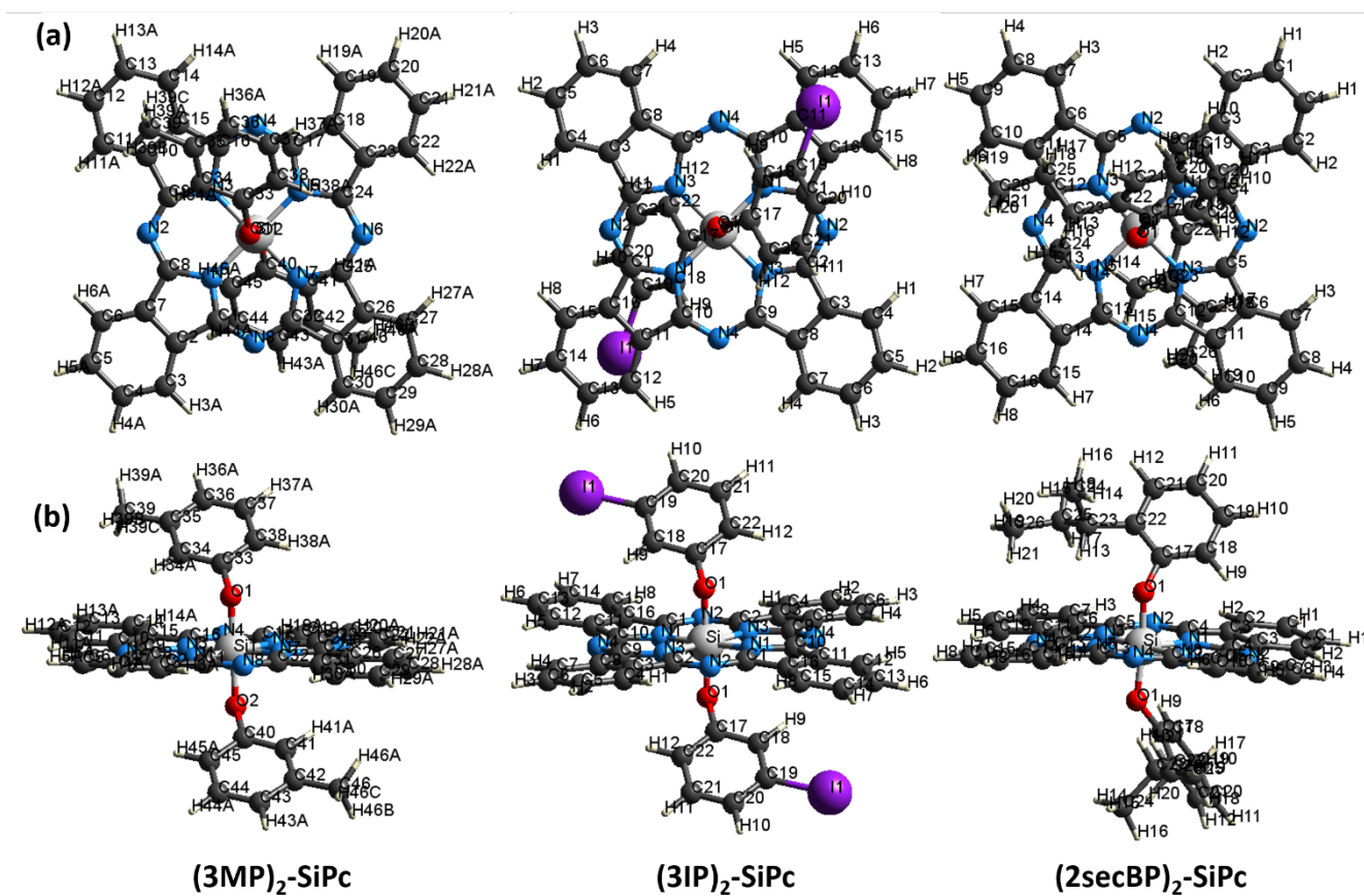
Scheme S1. – Labeled crystal structure organizations of (3MP) 2 -SiPc (left), (3IP) 2 -SiPc (middle) and (2secBP) 2 -SiPc (right), obtained by single crystal x-ray diffraction where A) top view and B) side view.
