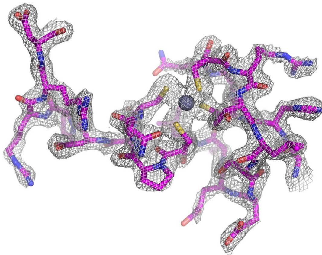
Figure S1 Representative 2mFo-DFc electron density for the Cys4 zinc finger domain, contoured at 1.6 r.m.s.d. The zinc finger domain is shown in magenta stick representation and the zinc ion is shown as a grey sphere.
