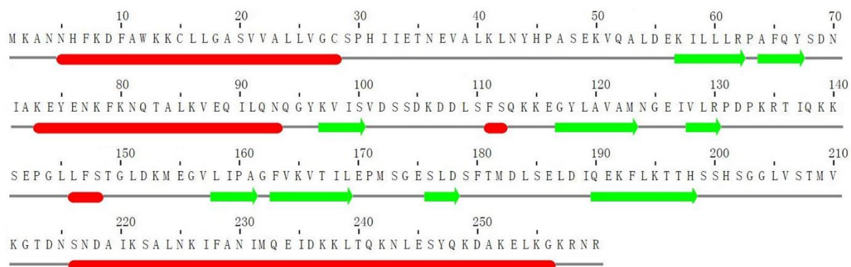
Figure S1 The predicted secondary structure of HpaA using Jpred4 (Drozdetskiy et al. , 2015). Helices are indicated as red tubes, sheets as green arrows, and loops as grey lines.
