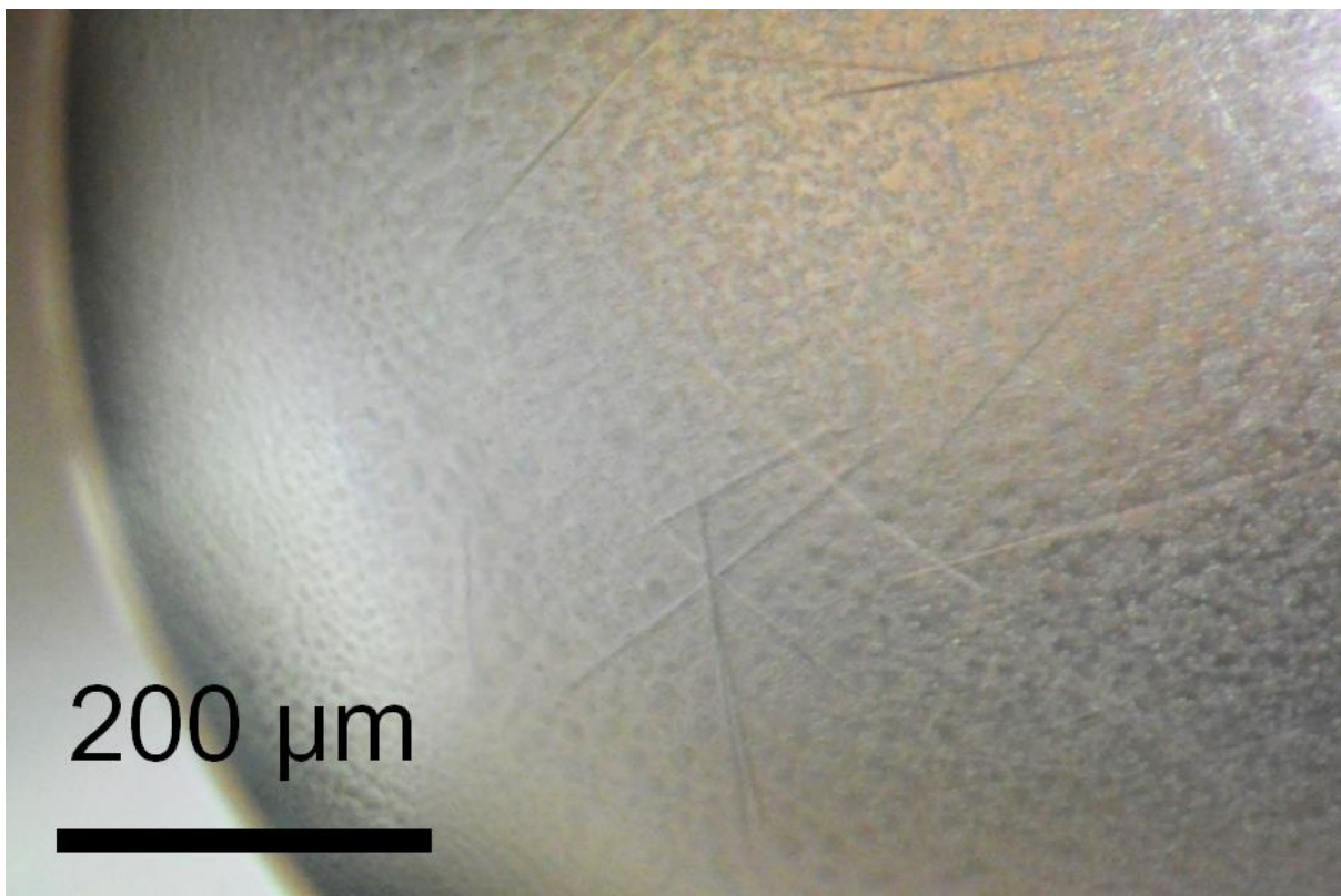
Figure S1 AfPAz crystals. The reservoir solution of 400 \mu\text{L} was poured in 0.5 mL sample cups and 1.0 \mu\text{L} protein solution (10 mg/mL AfPAz) was mixed with 1.0 \mu\text{L} reservoir solution on siliconized cover glass plates. The composition of reservoir solution was 0.2 M Sodium acetate trihydrate, 0.1 M Sodium cacodylate trihydrate pH 6.5, and 35% w/v Polyethylene glycol 8,000.
