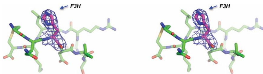
Figure S3 Composite omit map generated in Phenix (Adams et al. , 2010) for F3H mediotope variant and contoured at \sigma=1.0 . Only a section of the map is shown (in blue).
