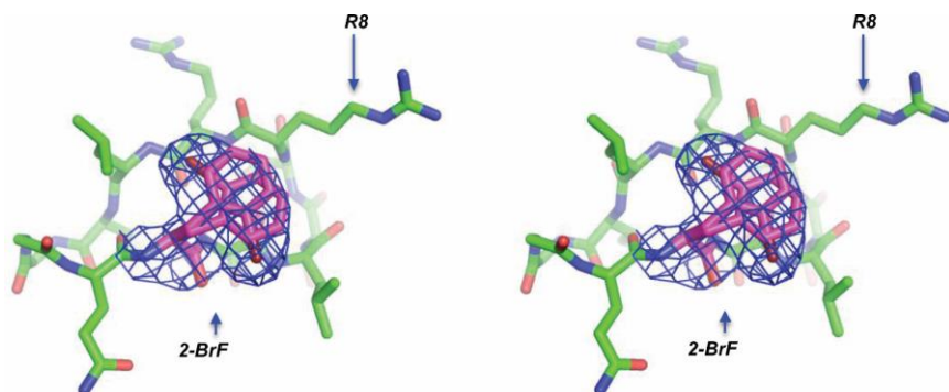
Figure S2 Composite omit map generated in Phenix (Adams et al. , 2010) for 2-bromophenylalanine mediotope variant and contoured at \sigma=1.0 . Only a section of the map is shown (in blue).
