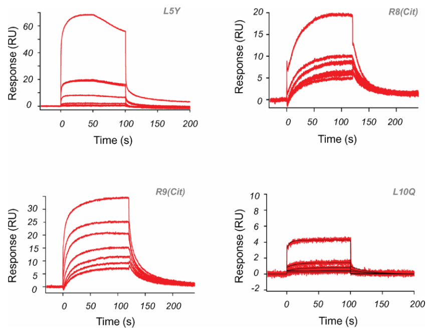
Figure S1 SPR sensograms of cetuximab – meditope variant interactions at 25°C.
