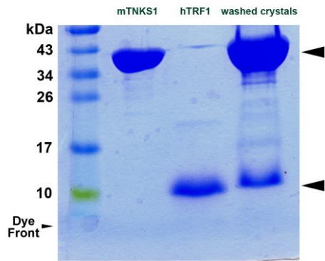
Supplementary Figure S1. SDS-PAGE analysis of crystal content. Carefully washed TNKS1-TRF1 complex crystals were dissolved in SDS loading buffer and analyzed by SDS-PAGE and stained with Coomassie Blue, along with mTNKS1(308-655) and hTRF1(1-55) controls.
