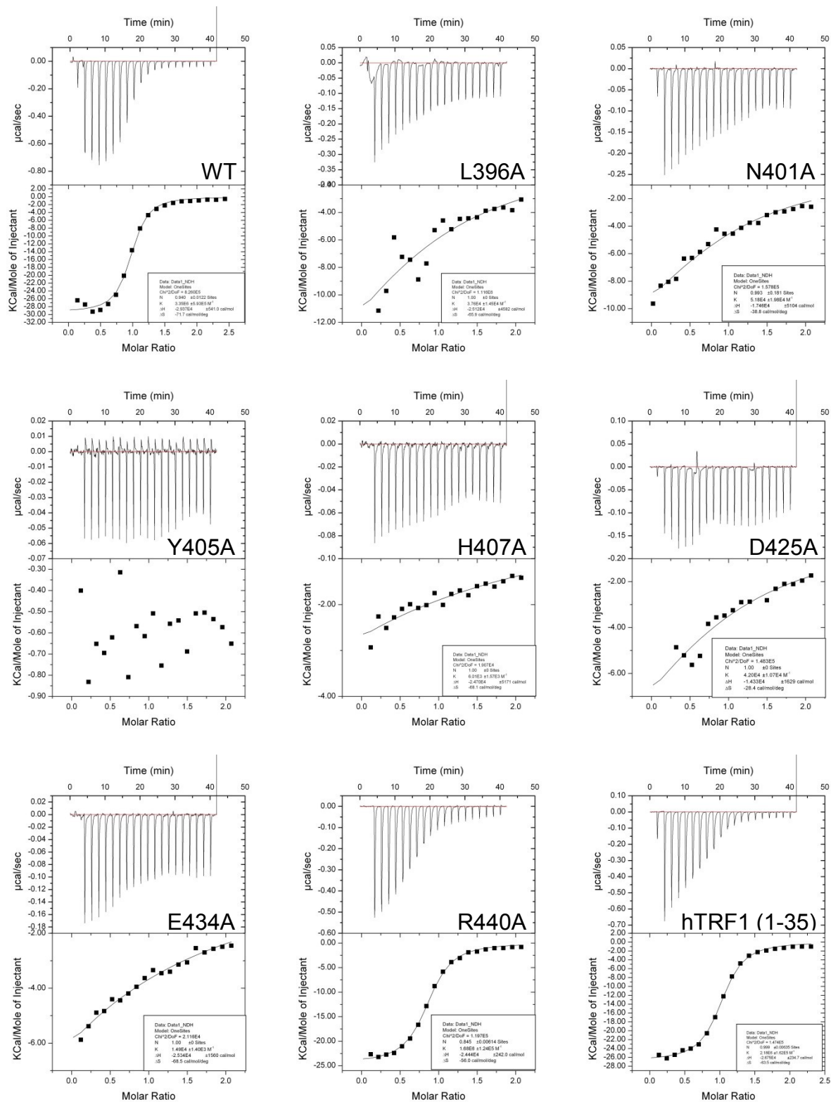
Supplementary Figure S2. Original data for ITC analysis.
