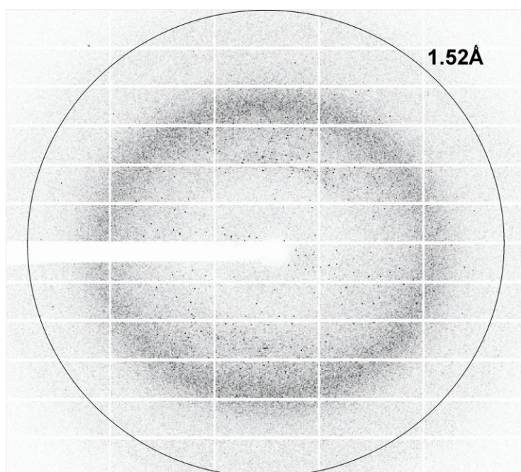
Figure S1 Diffraction image of ctCBM54.
