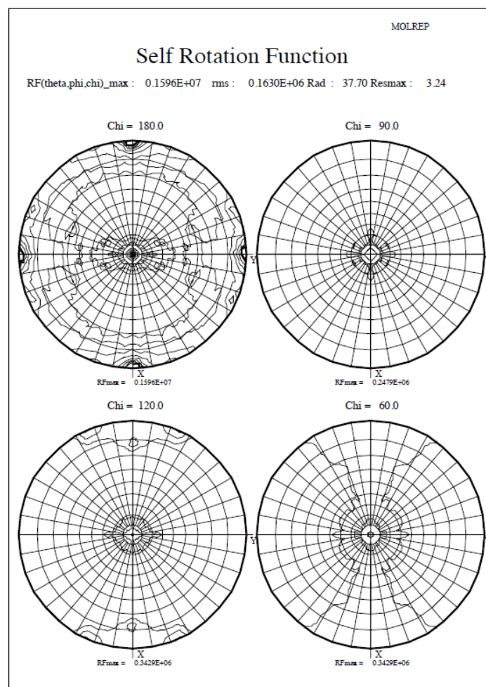
Figure S1 The self-rotation function of LFAI crystals.
