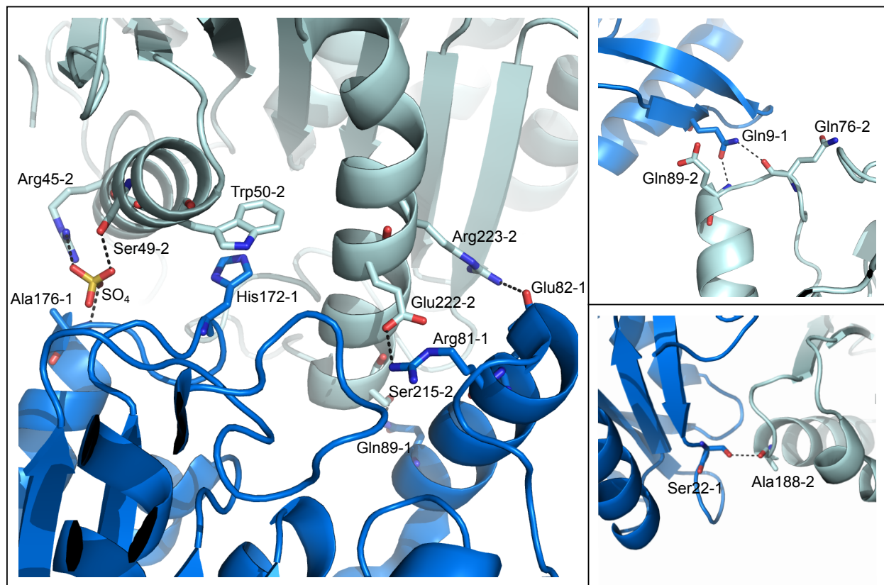
Figure S1: The three protein interfaces of the P2_12_1 crystal.
