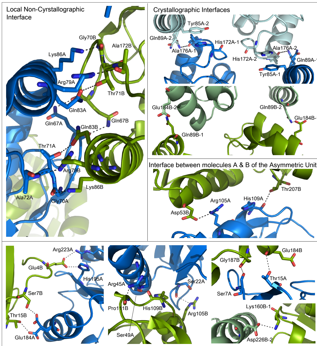
Figure S2: The eight protein interfaces of the C2 crystal
