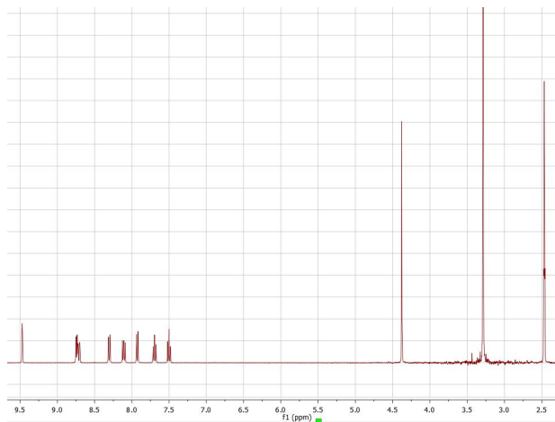
1 H NMR spectrum (iodide salt)
