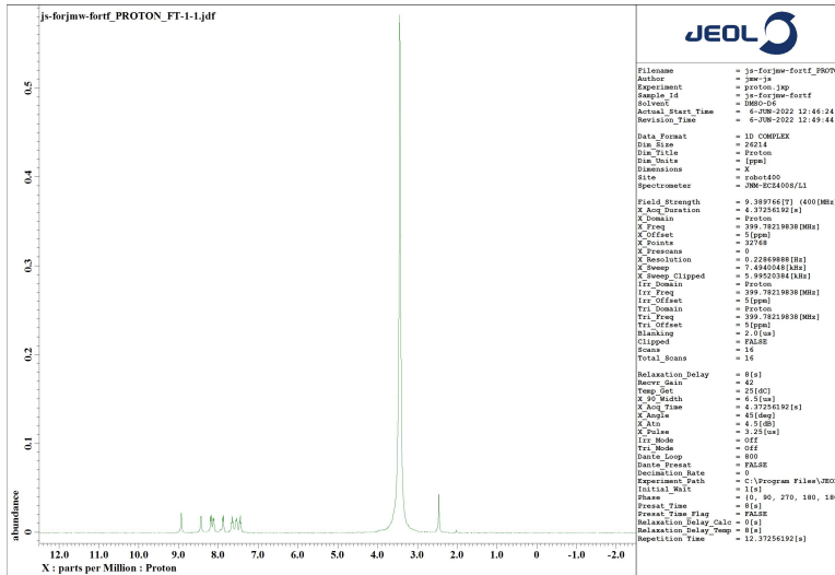
1 H NMR spectrum (free base)
