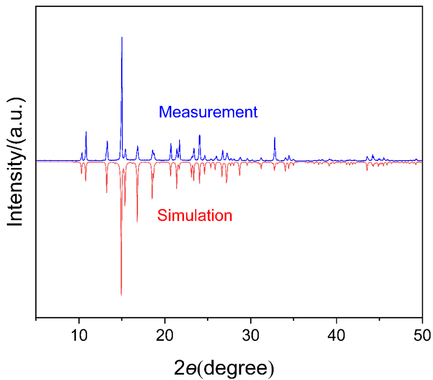
Figure S1 The powder X-ray diffraction (PXRD) pattern of 1 was measured at room temperature, verifying the purity of the bulk phase.
