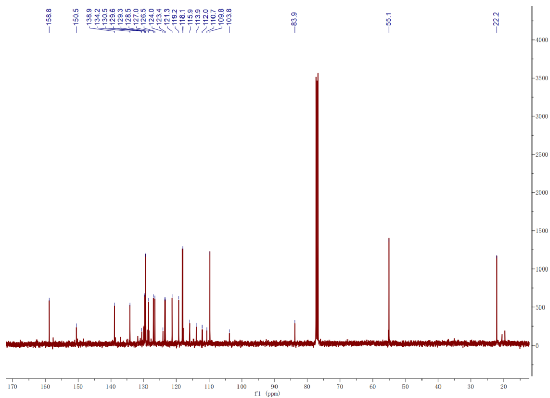
Figure S1 1 H NMR of NP4
