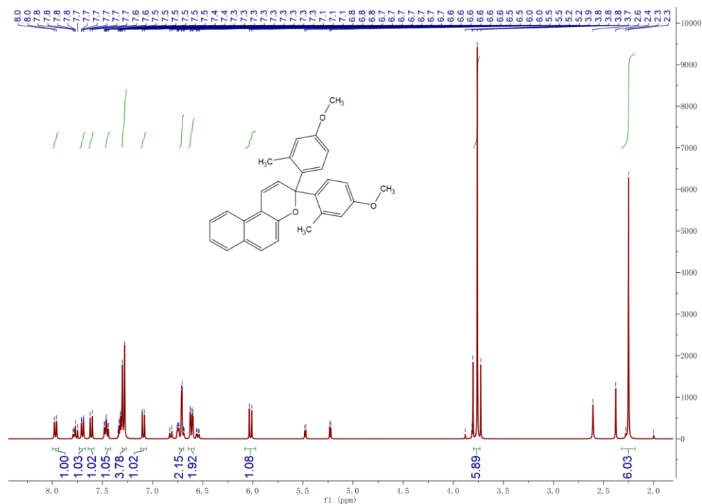
Figure S1 1 H NMR of NP4
