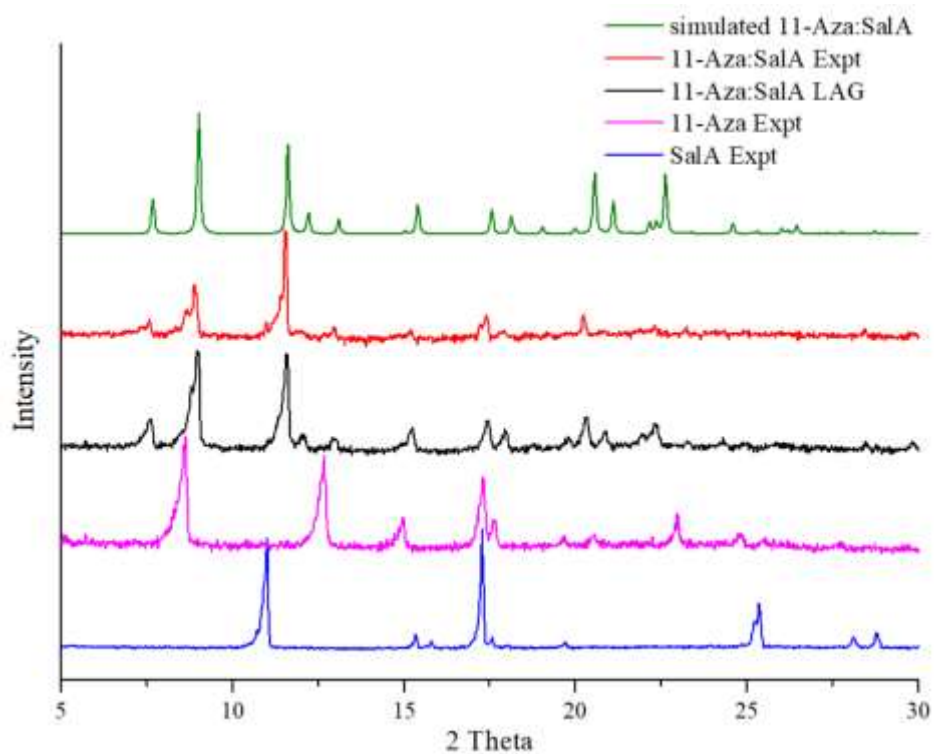
Figure 1. Powder XRD patterns of 11-Aza:SalA 1.
