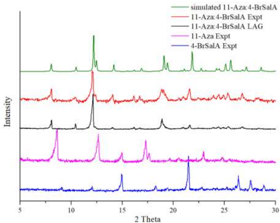
Figure 3. Powder XRD patterns of 11-Aza:4-BrSalA 3.
