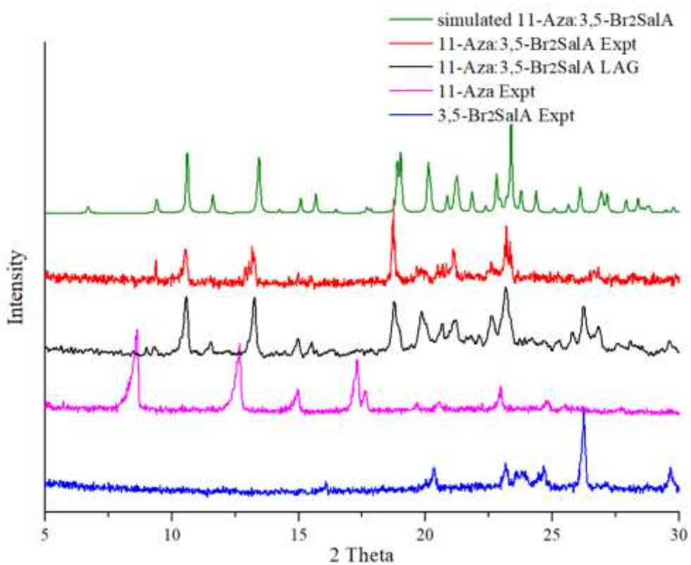
Figure 4. Powder XRD patterns of 11-Aza:3,5-Br 2 SalA 4.
