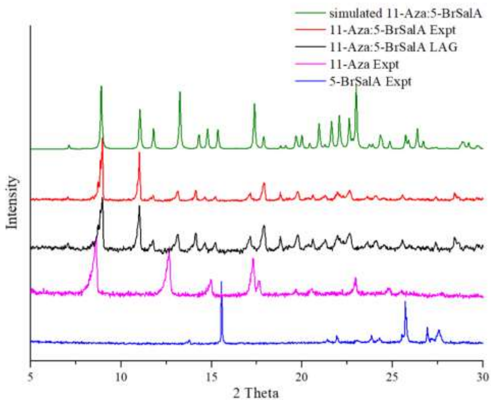
Figure 2. Powder XRD patterns of 11-Aza:5-BrSalA 2.
