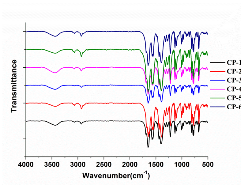
Fig. S1 FT-IR spectra of CP1-6
