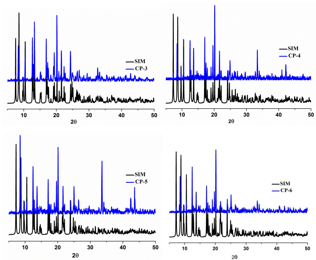
Fig. S2 PXR D patterns of CP1-6 at room temperature. Blue patterns correspond to the experimental data obtained using the as-synthesized bulk samples. Black patterns were simulated from the single crystal X-ray data.
