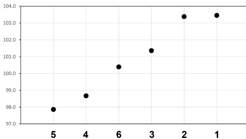
Figure S4 Plot of the c axis in ascending length order for structures 1–6
