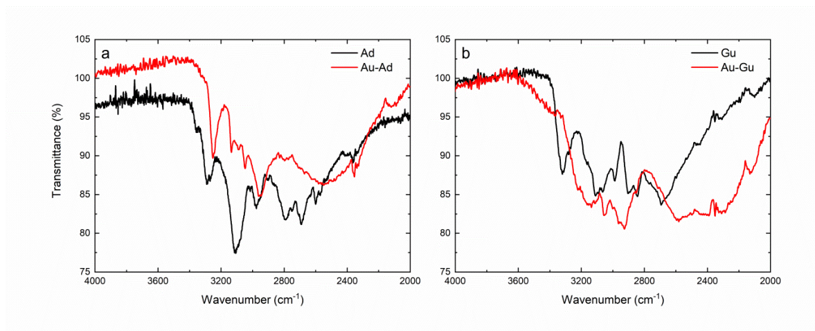
Figure S1 FTIR spectra of adenine (Ad) and compound 1 (Au-Ad) (a) and of guanine (Gu) and compound 2 (Au-Gu) (b).
