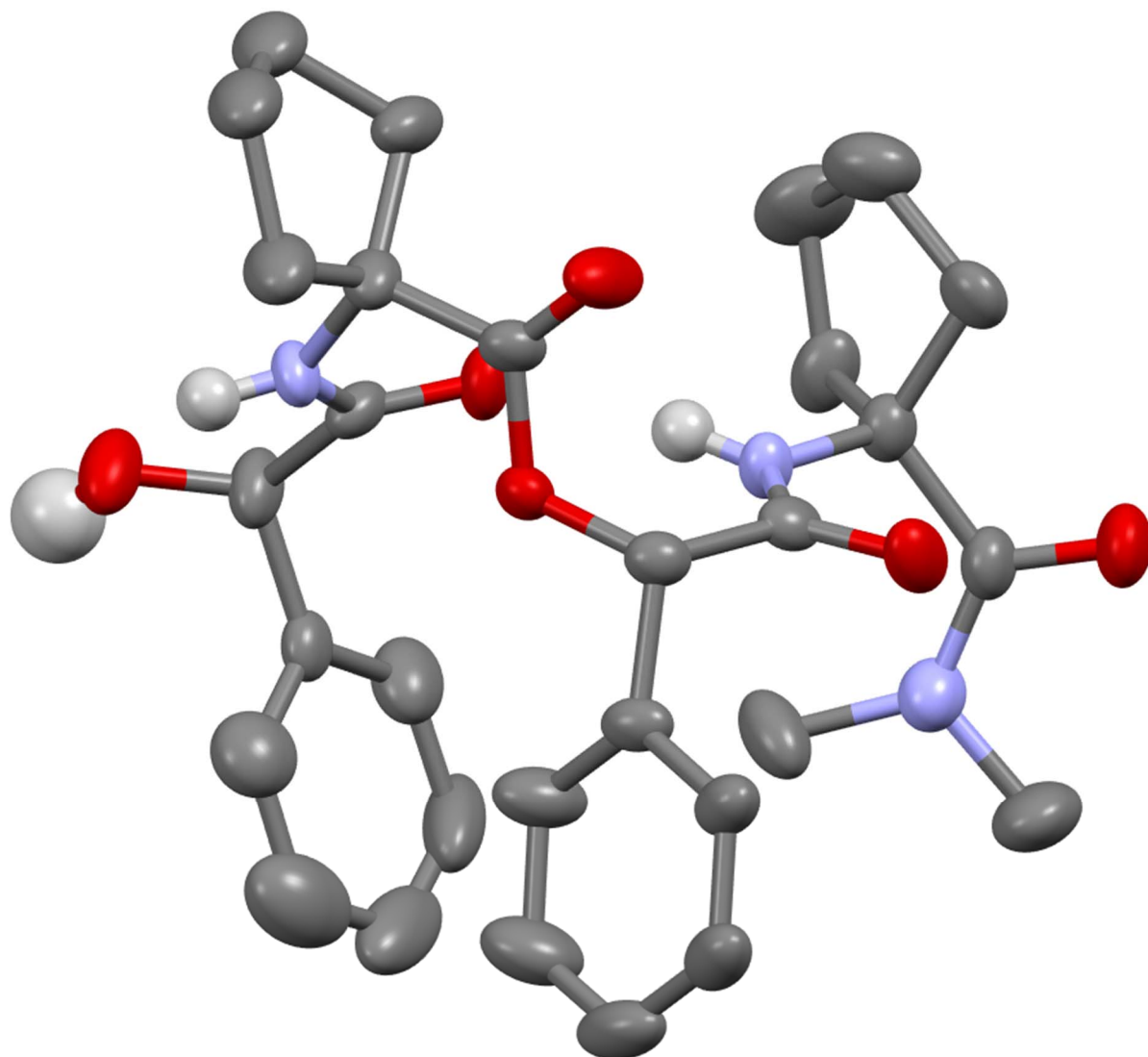
Figure S2 View of the molecule of (5c) showing the second conformation of the disordered five-membered ring (top left). Displacement ellipsoids are drawn at the 50% probability level. Most H atoms have been omitted for clarity.
