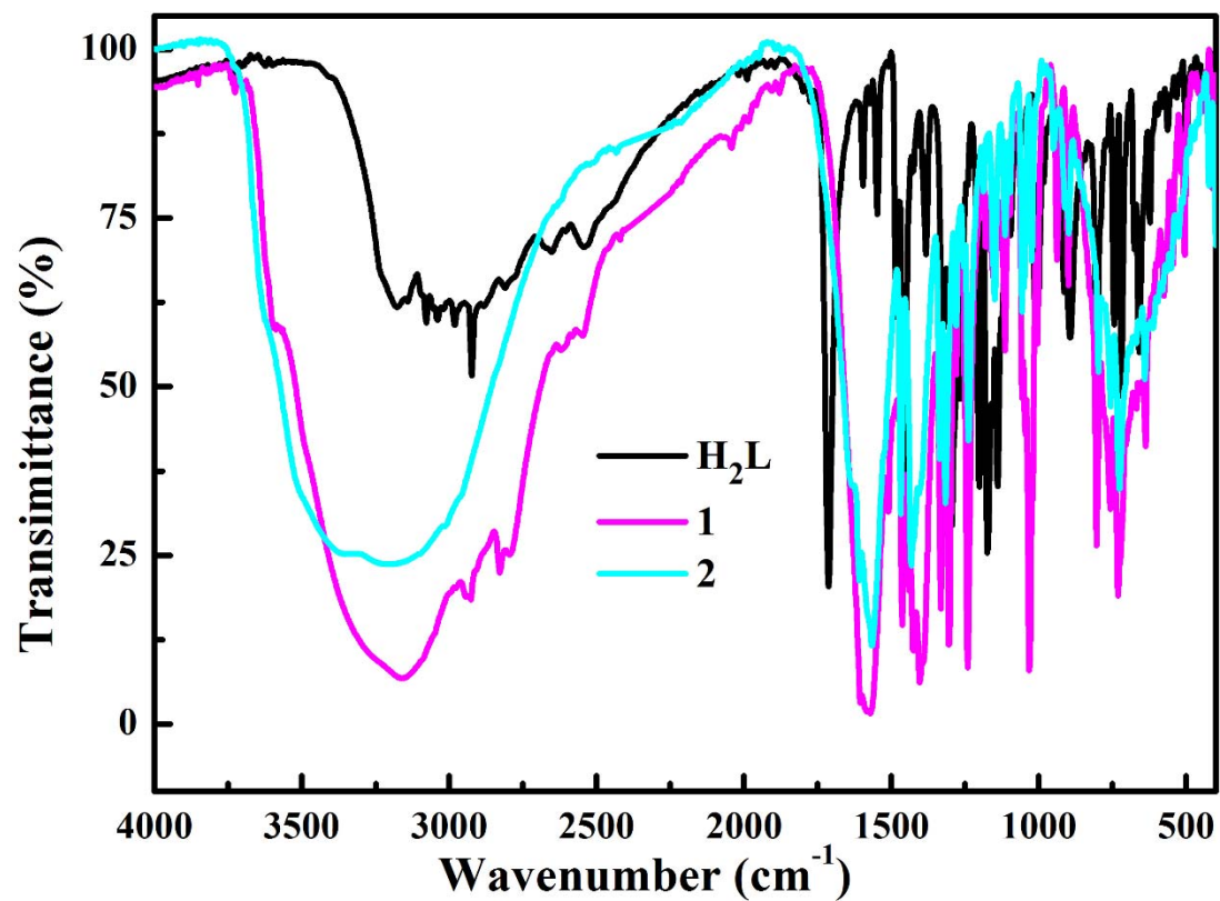
Figure S1 IR spectra of H 2 L, 1 and 2.
