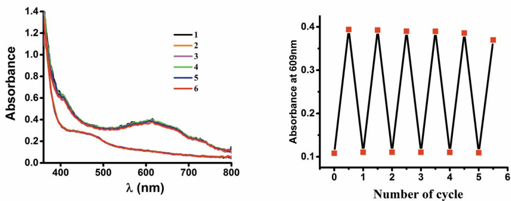
Fig. S2. The excellent colouration-decolouration phenomena of 1 indicate a possible application in the detection of UV light.
