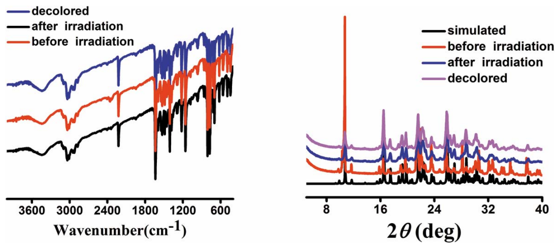
Fig. S1. (Left) The IR spectra and (right) the PXRD patterns for 1 .
