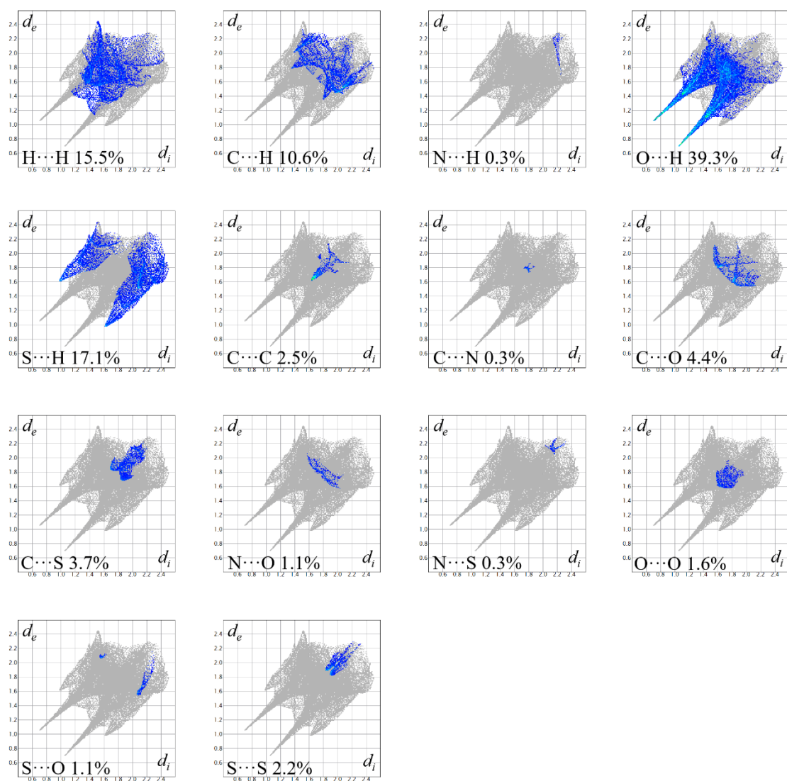
Figure S1 Decomposed 2D fingerprint plots for 1 showing different close contacts and their relative contributions.
