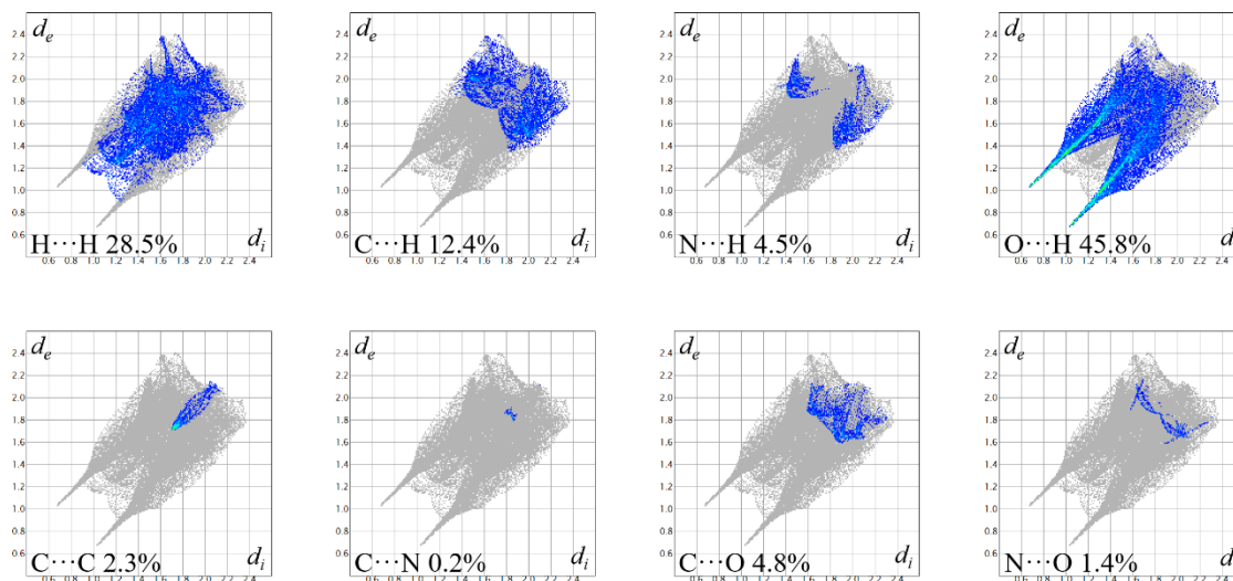
Figure S2 Decomposed 2D fingerprint plots for 4 showing different close contacts and their relative contributions.
