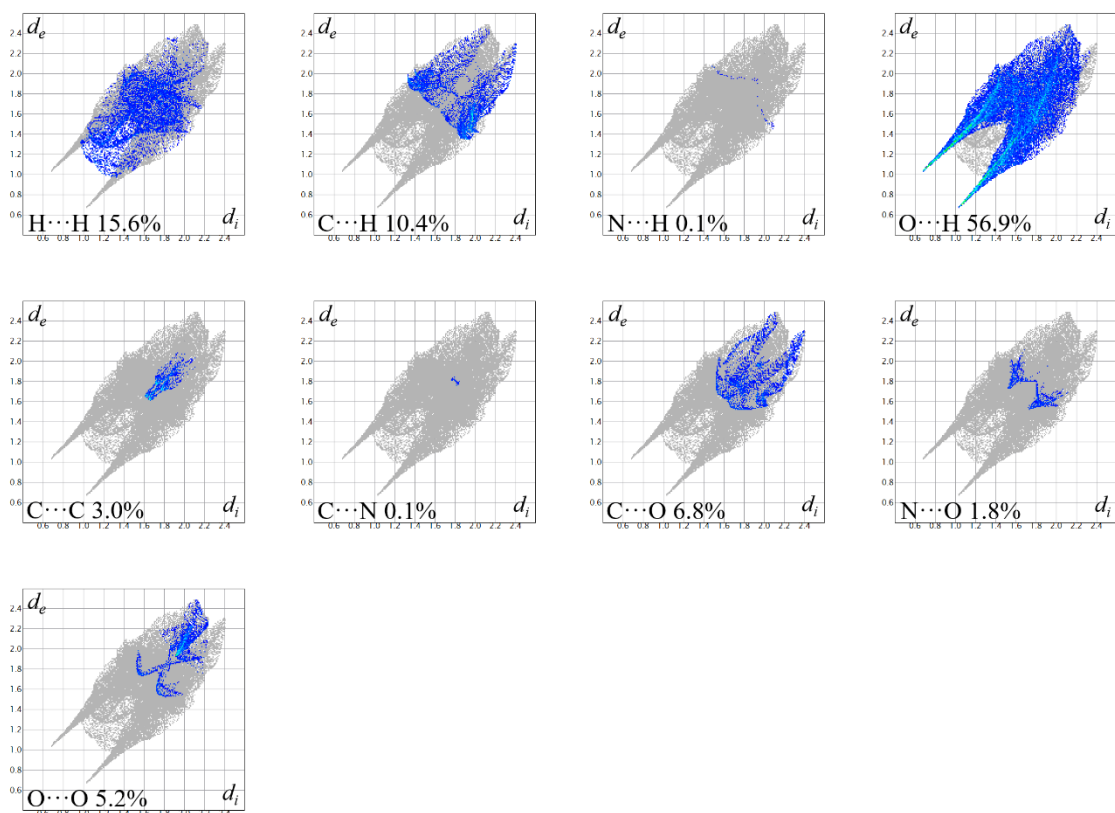
Figure S3 Decomposed 2D fingerprint plots for 5 showing different close contacts and their relative contributions.
