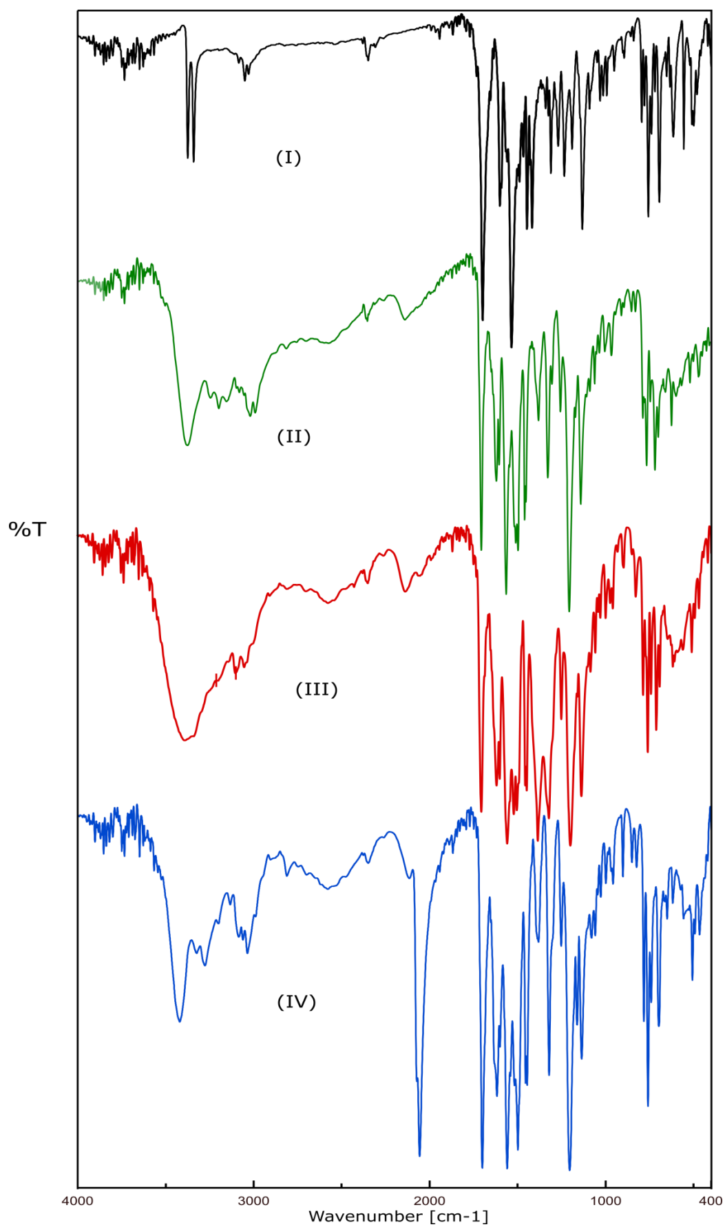
Figure S3 Infrared spectra of the compounds.
