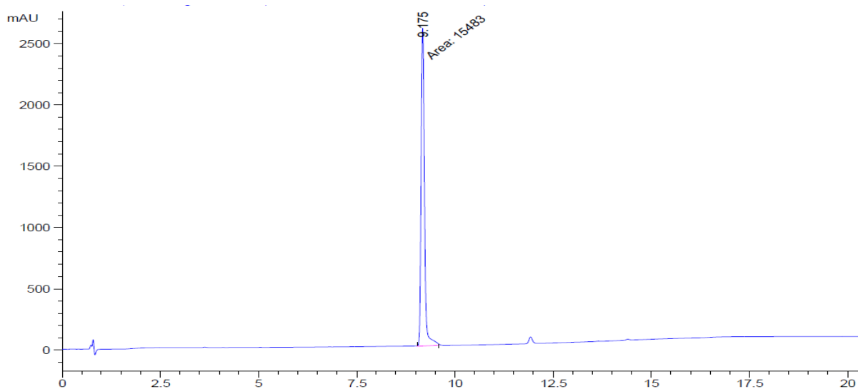
Figure S49 HPLC for compound A17
