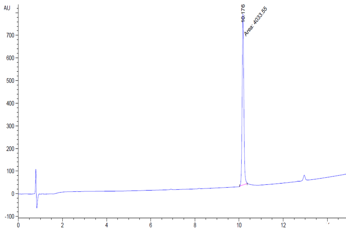
Figure S52 HPLC for compound A18
