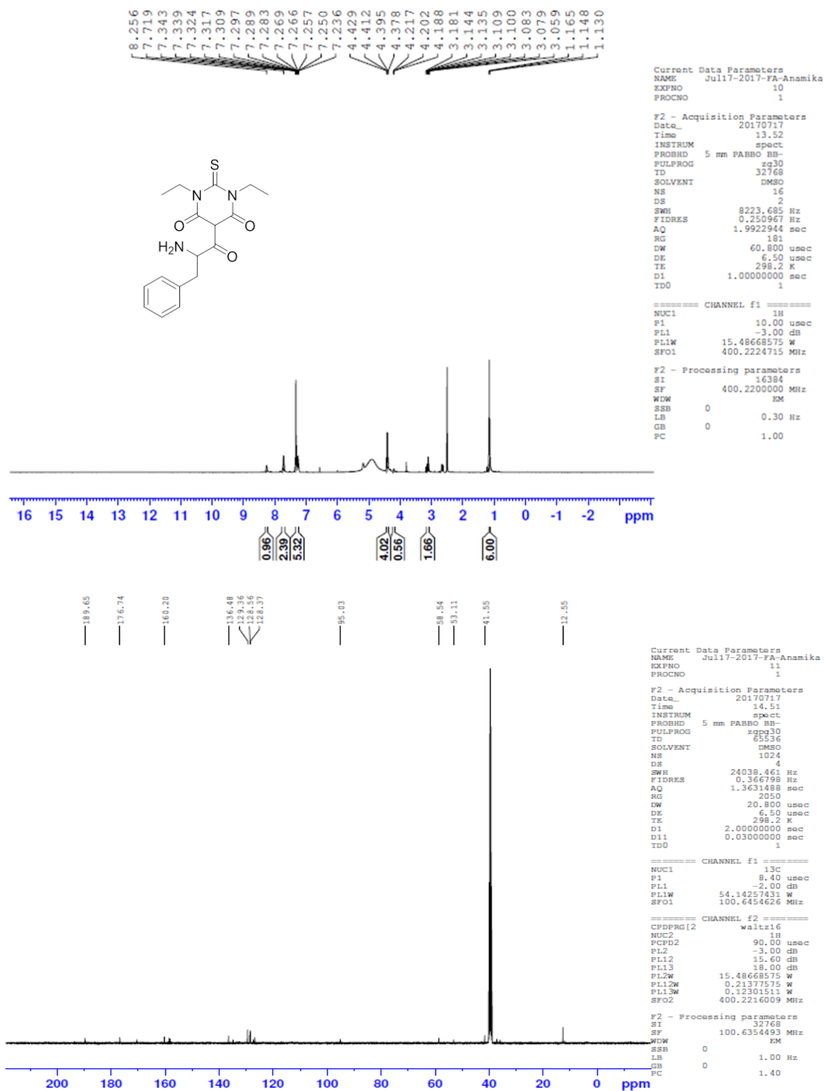
Figure S15 1 H NMR and 13 C NMR of compound A05
