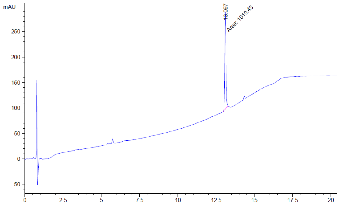
Figure S7 HPLC for compound A03
