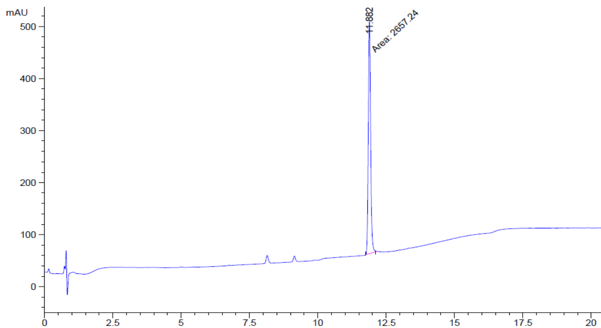
Figure S1 HPLC for compound A01
