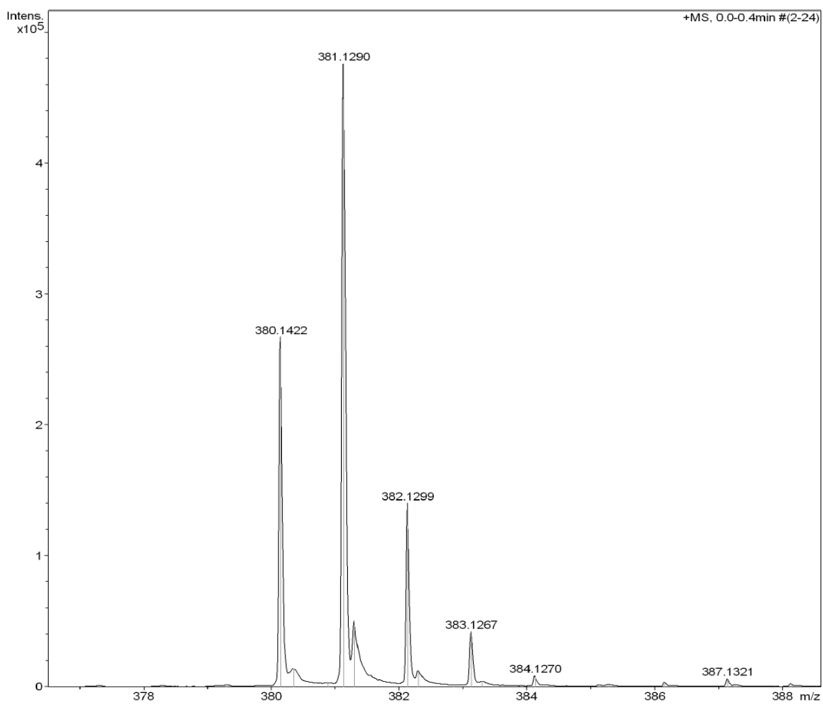
Figure S47 HRMS for compound A16
