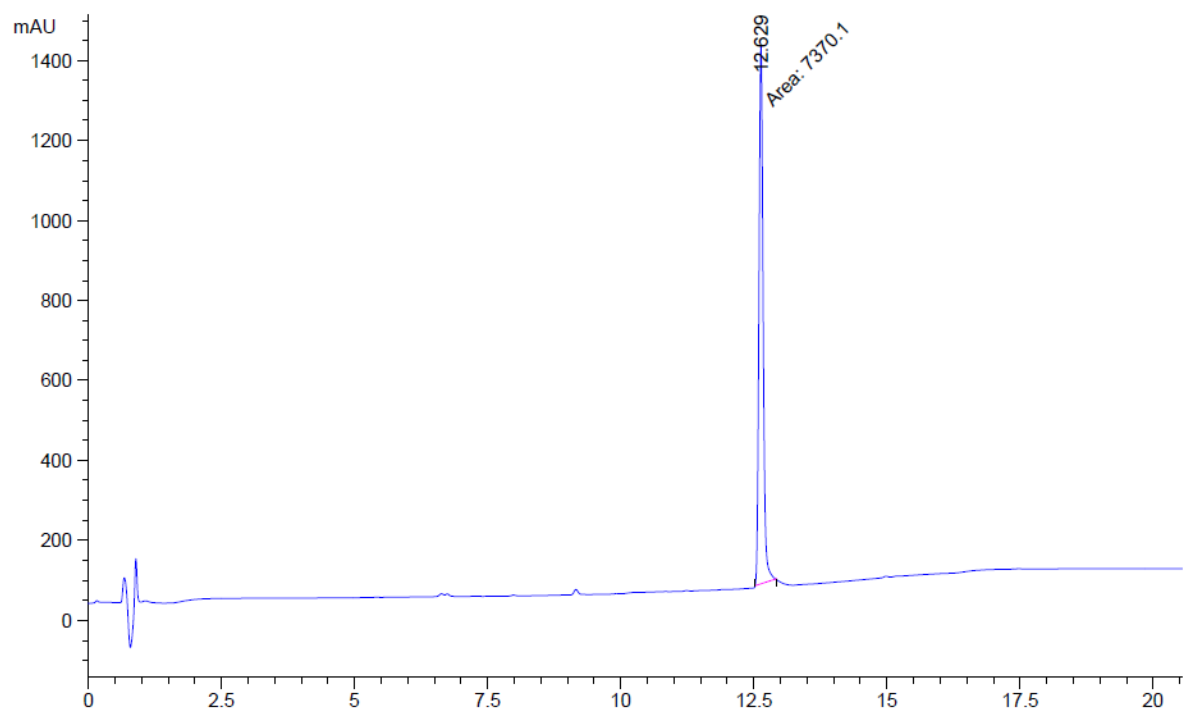
Figure S25 HPLC for compound A09
