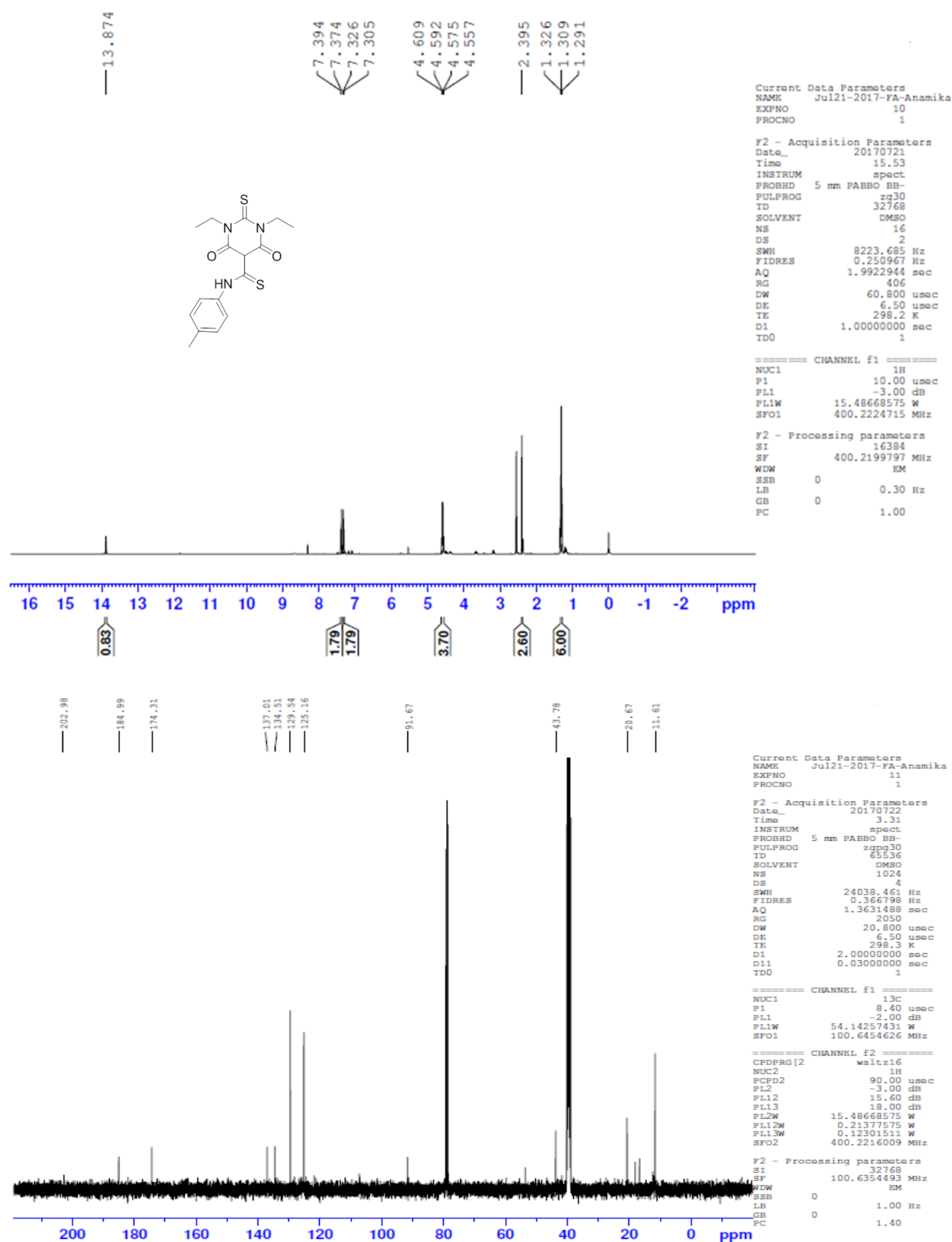
Figure S39 1 H NMR and 13 C NMR of compound A13
