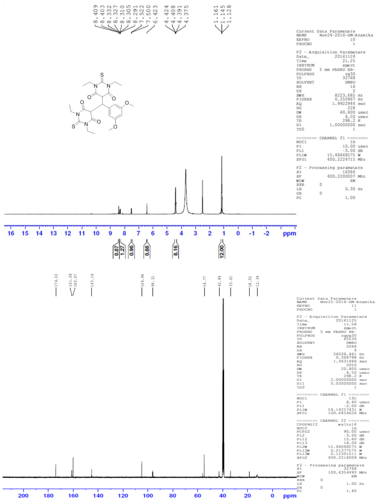
Figure S33 ^1\text{H} NMR and ^{13}\text{C} NMR of compound A11
