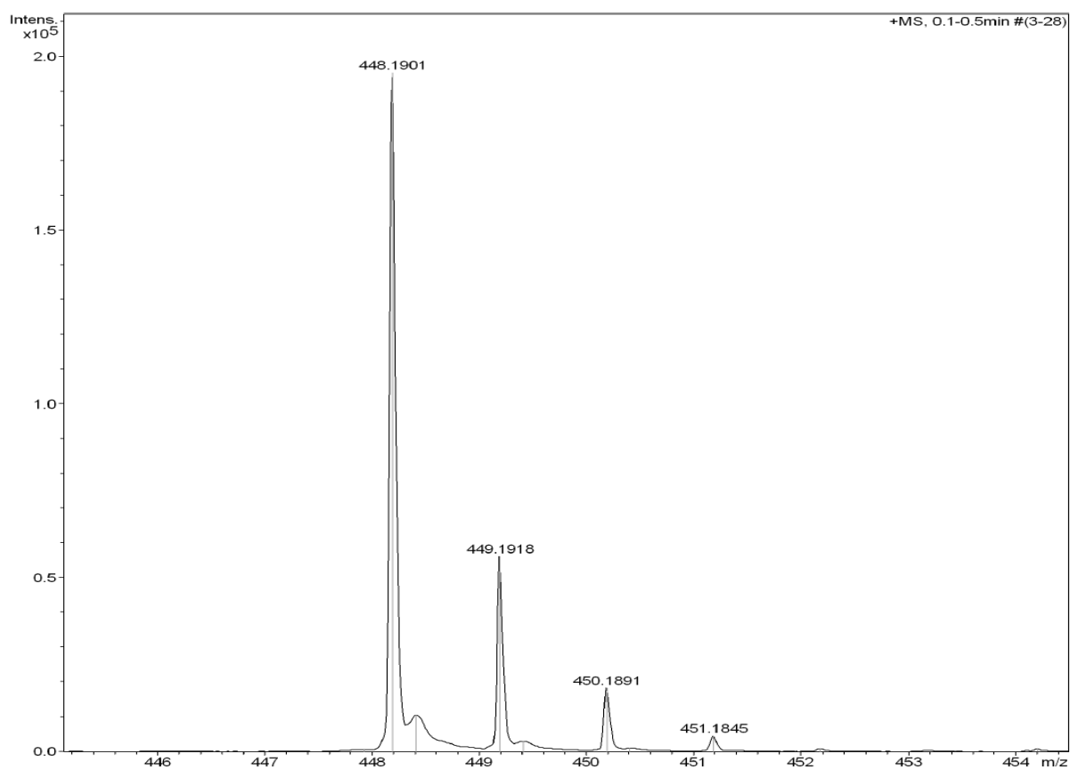
Figure S11 HRMS for compound A04
