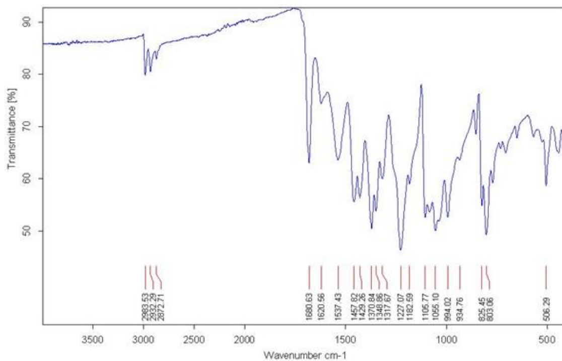
Figure S61 IR for compound A02
