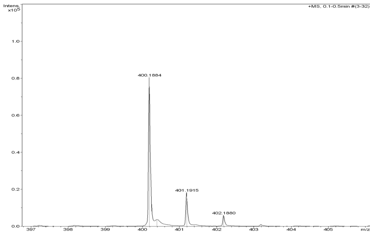
Figure S17 HRMS for compound A06
