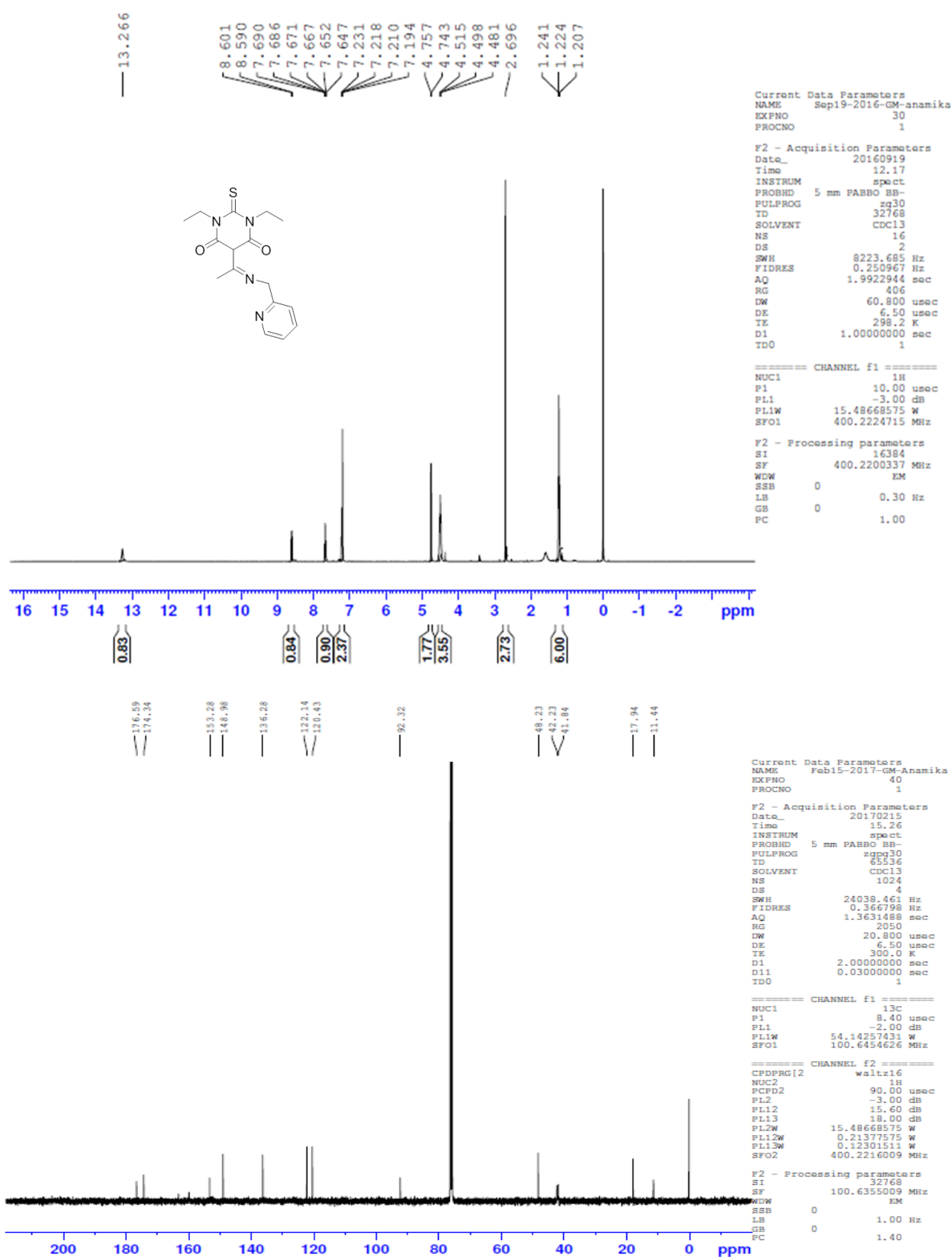
Figure S24 1 H NMR and 13 C NMR of compound A08
