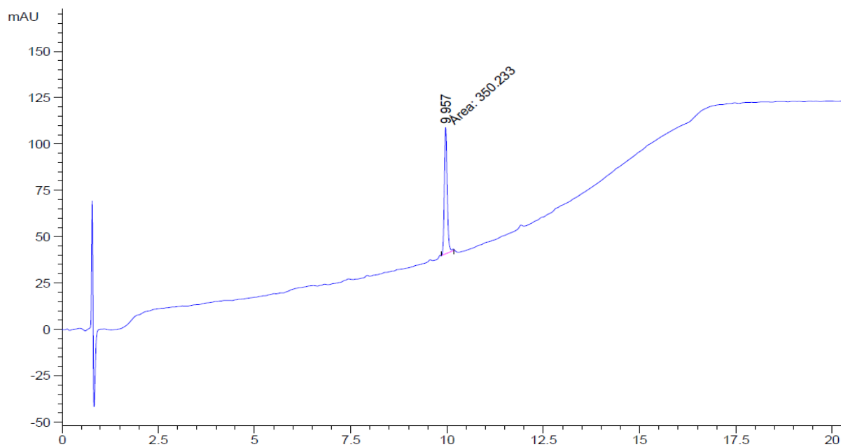
Figure S54 HPLC for compound A19
