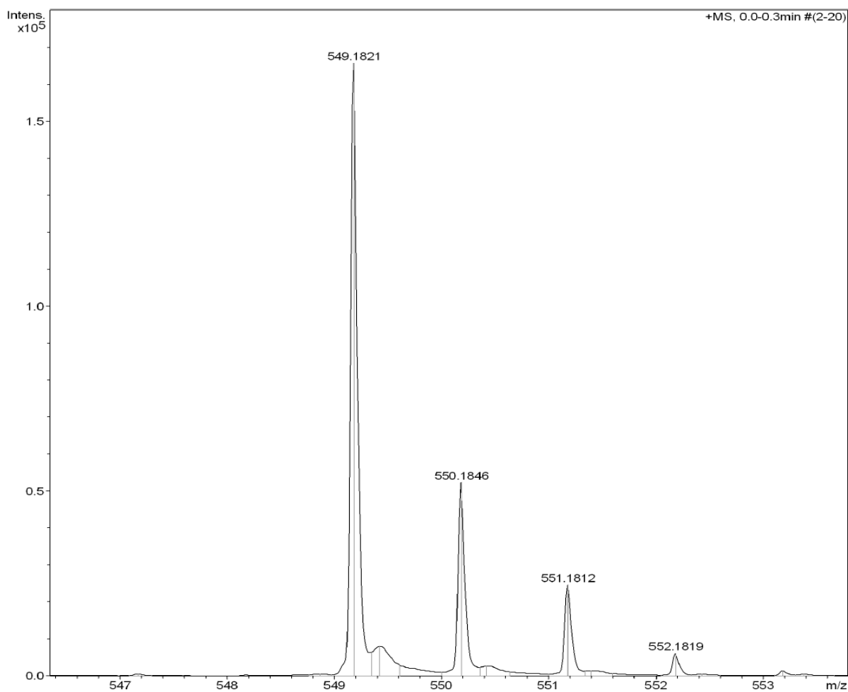
Figure S32 HRMS for compound A11
