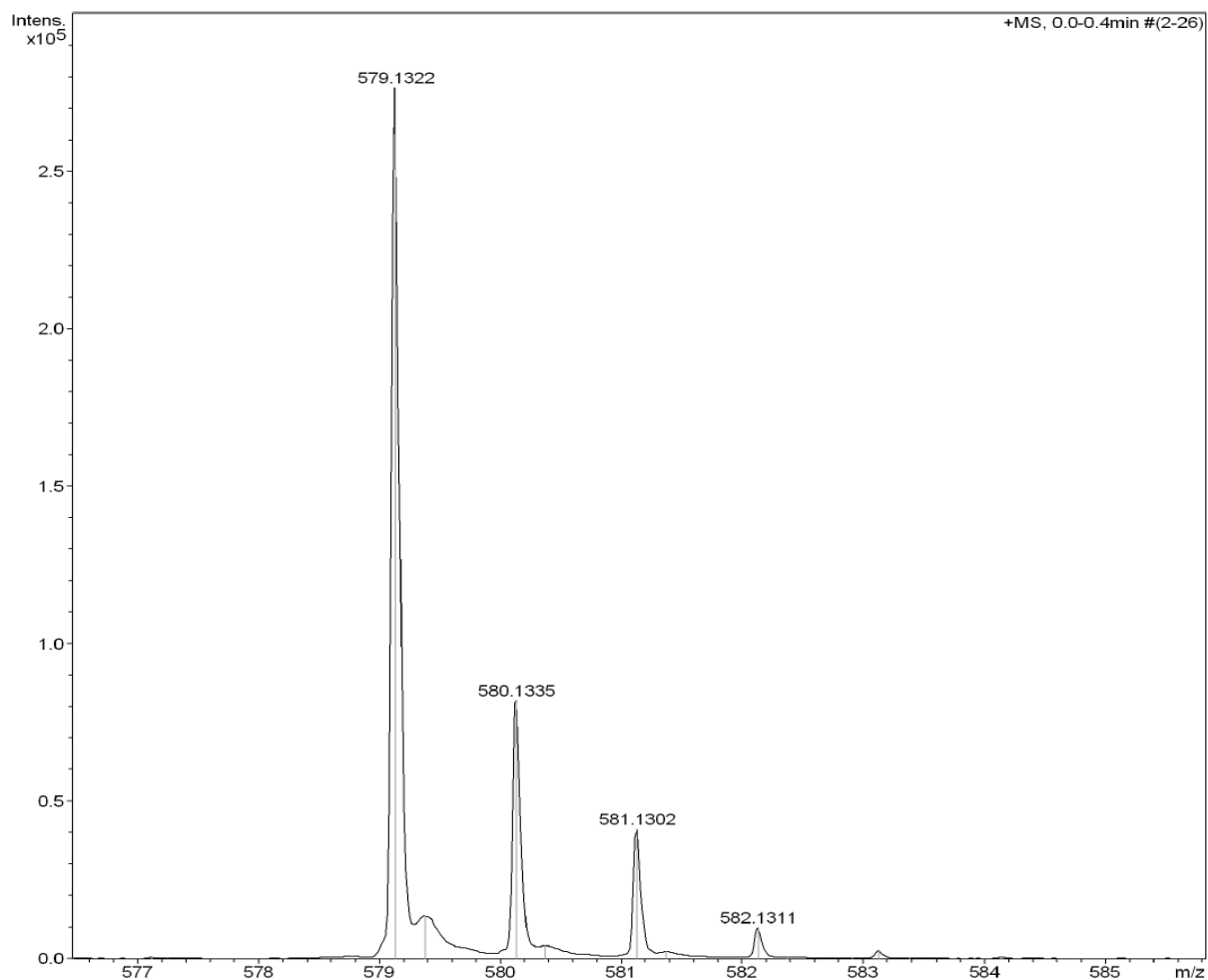
Figure S35 HRMS for compound A12
