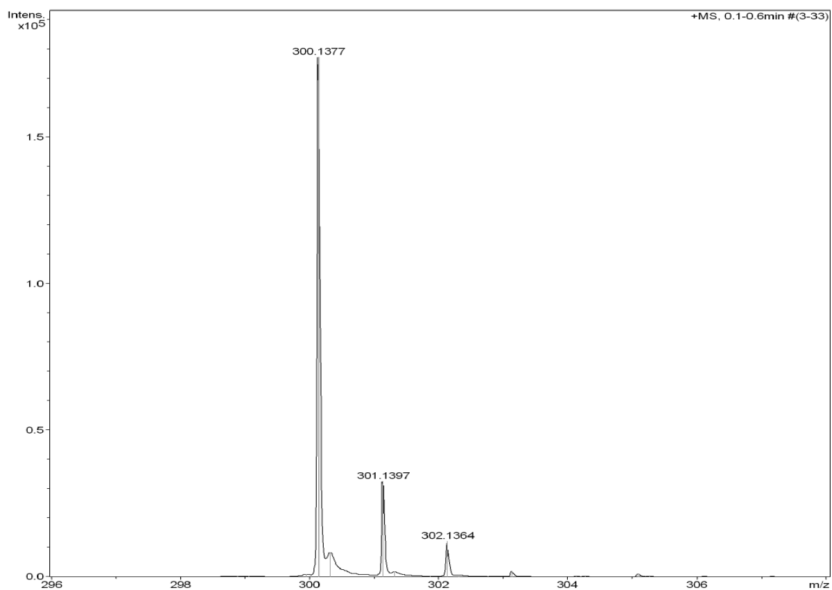
Figure S20 HRMS for compound A07
