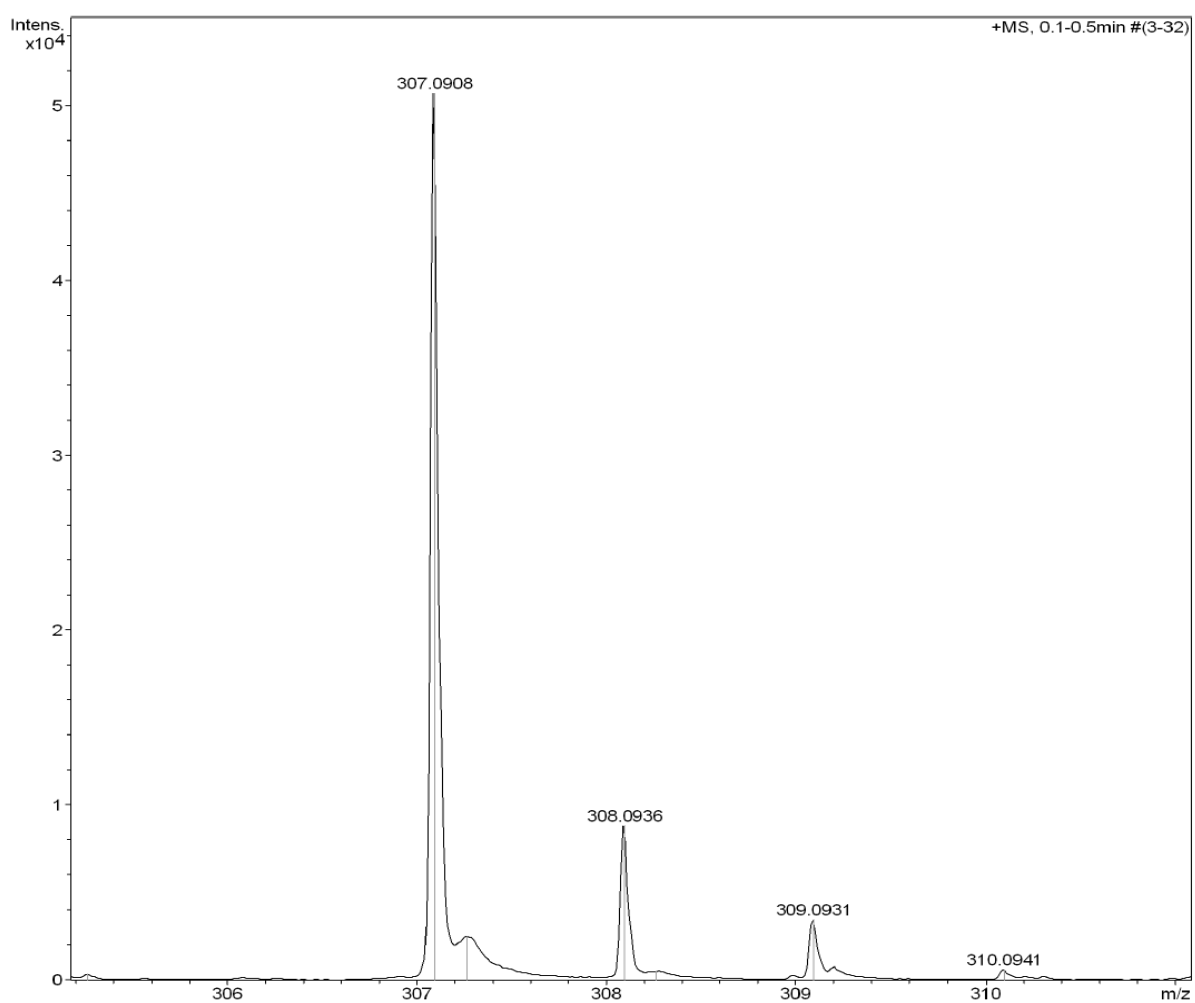
Figure S29 HRMS for compound A10
