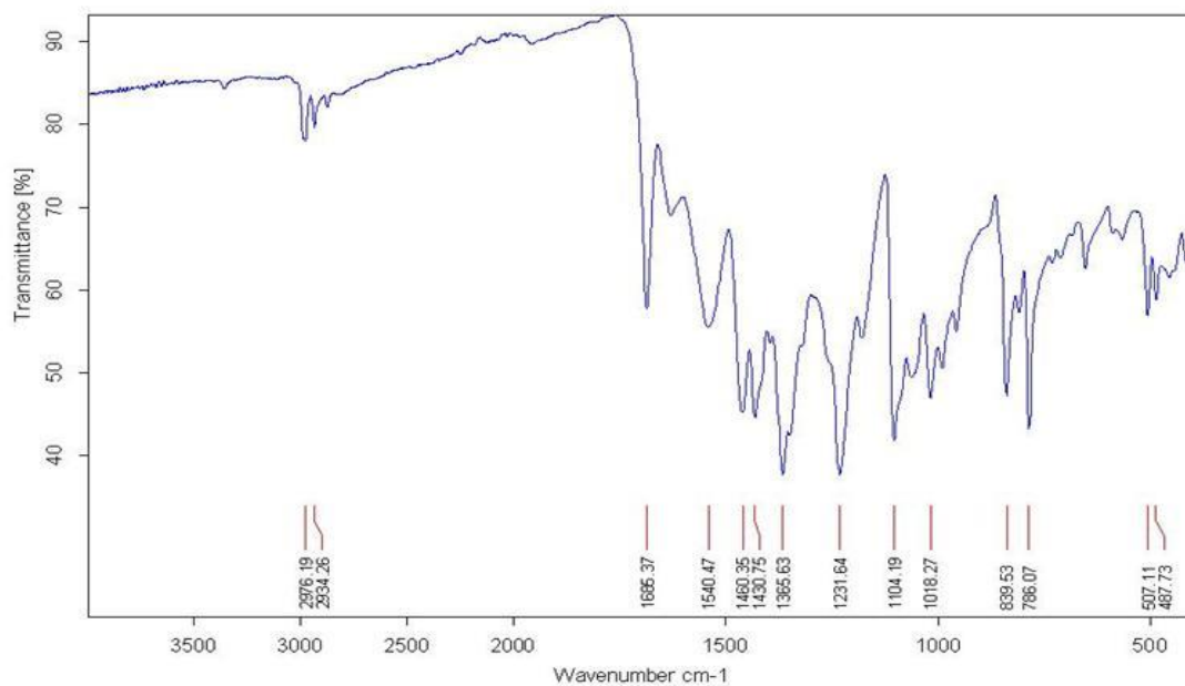
Figure S60 IR for compound A01
