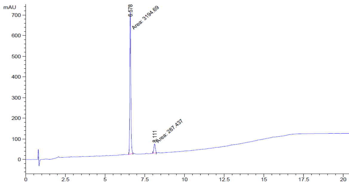
Figure S19 HPLC for compound A07
