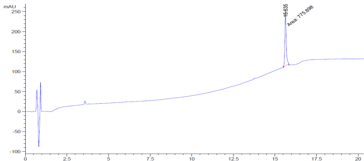
Figure S37 HPLC for compound A13
