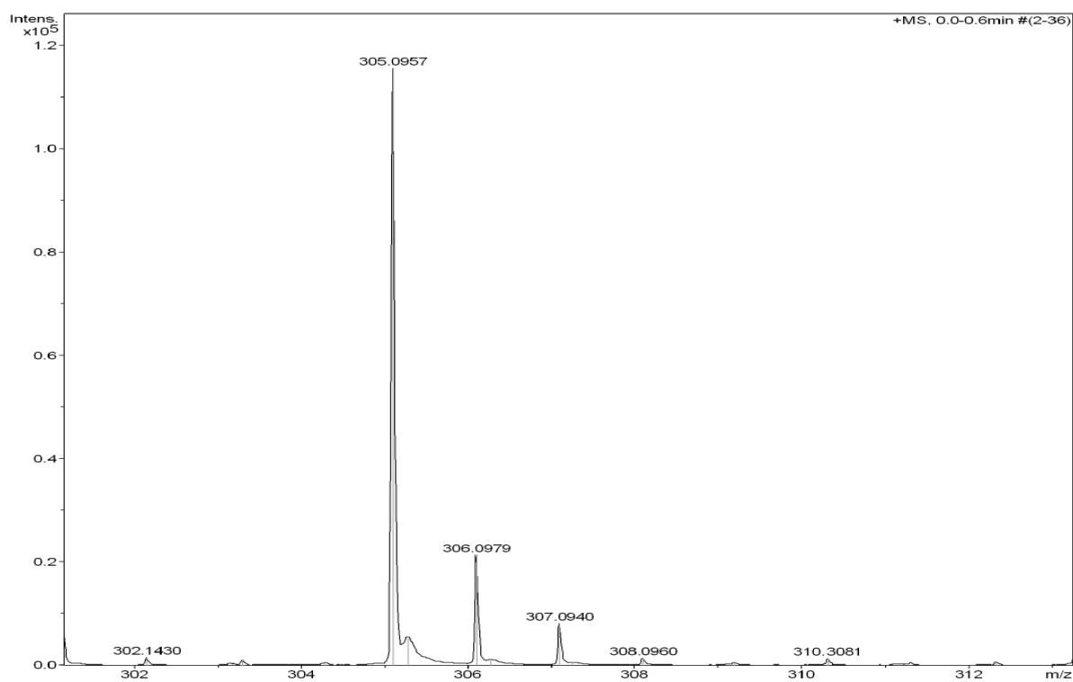
Figure S8 HRMS for compound A03
