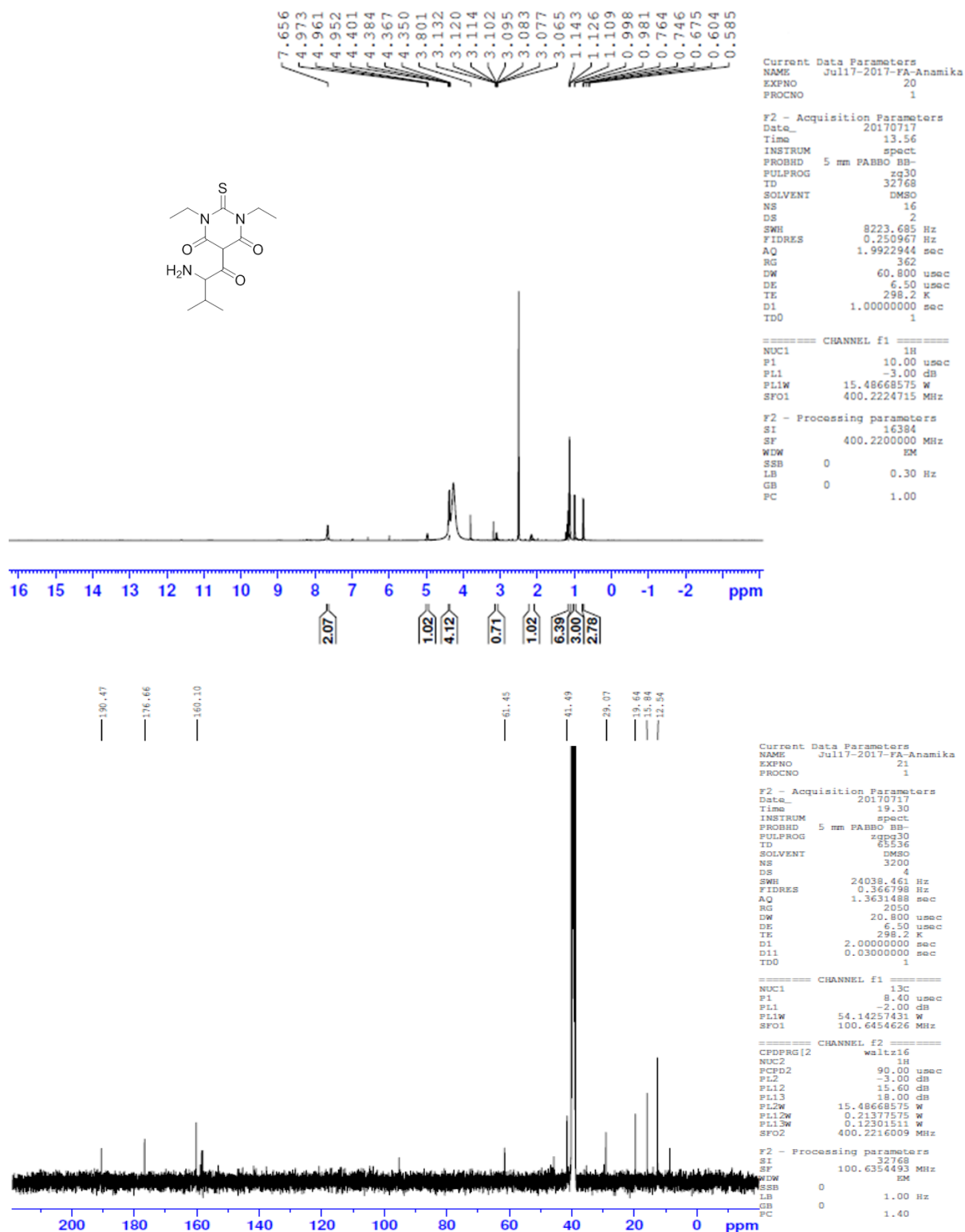
Figure S21 1 H NMR and 13 C NMR of compound A07
