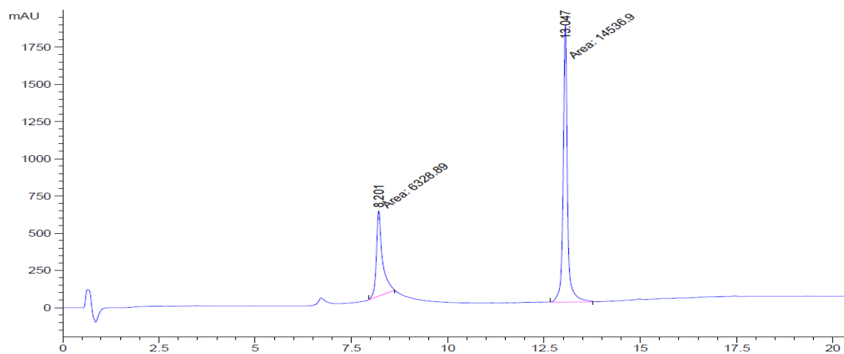
Figure S31 HPLC for compound A11
