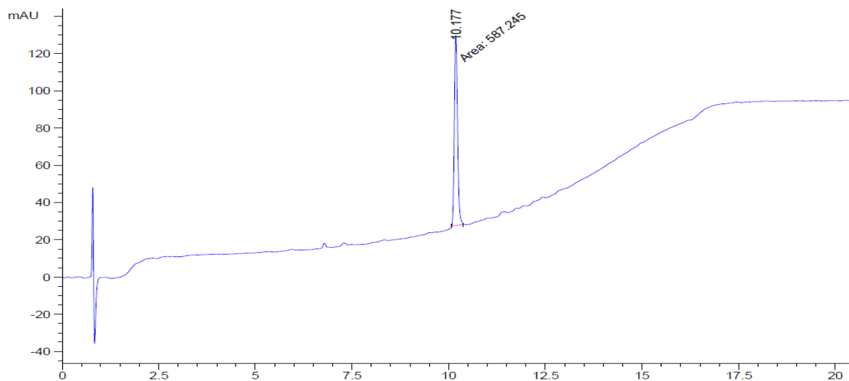
Figure S40 HPLC for compound A14
