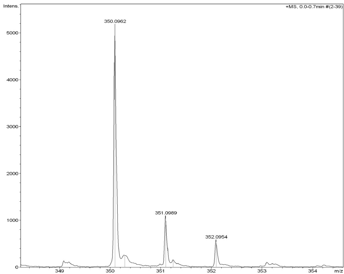
Figure S38 HRMS for compound A13
