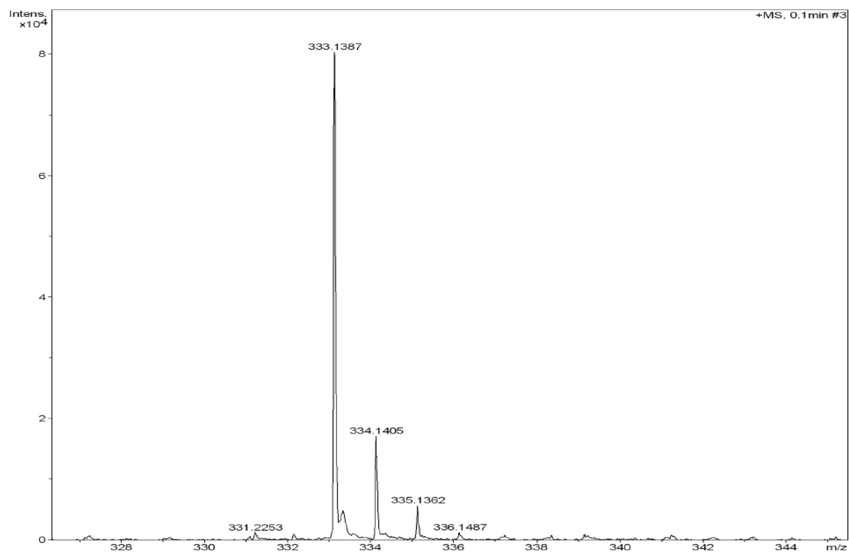
Figure S23 HRMS for compound A08
