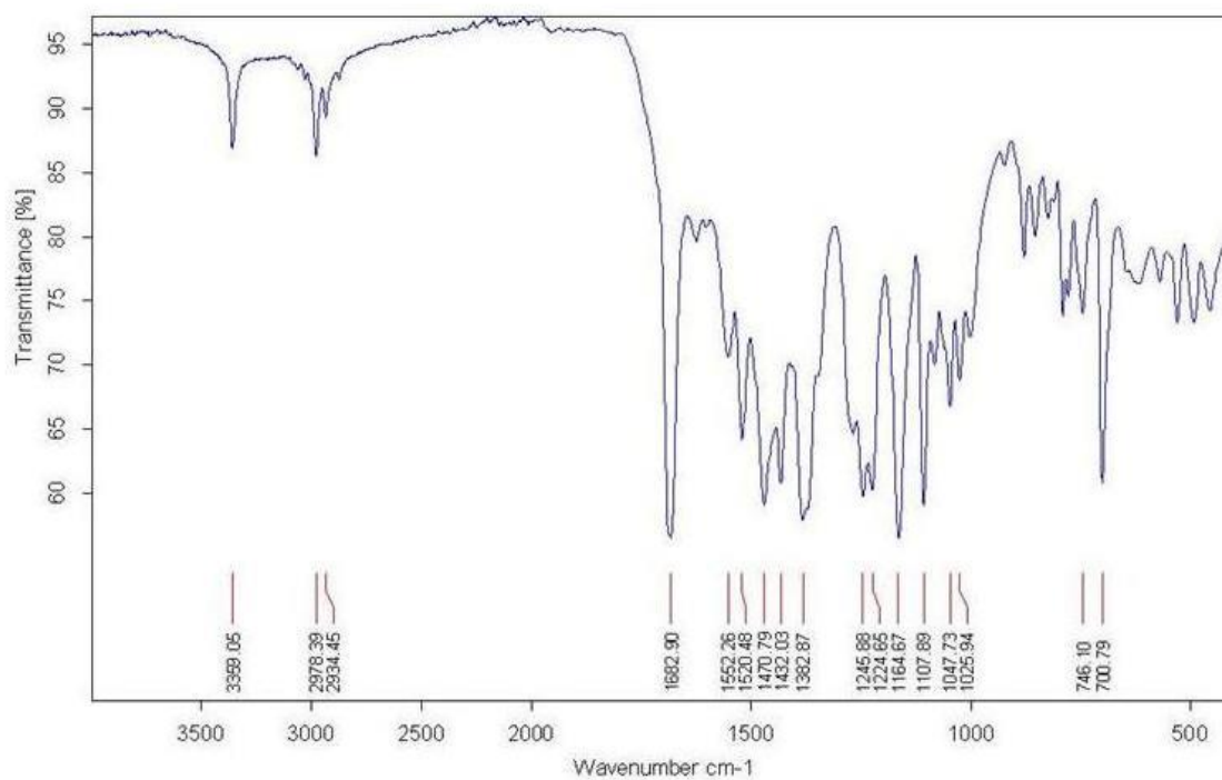
Figure S63 IR for compound A04
