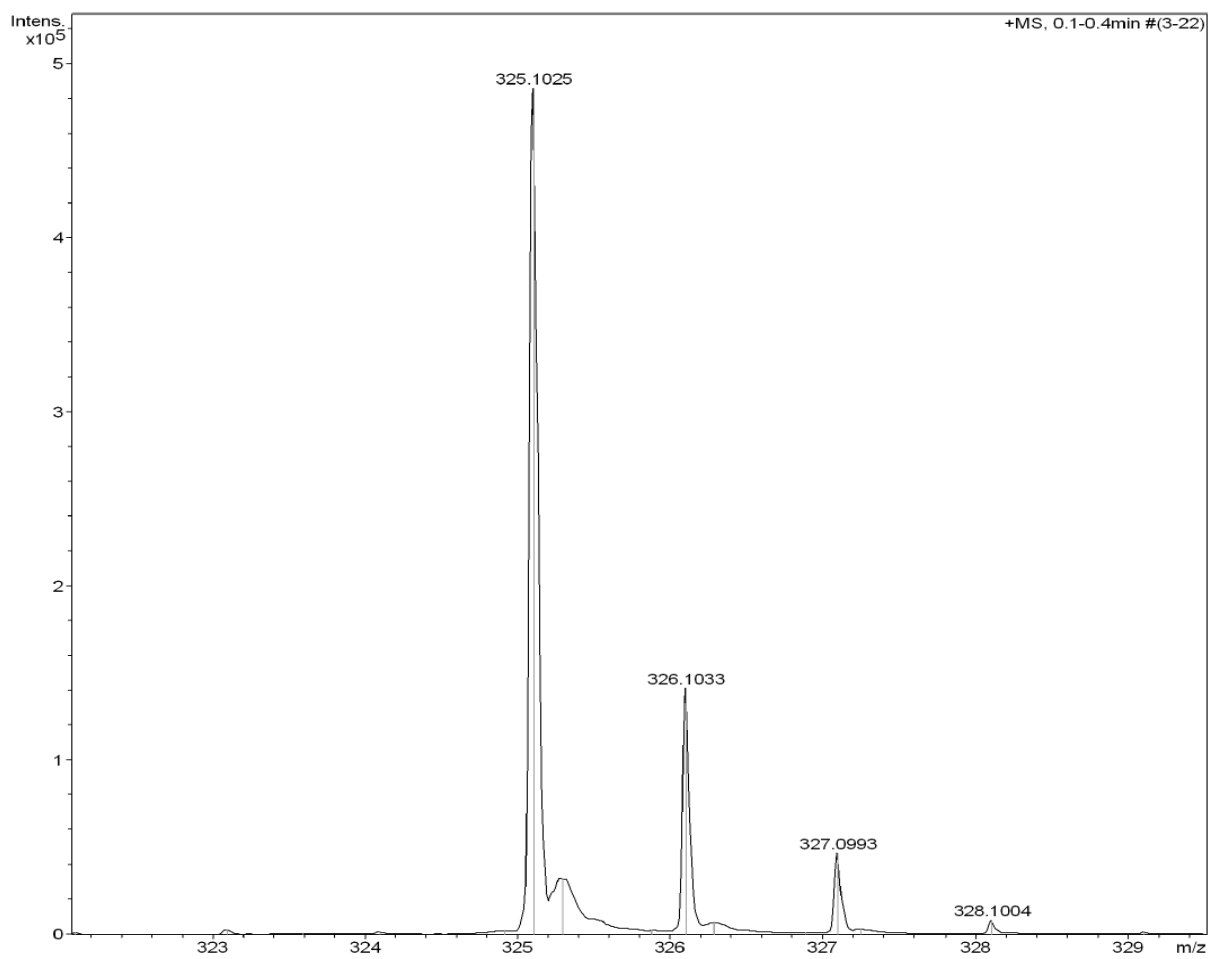
Figure S41 HRMS for compound A14
