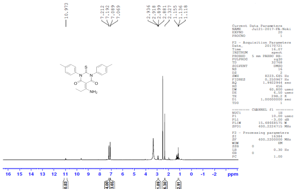
Figure S59 ^1\text{H} NMR of compound A20
