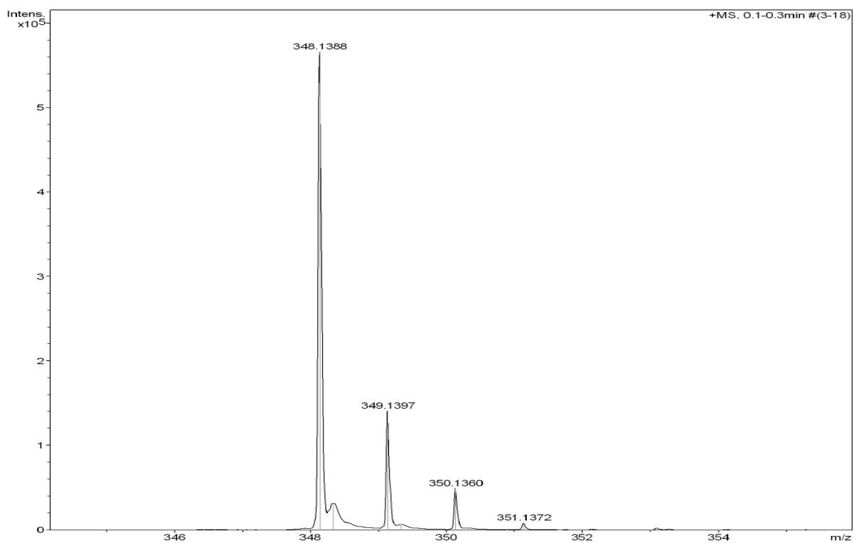
Figure S14 HRMS for compound A05
