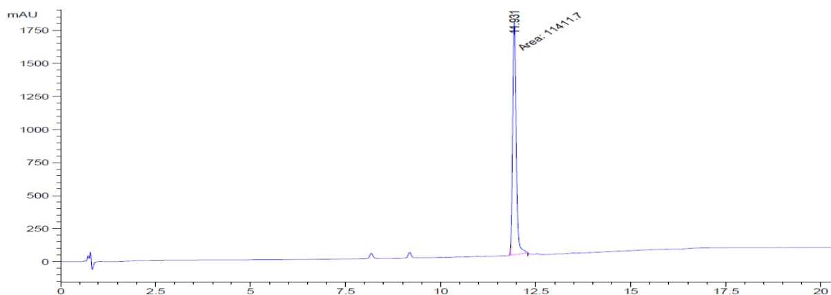
Figure S28 HPLC for compound A10
