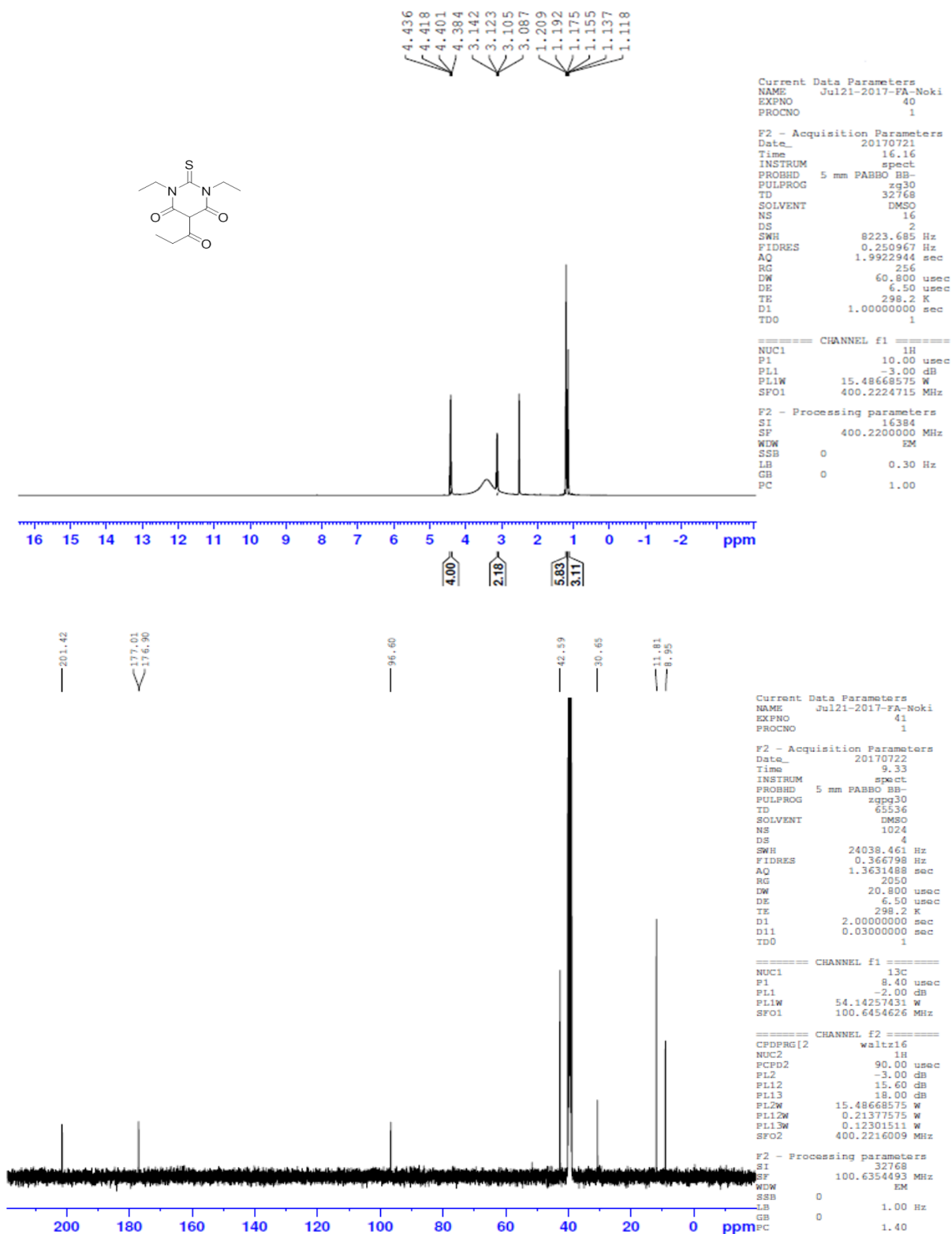
Figure S6 ^1\text{H} NMR and ^{13}\text{C} NMR of compound A02
