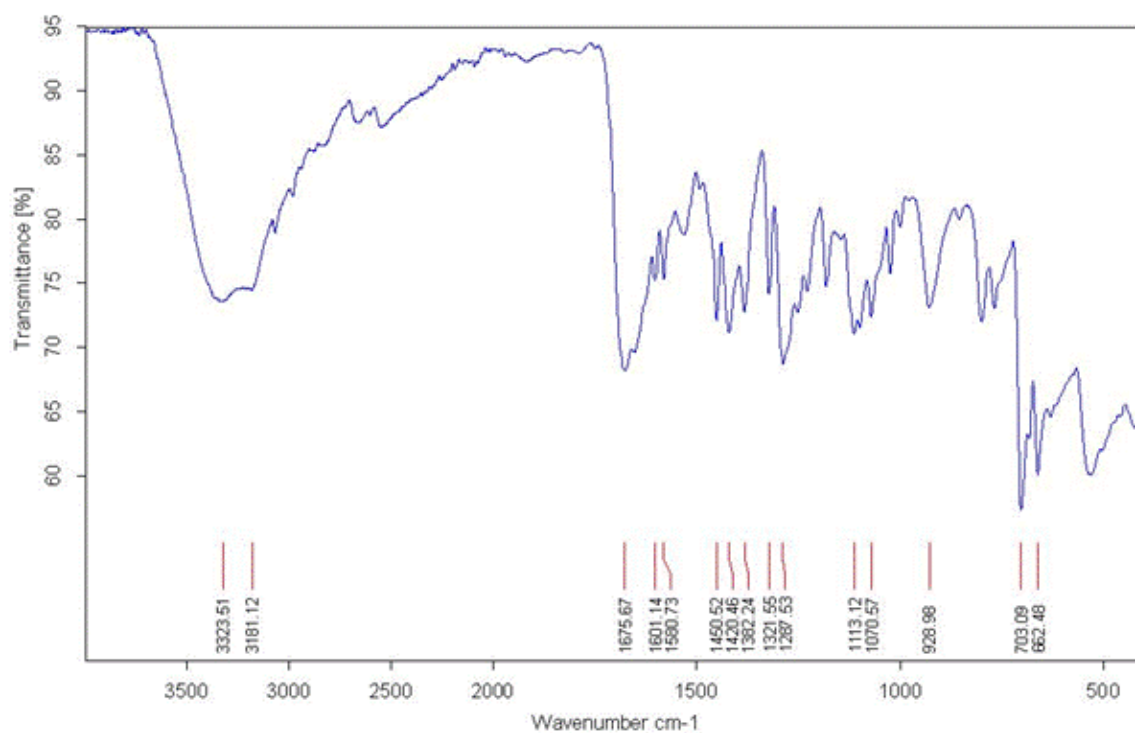
Figure S62 IR for compound A03
