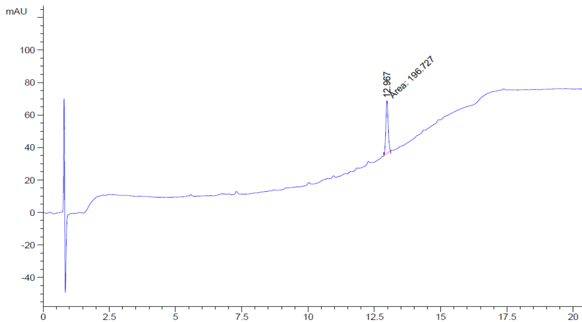
Figure S4 HPLC for compound A02
