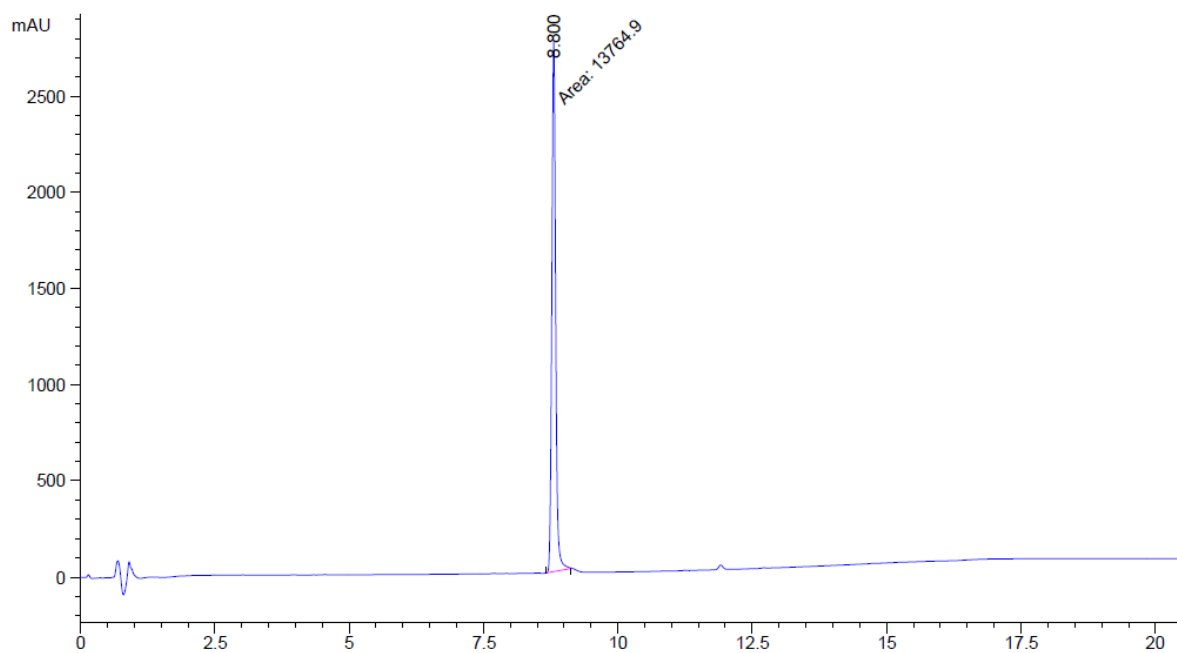
Figure S22 HPLC for compound A08
