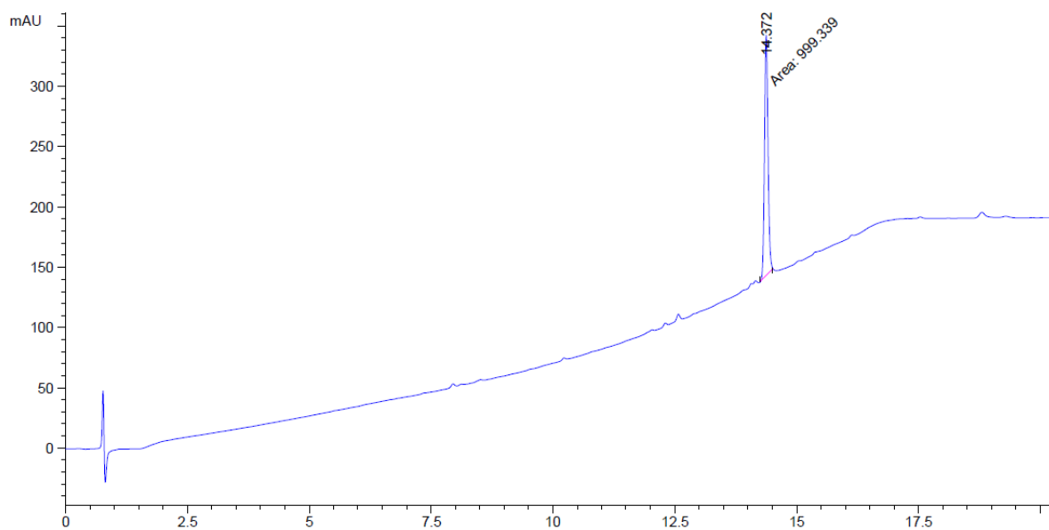
Figure S10 HPLC for compound A04
