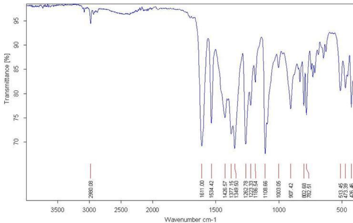
Figure S66 IR for compound A12
