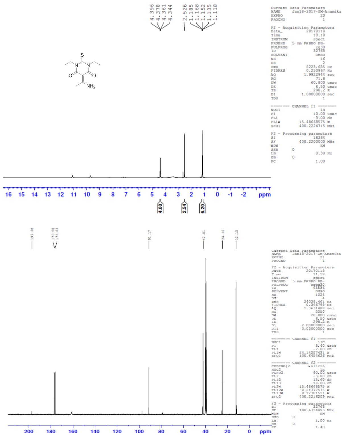
Figure S51 1 H NMR and 13 C NMR of compound A17
