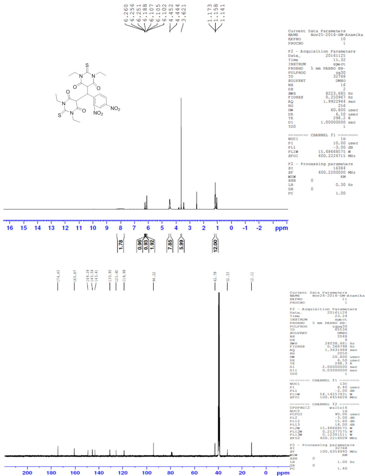
Figure S36 1 H NMR and 13 C NMR of compound A12
