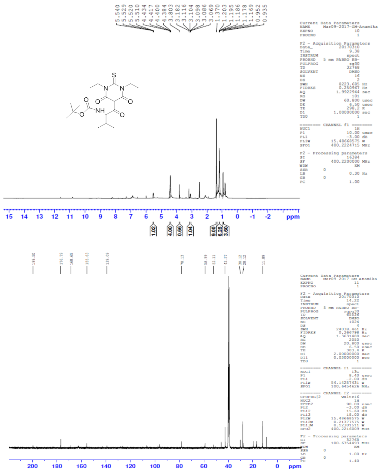
Figure S18 ^1\text{H} NMR and ^{13}\text{C} NMR of compound A06
