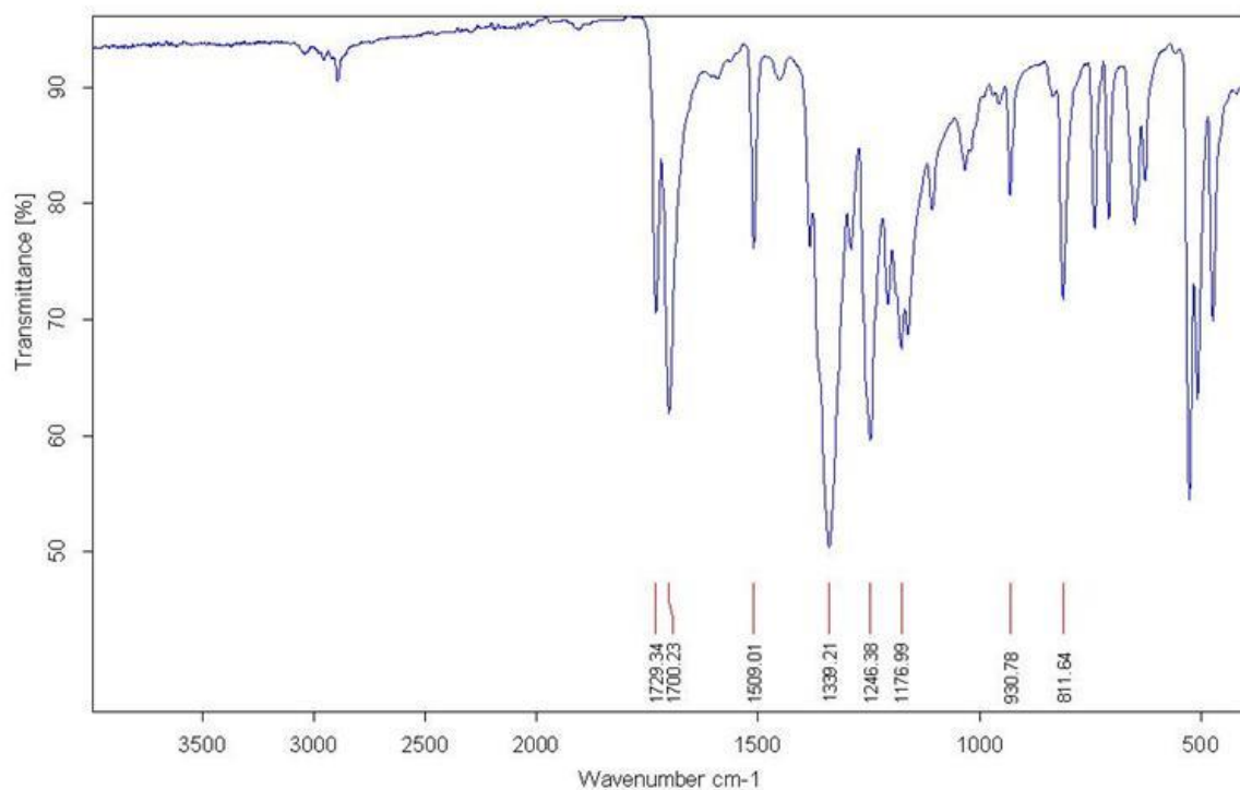
Figure S68 IR for compound A14
