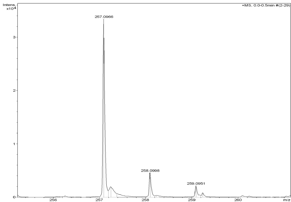
Figure S5 HRMS for compound A02
