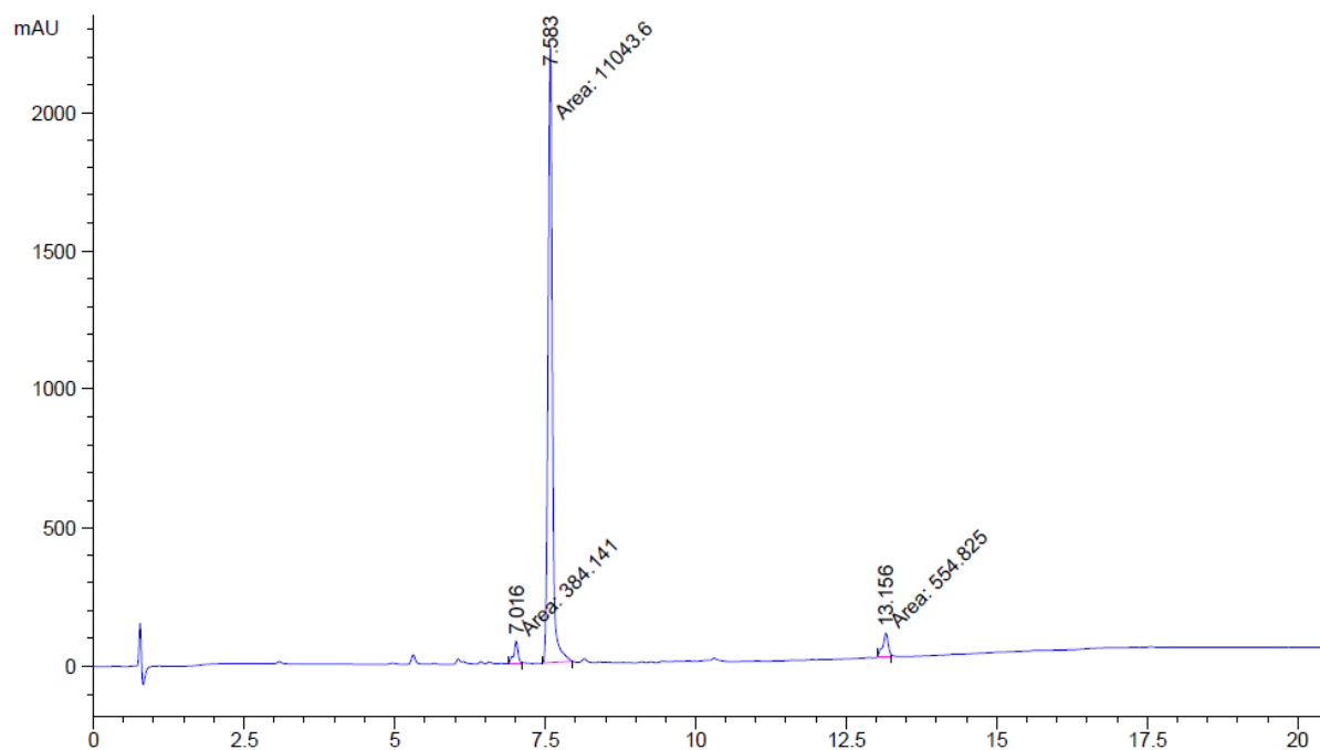
Figure S13 HPLC for compound A05
