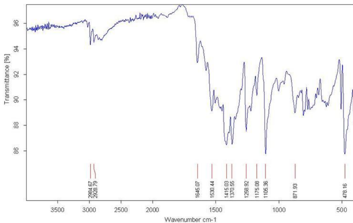
Figure S67 IR for compound A13
