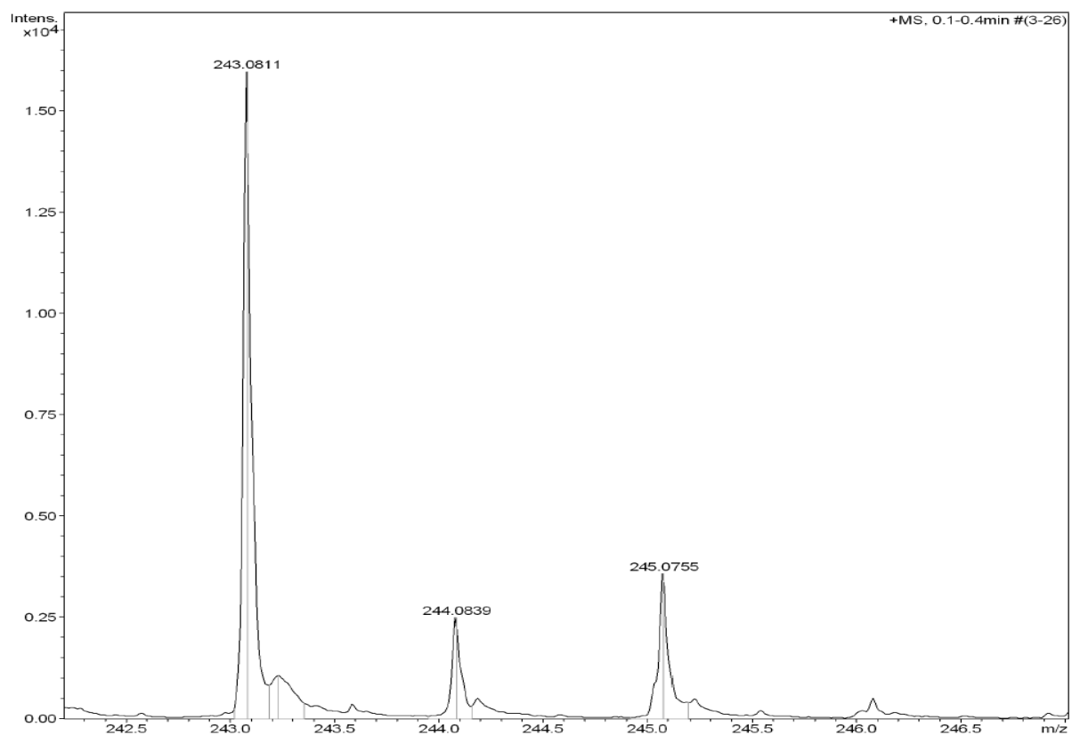
Figure S2 HRMS for compound A01
