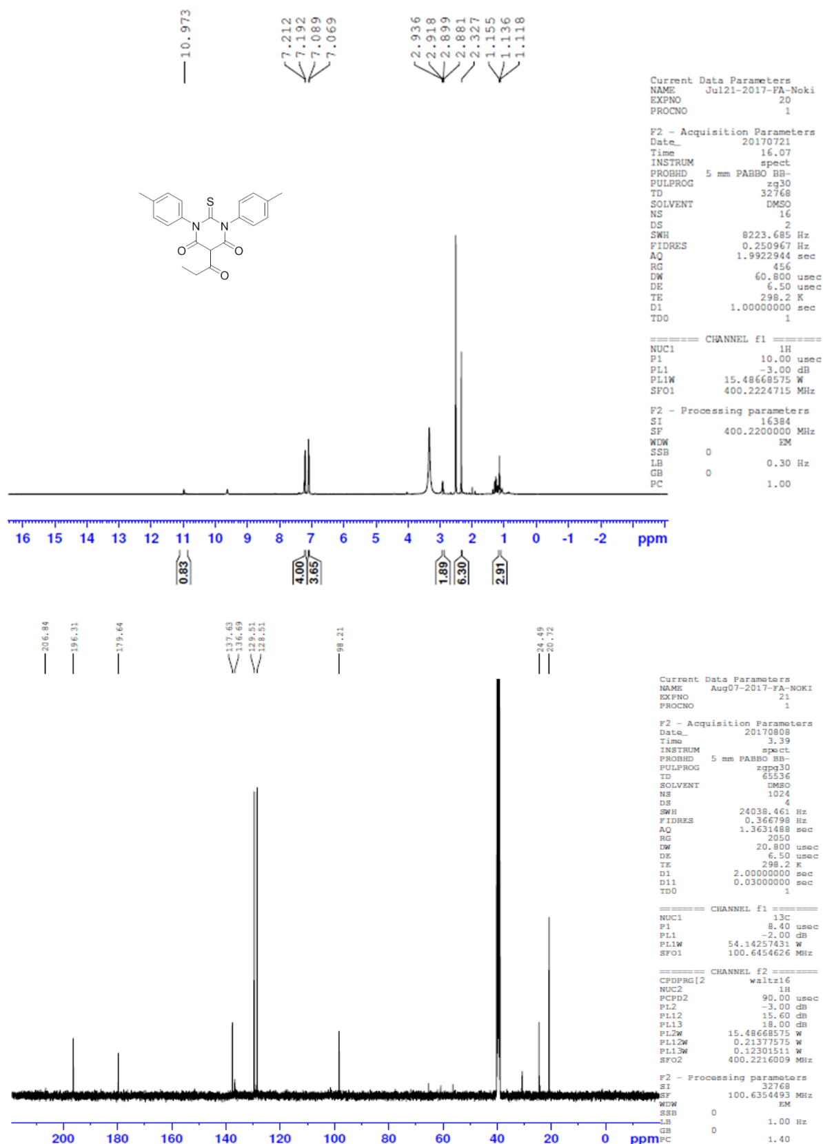
Figure S48 1 H NMR and 13 C NMR of compound A16
