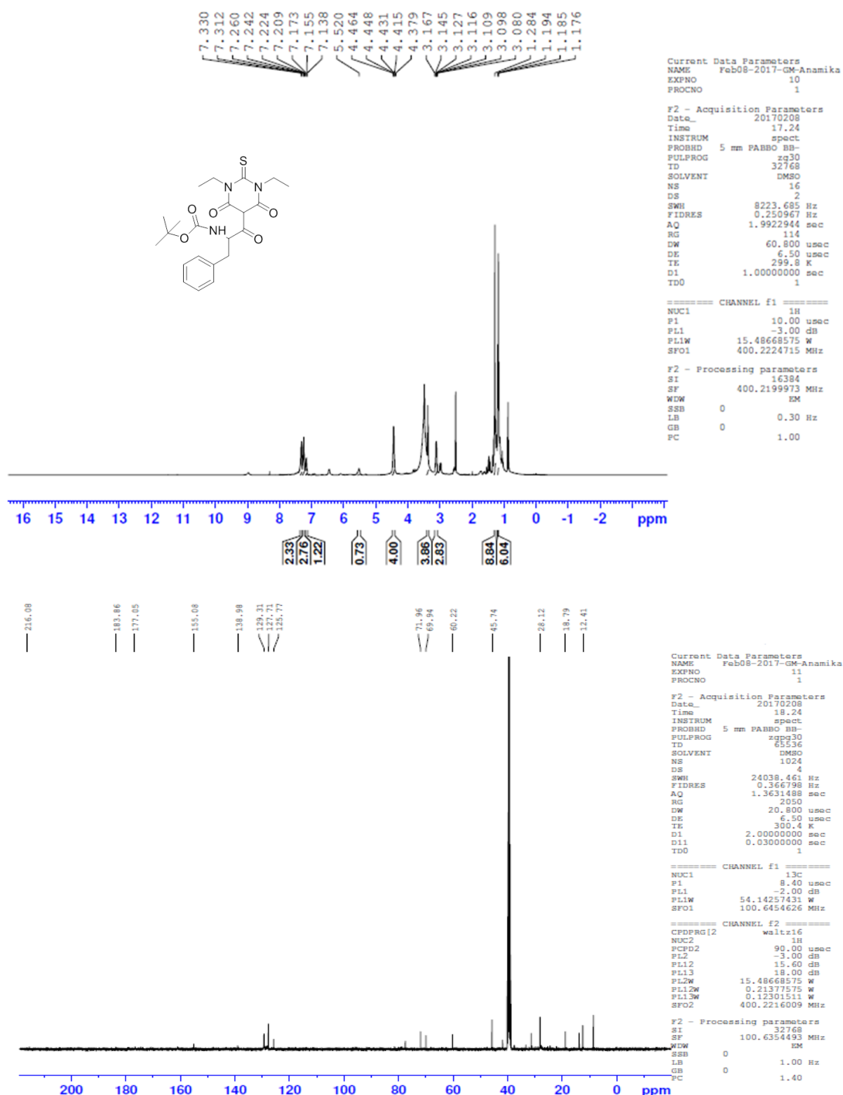
Figure S12 1 H NMR and 13 C NMR of compound A04
