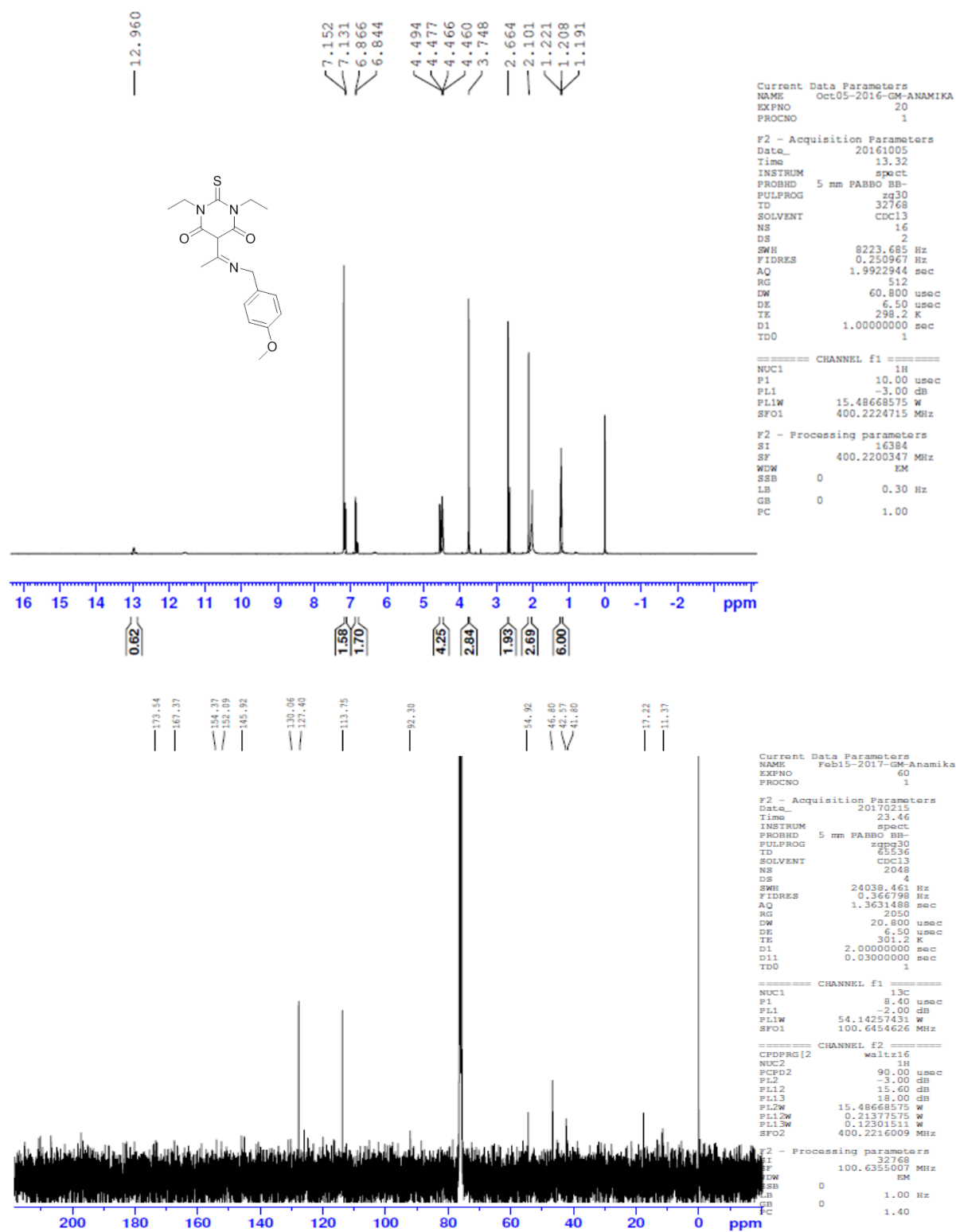
Figure S27 1 H NMR and 13 C NMR of compound A09
