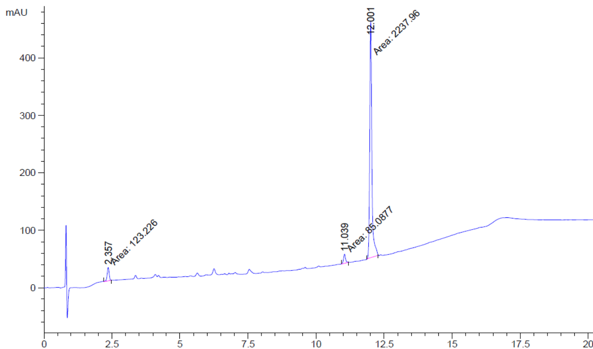
Figure S43 HPLC for compound A15
