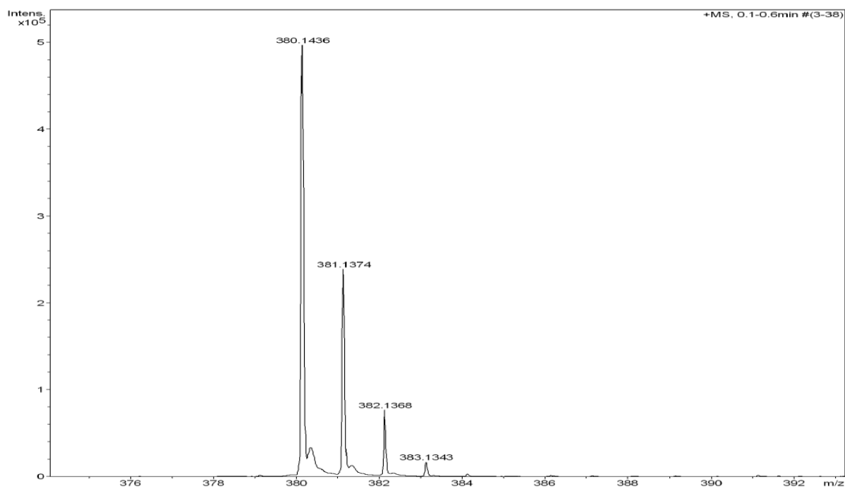
Figure S58 HRMS for compound A20
