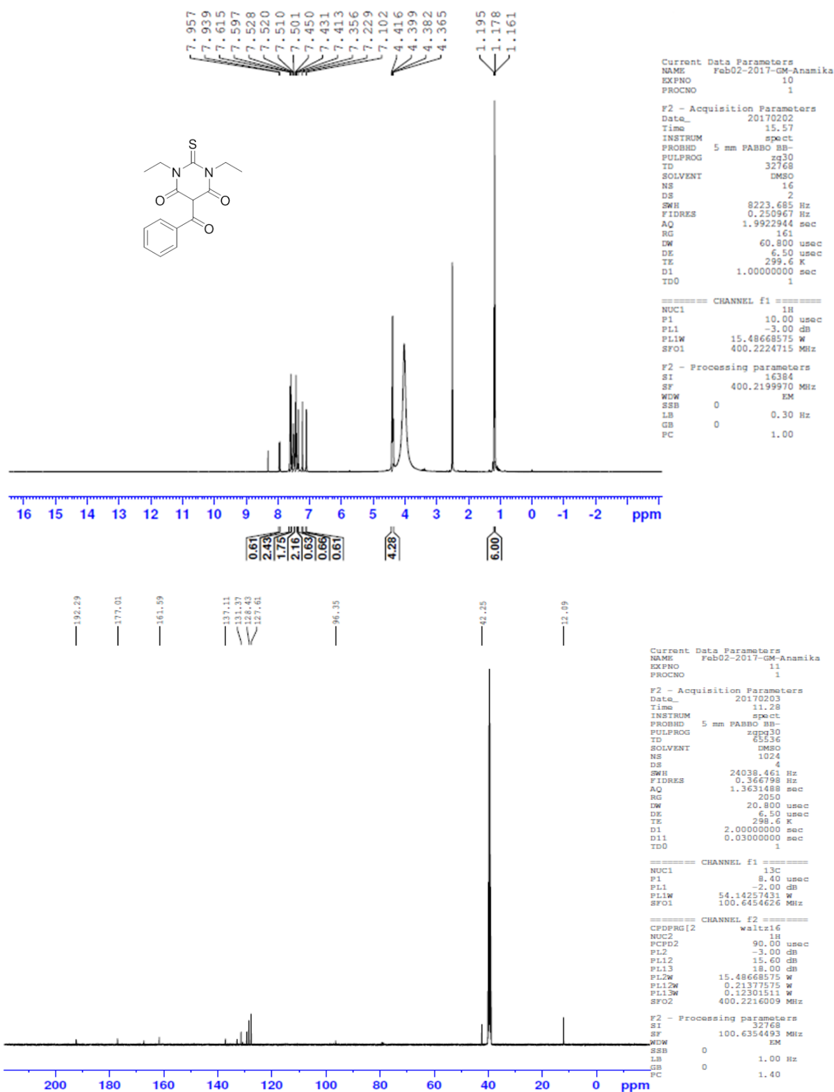
Figure S9 1 H NMR and 13 C NMR of compound A03
