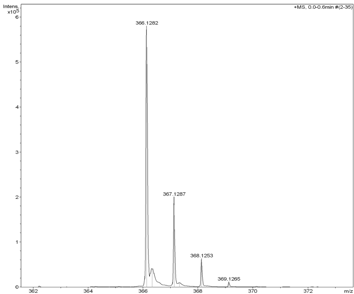
Figure S55 HRMS for compound A19
