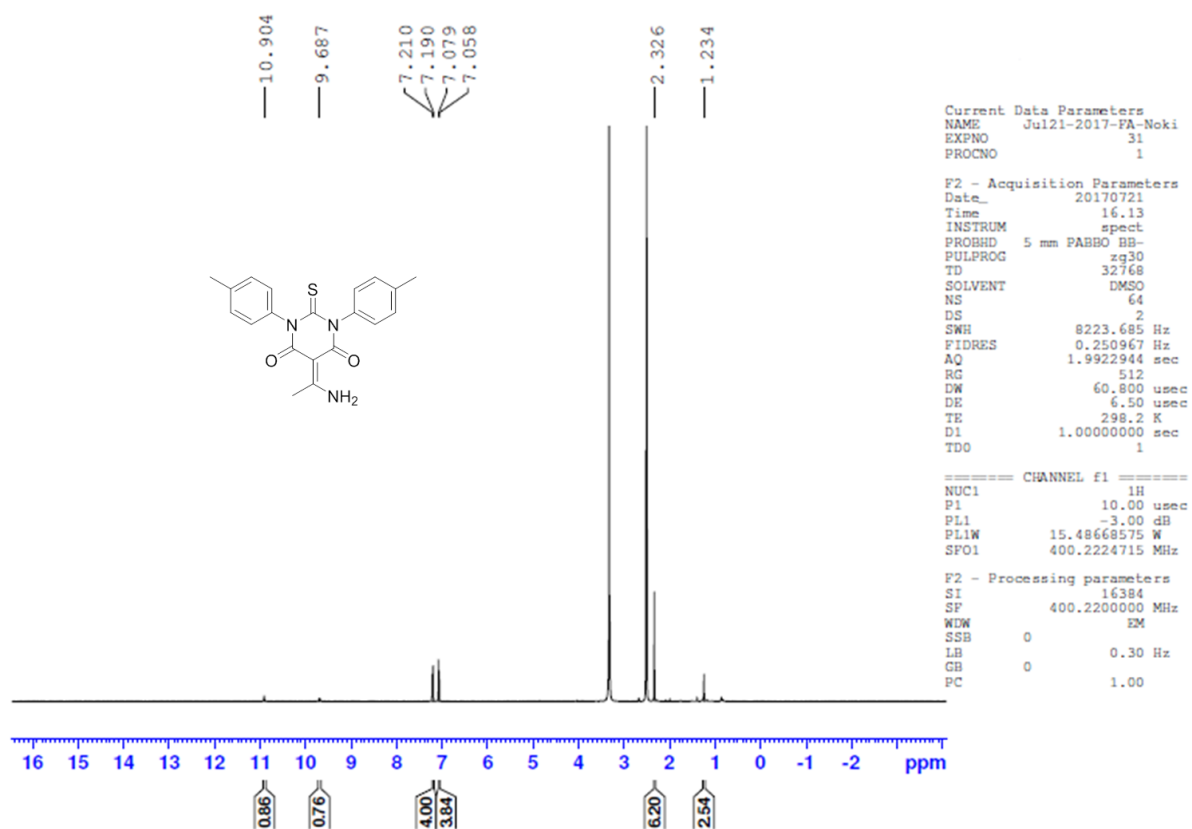
Figure S56 ^1\text{H} NMR of compound A19
