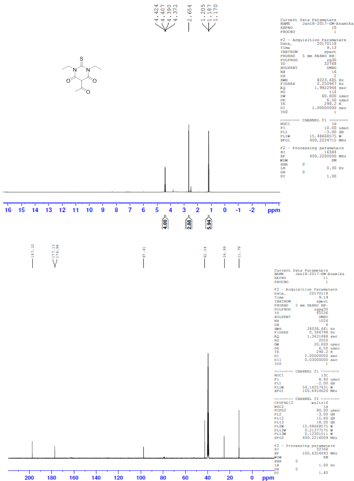
Figure S3 1 H NMR and 13 C NMR of compound A01
