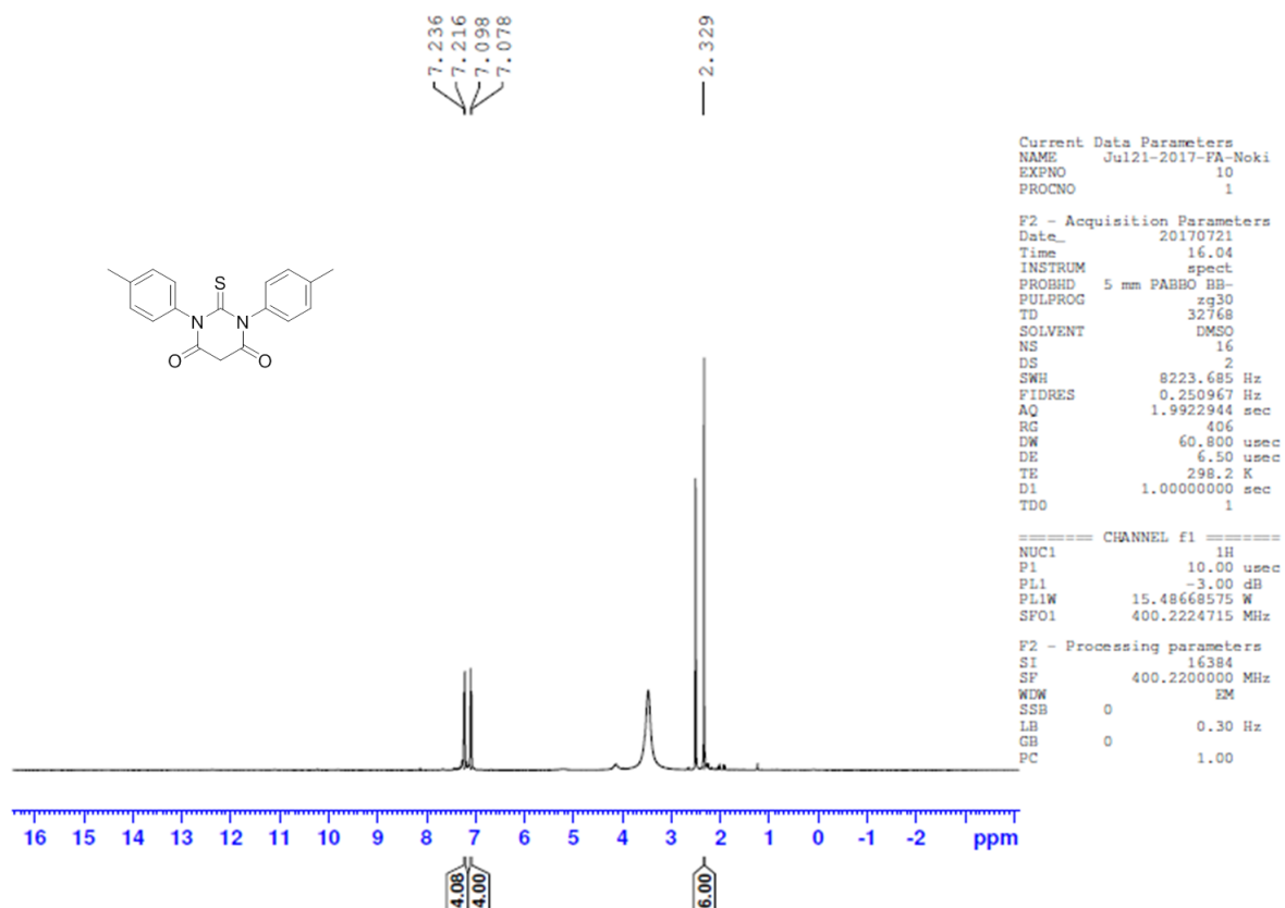
Figure S42 ^1\text{H} NMR of compound A14
