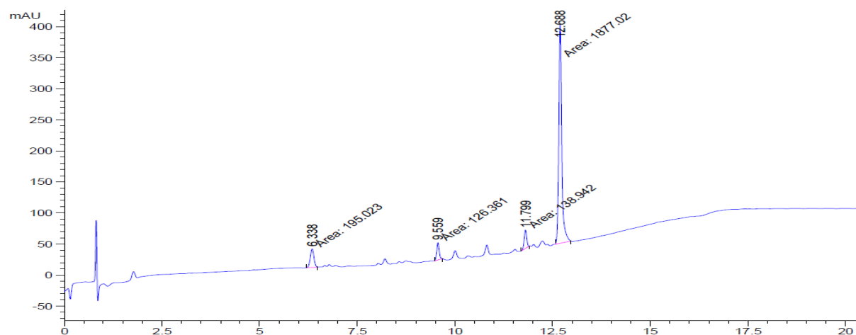
Figure S46 HPLC for compound A16
