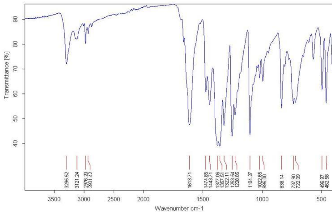
Figure S69 IR for compound A17
