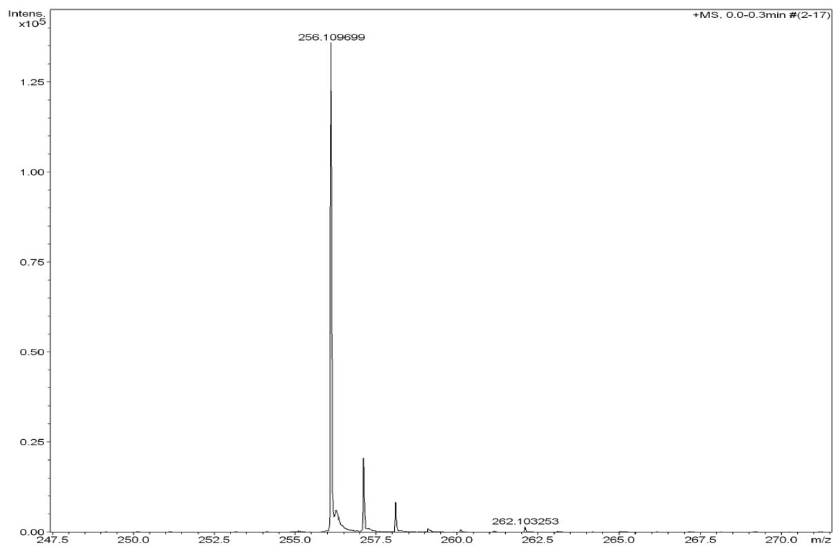
Figure S53 HRMS for compound A18
