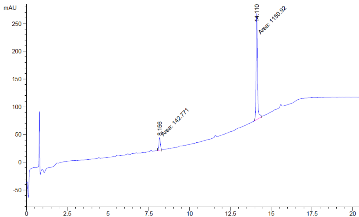
Figure S16 HPLC for compound A06
