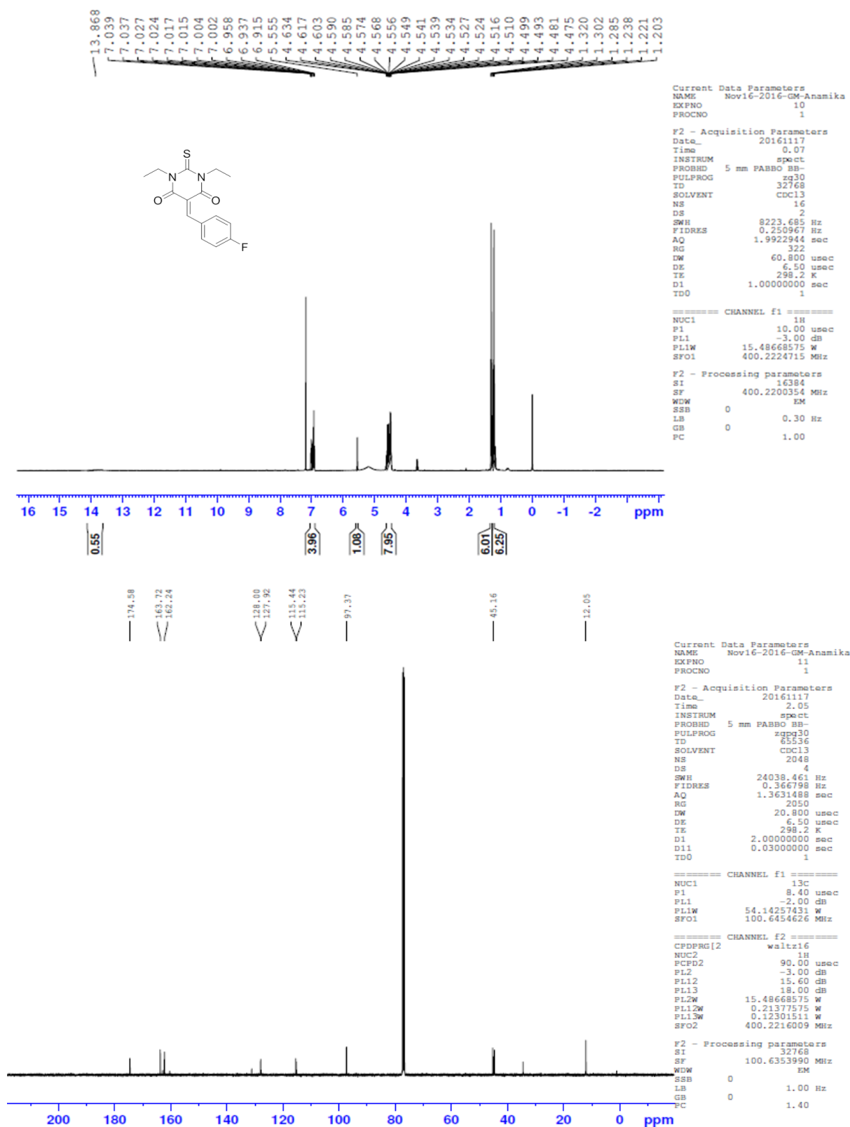
Figure S30 1 H NMR and 13 C NMR of compound A10
