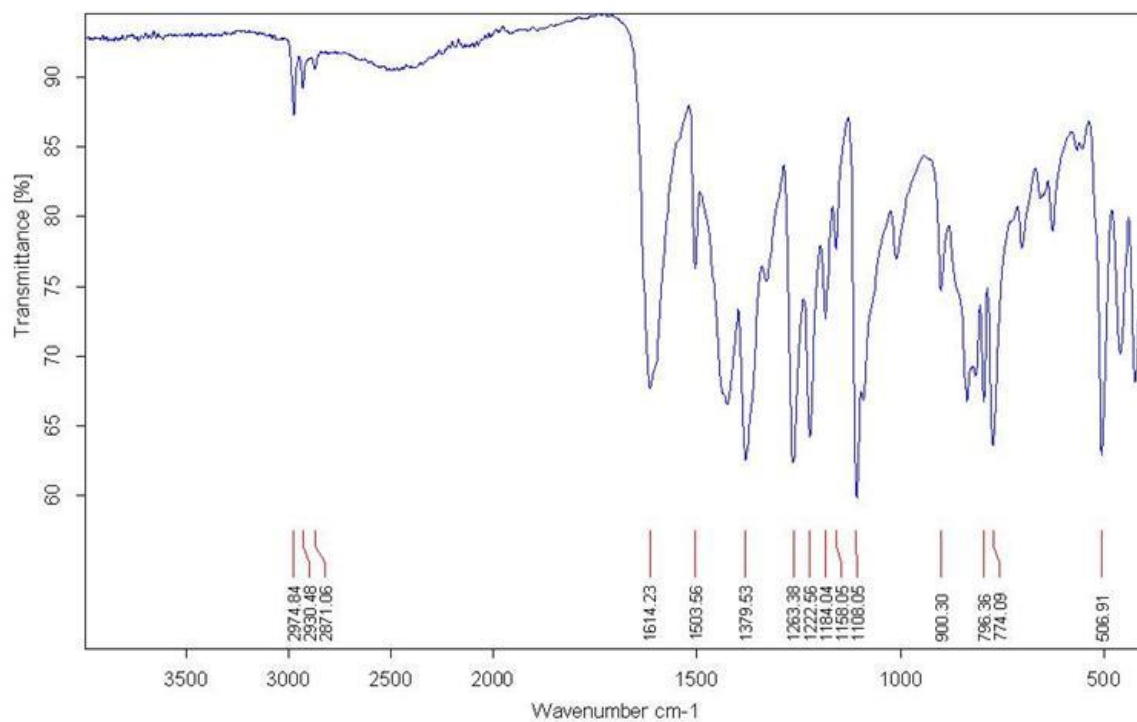
Figure S65 IR for compound A10
