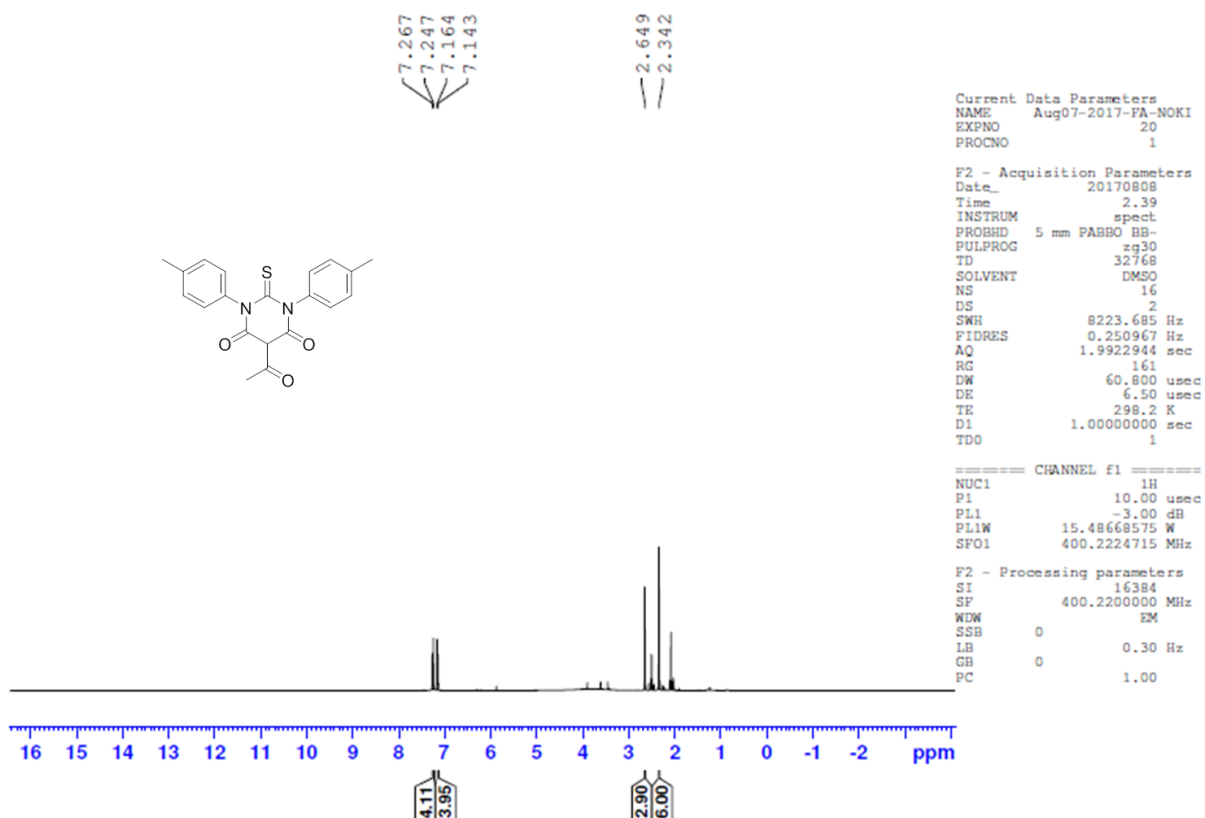
Figure S45 1 H NMR of compound A15
