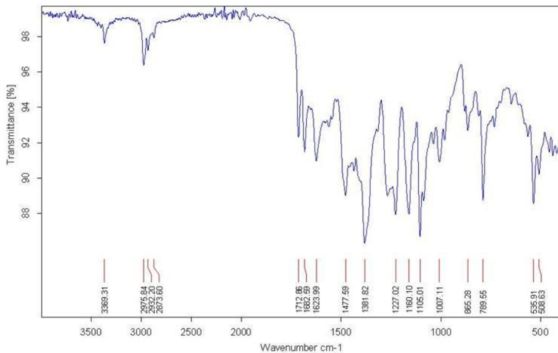
Figure S64 IR for compound A06
