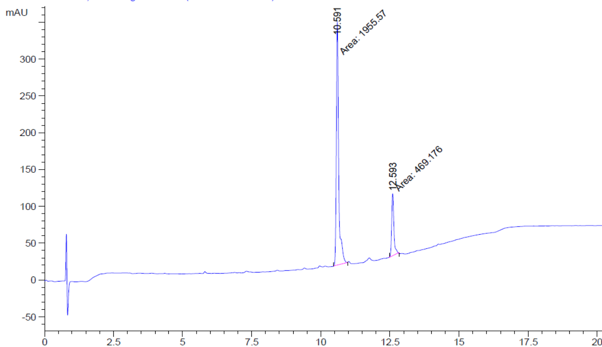
Figure S57 HPLC for compound A20
