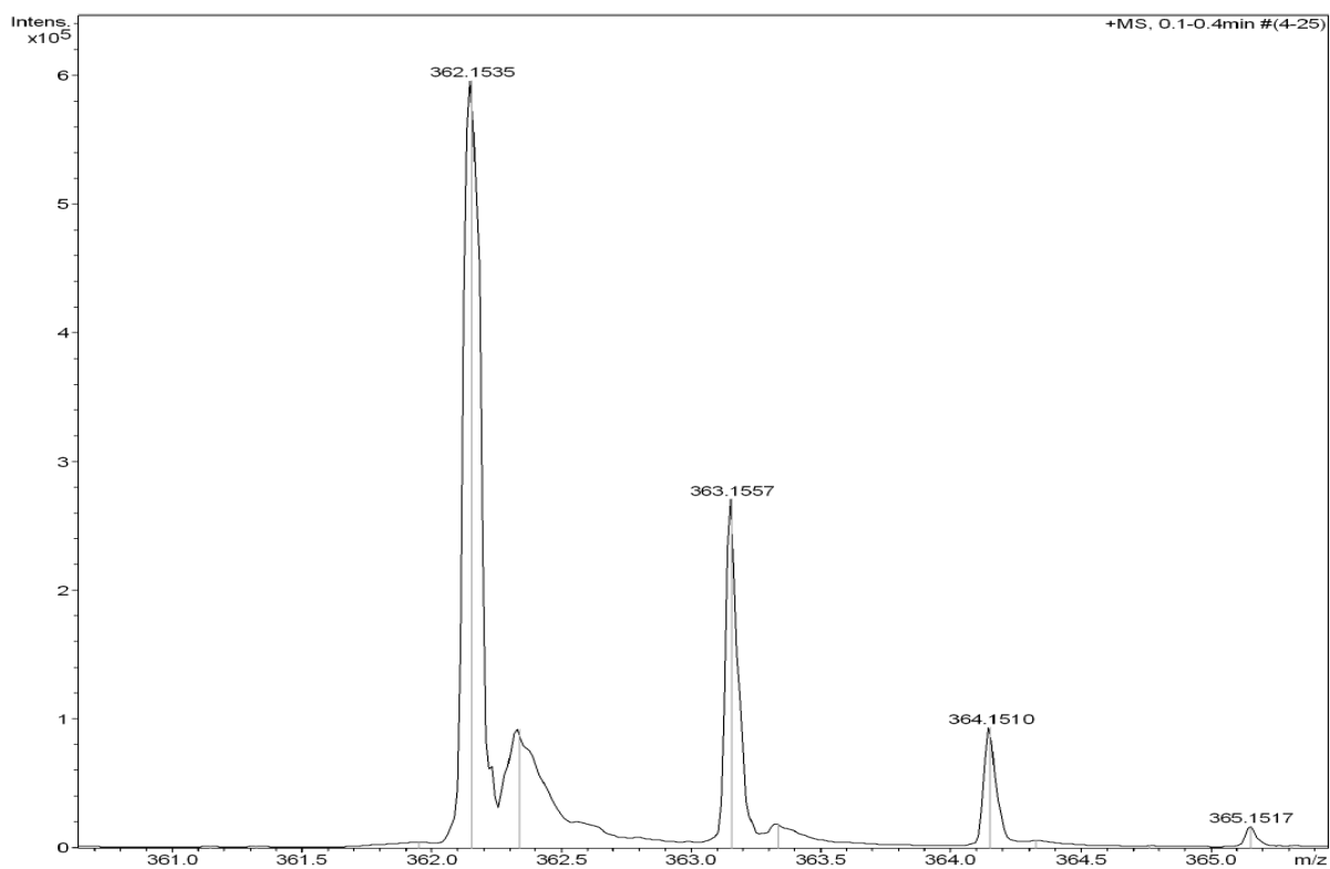
Figure S26 HRMS for compound A09
