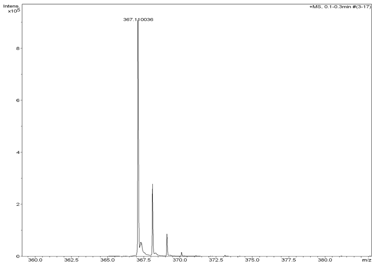
Figure S44 HRMS for compound A15
