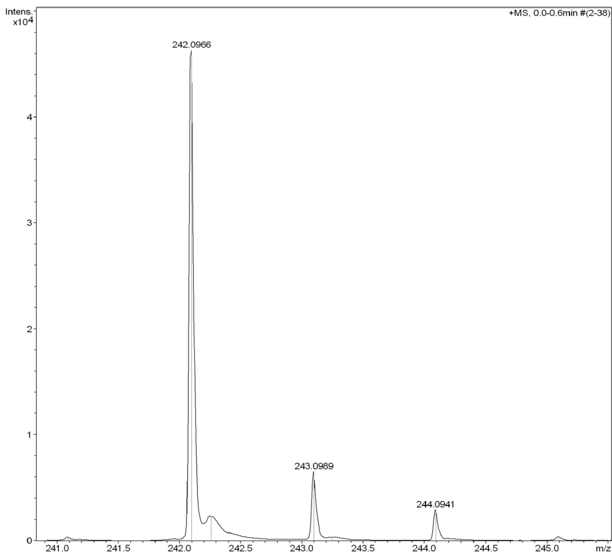
Figure S50 HRMS for compound A17
