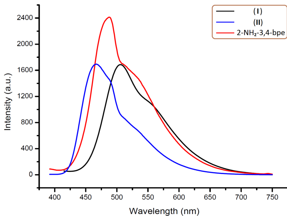
Figure S3 Emission spectra of the free 2-NH 2 -3,4-bpe ligand and complexes (I) and (II) in the solid state at room temperature.
