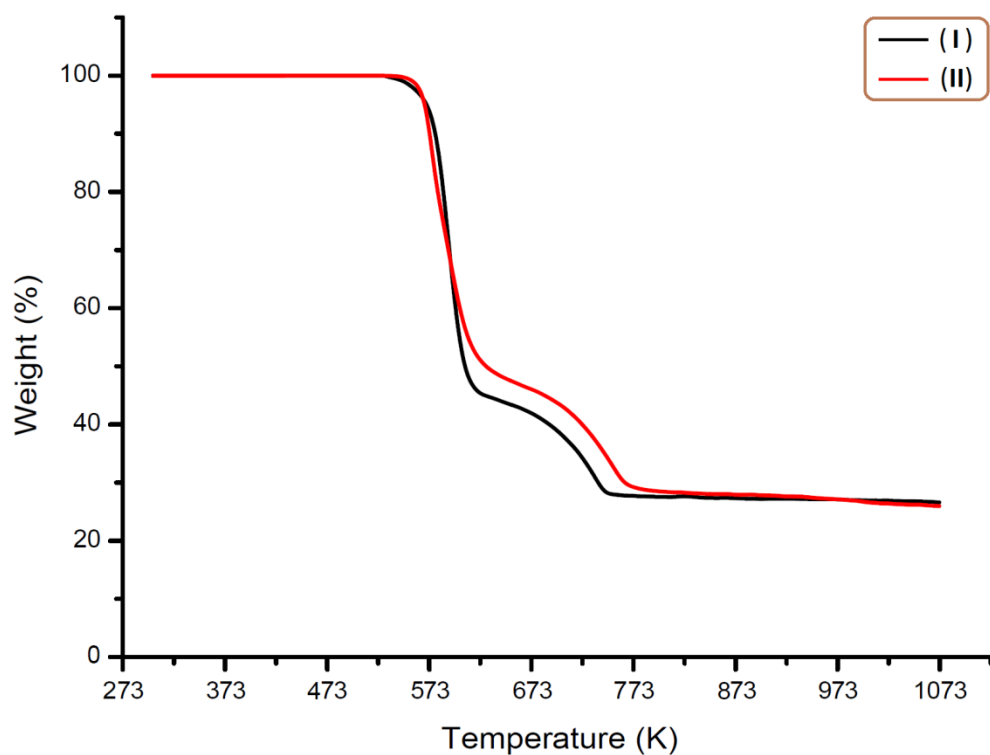
Figure S2 The TGA curves for (I) and (II).
