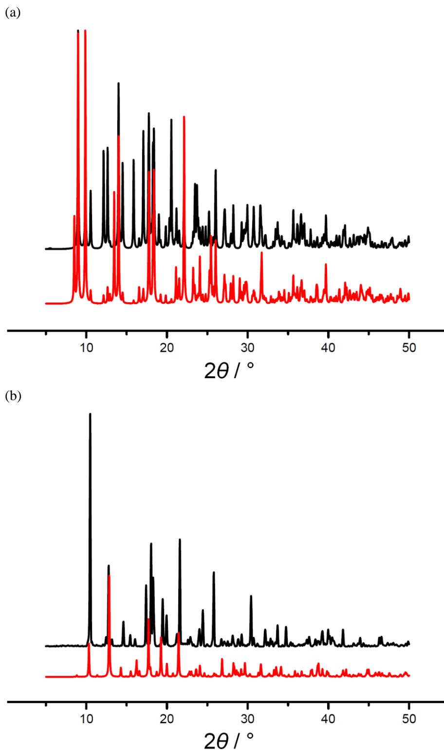
Figure S1 (a) Experimental (black) and simulated (red) PXRD patterns of (I). (b) Experimental (black) and simulated (red) PXRD patterns of (II).
