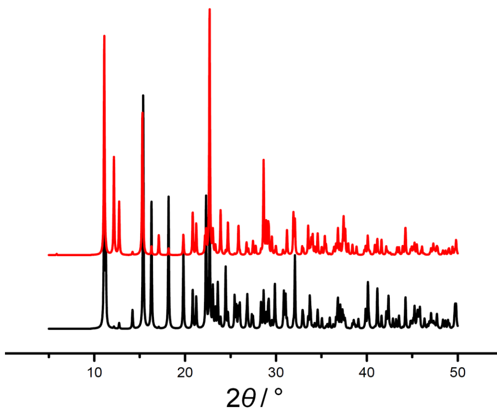
Figure S1 Experimental (red) and simulated (black) PXRD patterns of (I).
