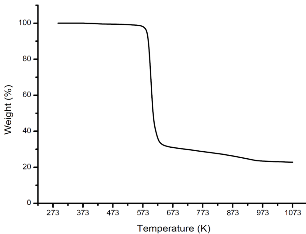
Figure S2 The TGA curve for (I).
