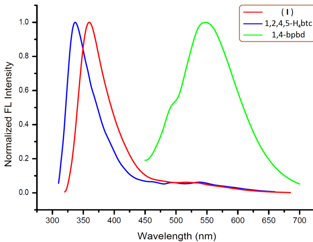
Figure S3 Normalized fluorescence spectra of (I), 1,2,4,5-H 4 btc and 1,4-bpbd in the solid state at ambient temperature.
