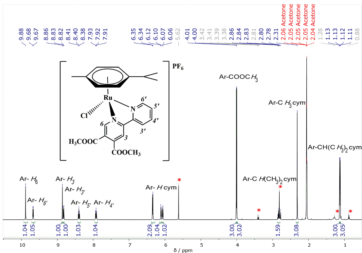
Figure S1: ^1\text{H} NMR spectrum of the studied complex with the proton assignment for the studied complex. With * are marked the protons belonging to the solvent residue (dichloromethane, diethylether, water and hexane).
