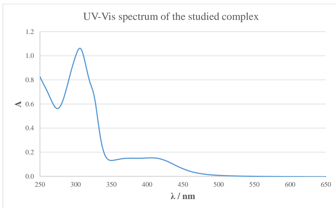
Figure S2: Experimental UV-Vis spectra of the studied complex in methanol with concentration of 60 \mu\text{M} .
