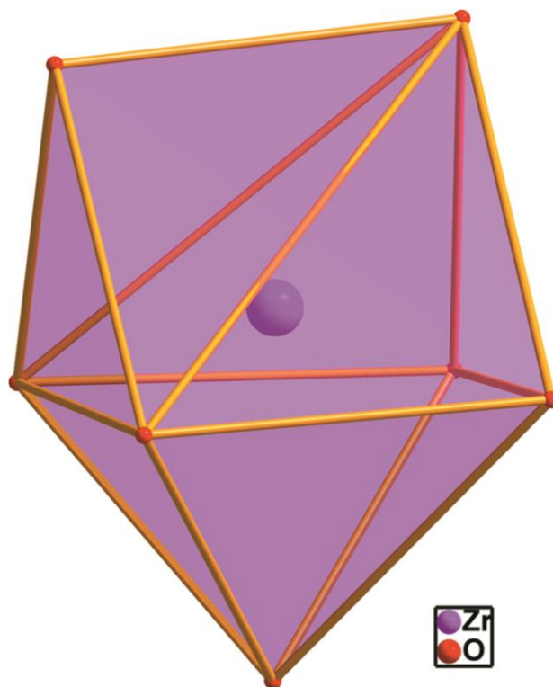
Fig. S1. Capped octahedral geometry of the Zr^{4+} cation in 1 .
