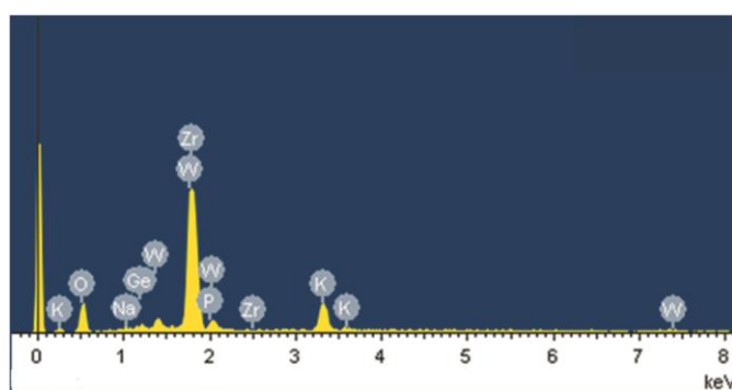
Fig. S6. The energy-dispersive X-ray spectroscopy (EDS) of 1 .
