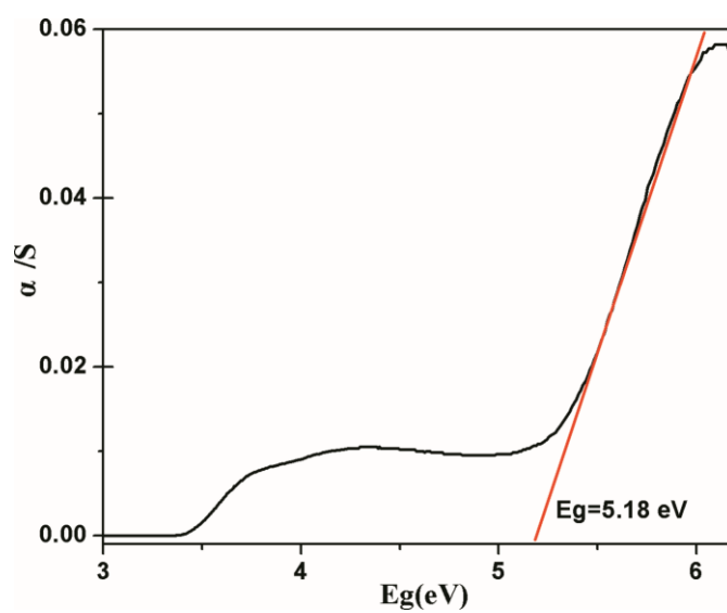
Fig. S5. UV-Vis plots of Kunelka-Munk function versus energy E (eV) of 1 .
