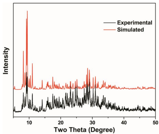
Fig. S3. Comparison of the simulated and experimental PXRD patterns of 1 .
