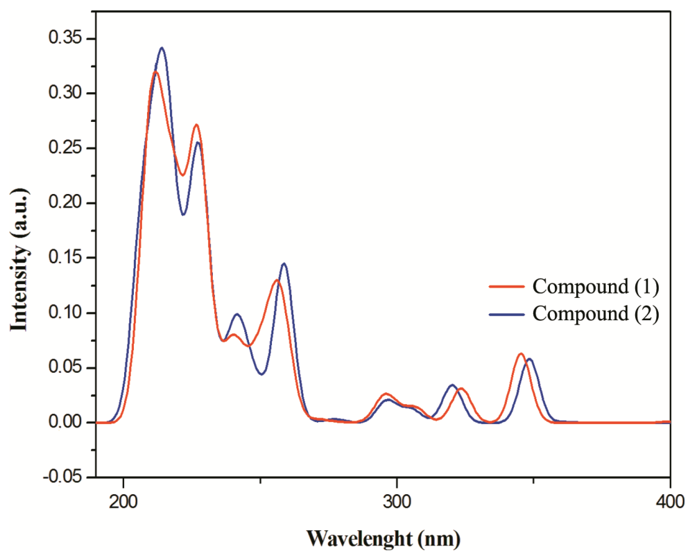
Fig. S4: Absorption spectra of the two compounds
