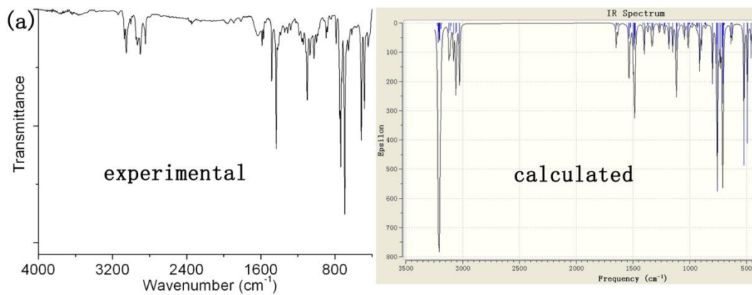
Figure S1 Experimental and calculated IR spectra of: (a) complex 1 , and (b) complex 2 .
