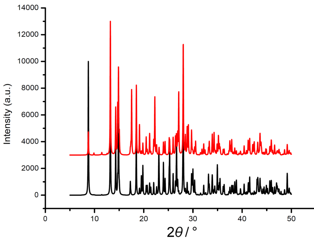
Figure S3 Experimental (red) and simulated (black) PXRD patterns of (I).
