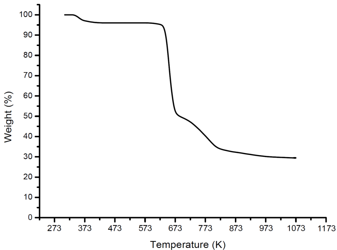
Figure S1 The TGA curve for (I).
