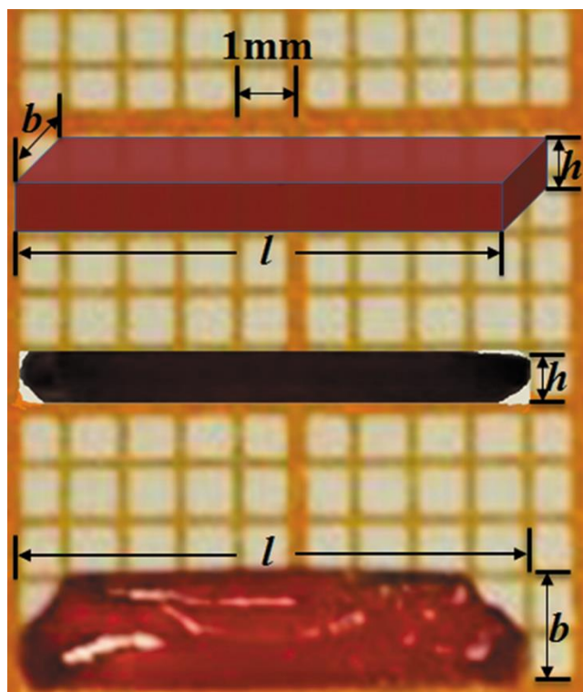
Figure S1 Size of the biggest single crystal of PDAK.
