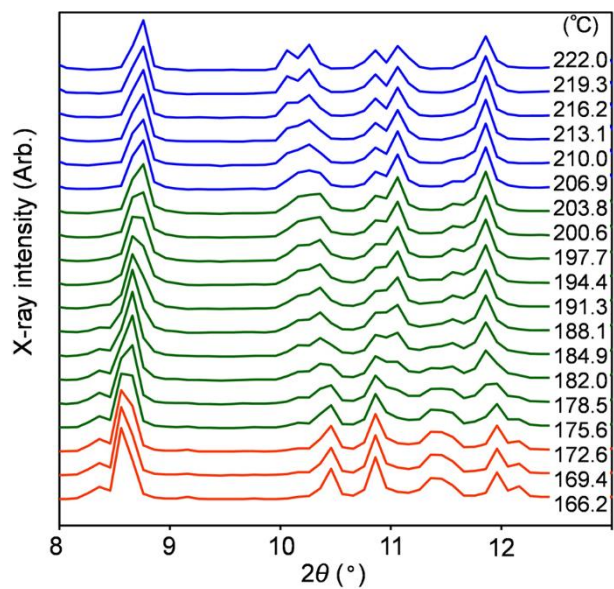
Fig. S1. Enlarged PXRD profiles of SN-38 monohydrate at a 2\theta value of around 10.1^\circ on heating.
