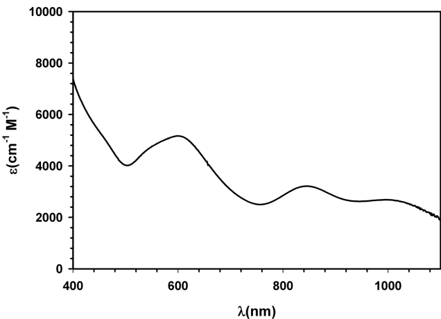
Figure S2. The UV-Vis-NIR spectrum of (I).
