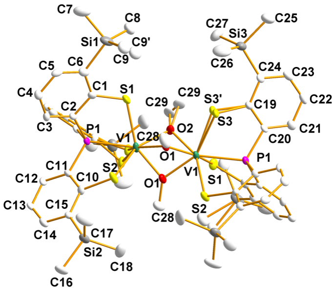
Fig. S1. A fully labelled plot of the anion of (I), shown with 35% probability displacement ellipsoids. The H atoms tetraphenylphosphonium cations and methanol solvent molecules have been omitted for clarity.
