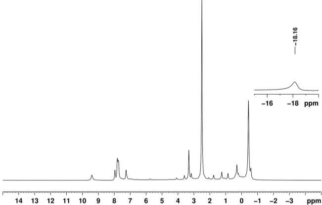
Figure S3. The ^1\text{H} NMR spectrum of (I).
