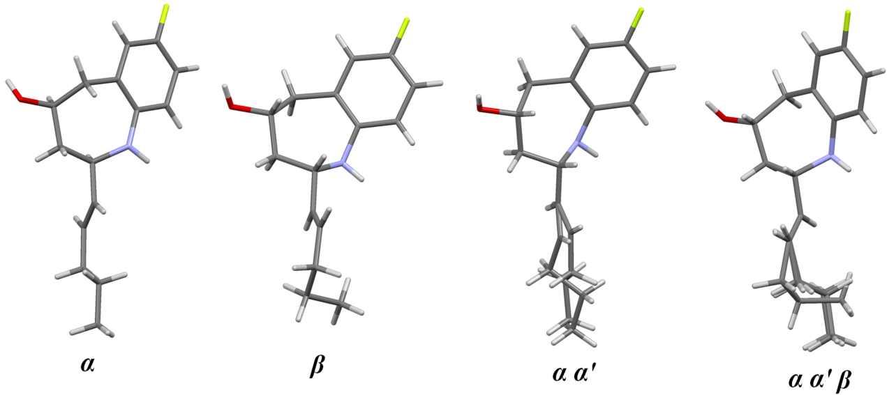
Fig. S1. The conformers of compound (5LT).
