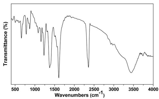
Figure S1 The IR spectrum of (I)
